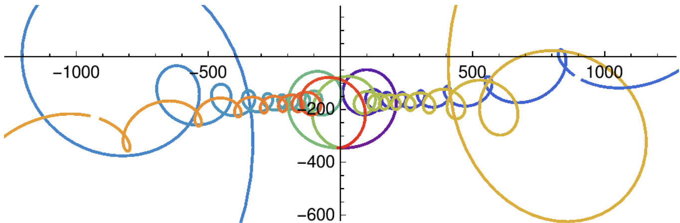
Figure 2: Zoom in of the parametric plot of the eigenvalues in Eq. (119) with coordinates \Re(t_n) and \Im(t_n) as a function of \theta . The lower bound of the summation is n = 0 and the upper bound of the summation is n = 10 (color online).
