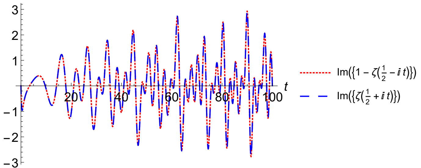
Figure 1: Plot of the imaginary components of Eq. (1). Results are compared with Eq. (115) (color online).
