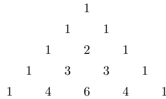
Figure 4. Pascal's triangle built up given n = 4 over k from 0 to n , sequence A007318 in OEIS, [9], [1], [13].
