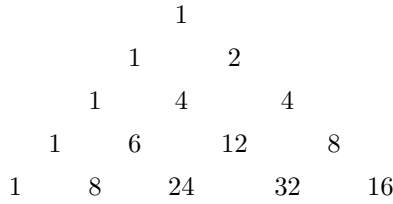
Figure 5. Triangle built by \binom{n}{k} \cdot 2^k, 0 \leq k \leq n .
