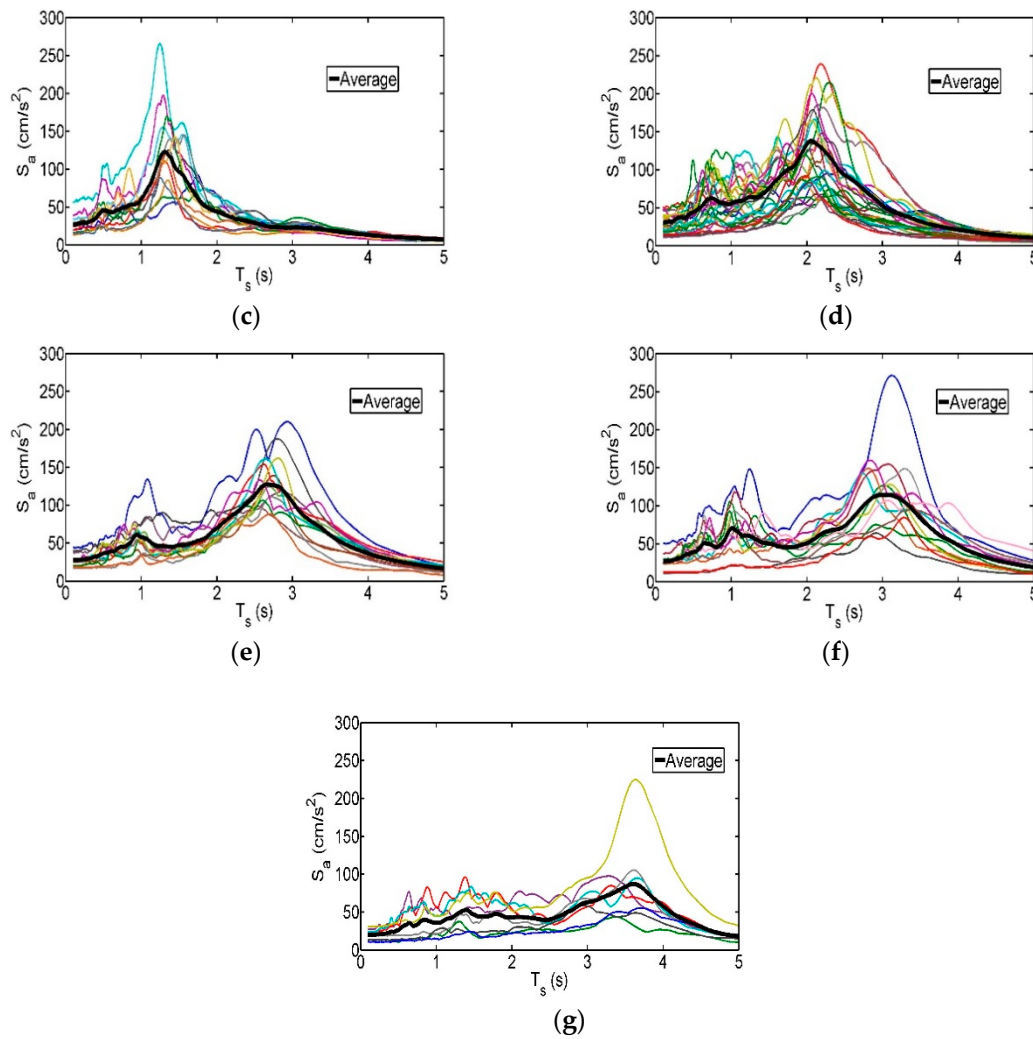
Figure 6. Pseudo-acceleration response spectra for 5% of critical damping, corresponding to the seismic records selected in (a) Zone A, (b) Zone B, (c) Zone C, (d) Zone D, (e) Zone E, (f) Zone F and (g) Zone G of the valley of Mexico considered in this study (E-W Component).
