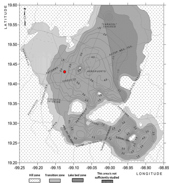
Figure 2. Curves of the dominant soil periods in the valley of Mexico.
