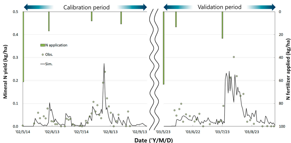
Figure 6. Daily QN predicted by APEX-Paddy is calibrated for the growing season in 2002 and then validated in 2003 at the Icheon site.
