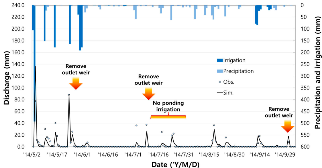
Figure 5. Simulated discharge amounts indicate that the timing and magnitude of peak discharges in response to outlet weir management are well predicted during the growing season in 2014 at the Gimje site.
