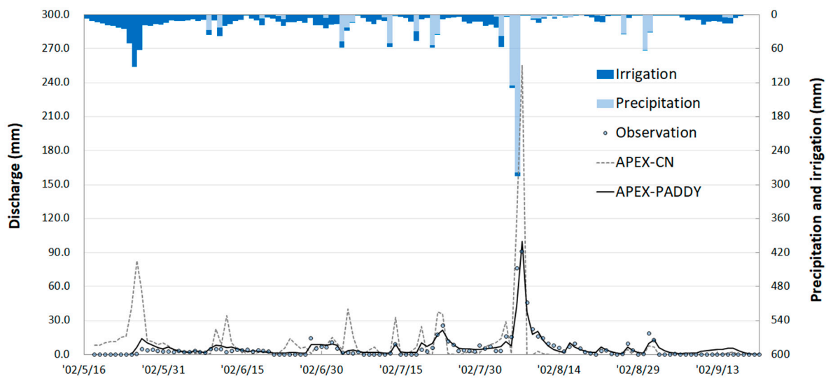
Figure 7. Predicted daily discharge hydrographs indicate that APEX-Paddy successfully simulates high peaks in daily discharge at the Icheon site by allowing surface retention of stormwater. The APEX model with the SCS-CN method over-predicted peak daily discharges up to 250% of the measured value.
