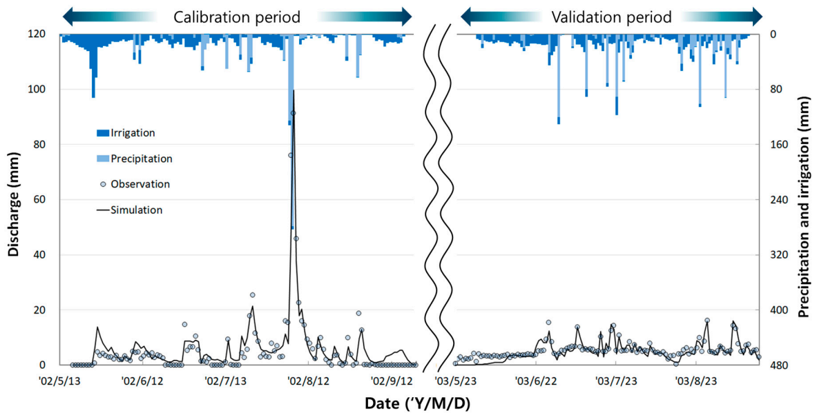
Figure 4. Predicted daily paddy field discharges are calibrated for the growing season in 2002, and then validated for the year 2003 at the Icheon site.
