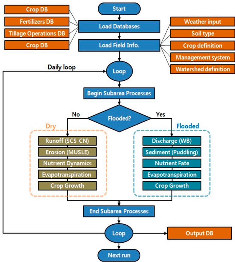
Figure 2. Schematic diagram of the APEX-Paddy algorithm.
