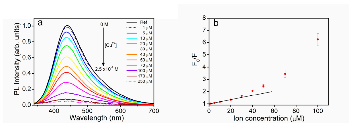
Fig. 2. (a) Emission spectra of the reference aqueous suspension of UFQDs in the presence of \text{Cu}^{2+} at different concentrations. (b) Stern-Volmer plot describes the fluorescence quenching intensity vs. the \text{Cu}^{2+} concentration over the range 0–100 \mu\text{M} .
