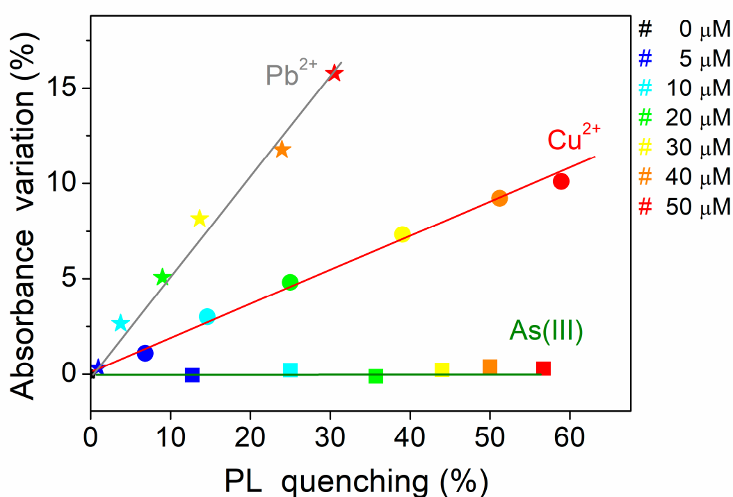
Fig. 6. The relative increase of the apparent absorption, measured at \lambda_a = 275 nm, plotted as a function of the relative quenching ratio (F_0 - F)/F_0 for each ion at different the concentrations according to the color scale on the right. The lines are guides for the eye.
