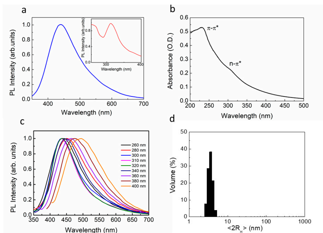
Fig. 1. (a) Fluorescence and excitation (inset) spectra of the UFQDs aqueous suspension. Excitation and emission wavelengths were 300 nm and 445 nm, respectively. (b) UV-vis absorption spectrum of the UFQDs aqueous suspensions. (c) Emission spectra excited at different wavelengths. (d) Particle size distribution of UFQDs, determined by using dynamic light scattering: \langle 2R_H \rangle 3.5 \pm 1.0 nm.
