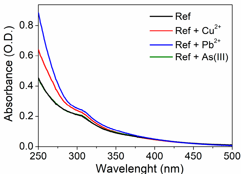
Fig. 4. The UV-vis spectrum of the UFQD reference solution in the presence of Cu 2+ , Pb 2+ and As(III) ions at a concentration of 100 \mu M.
