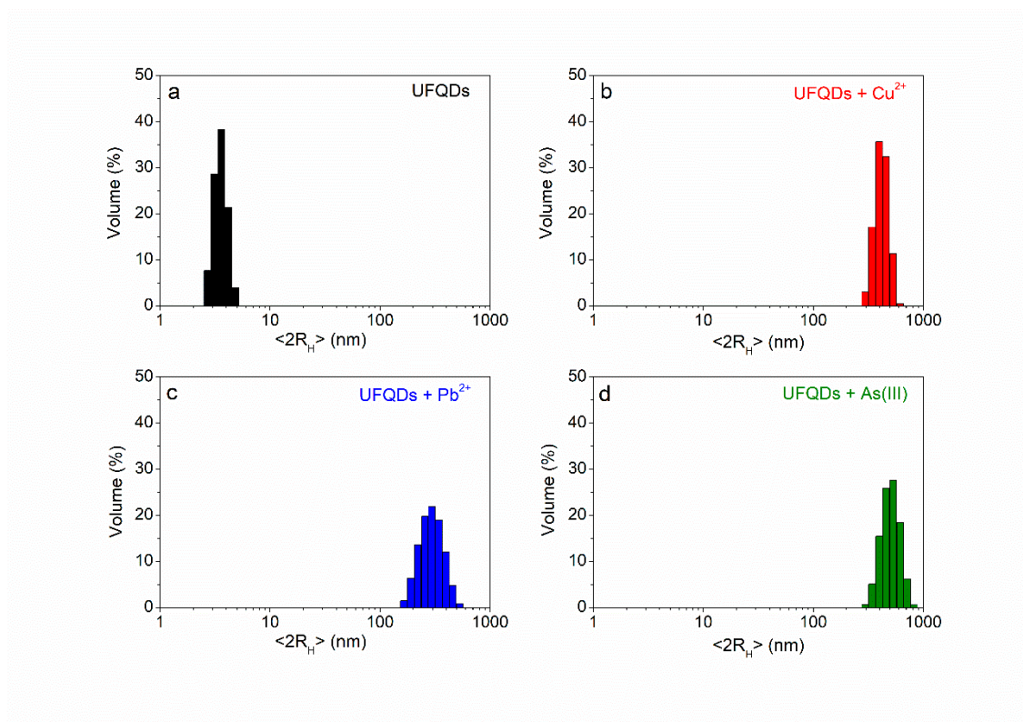
Fig. 5. Particle size distribution of UFQDs as determined by dynamic light scattering: (a) in the absence of any ion: \langle 2R_H \rangle = 3.5 \pm 1.0 nm; (b) in the presence of 100 \mu\text{M} of \text{Cu}^{2+} : \langle 2R_H \rangle = 420 \pm 25 nm; (c) in the presence of 100 \mu\text{M} of \text{Pb}^{2+} : \langle 2R_H \rangle = 300 \pm 22 nm; (d) in the presence of 100 \mu\text{M} of \text{As(III)} : \langle 2R_H \rangle = 510 \pm 35 nm.
