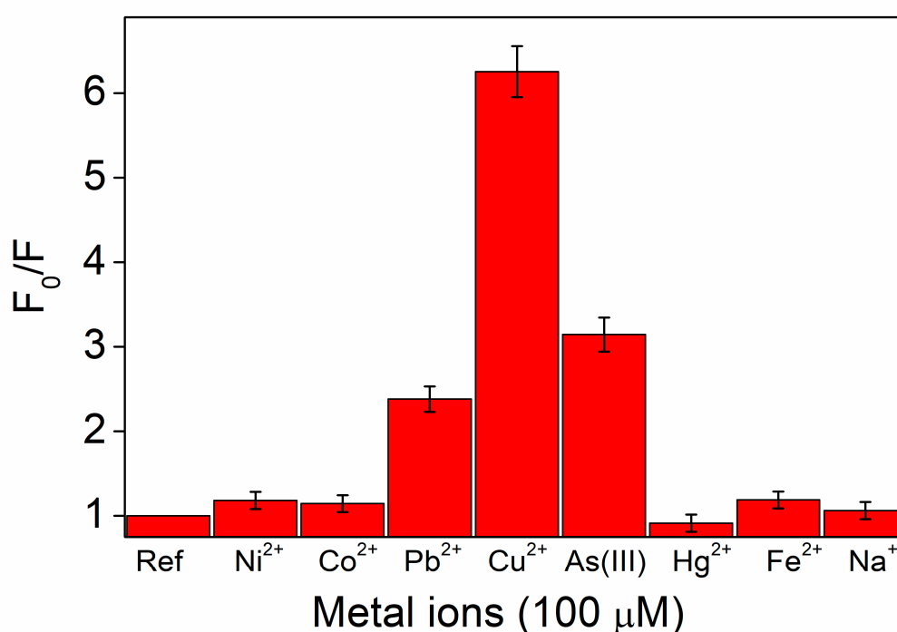
Fig. 3. Fluorescence intensity ratio F_0/F of the UFQD reference solution in the absence and presence of various individual metal ions at a concentration of 100 \mu\text{M} .
