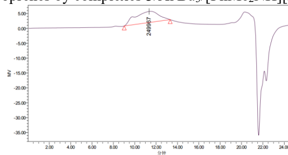
SFigure 20. GPC profiles of the polyisoprenes by complexes 3 /Al i Bu 3 /[PhMe 2 NH][B(C 6 F 5 ) 4 ] systems in Table 2, entry 10.
