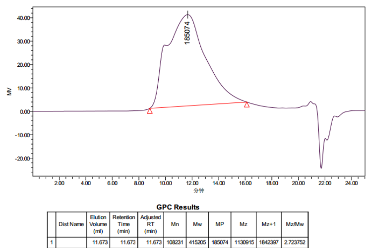
Figure 17. GPC profiles of the polyisoprenes by complexes 2 /Al i Bu 3 /[Ph 3 C][B(C 6 F 5 ) 4 ] systems in Table 2, entry 7.
