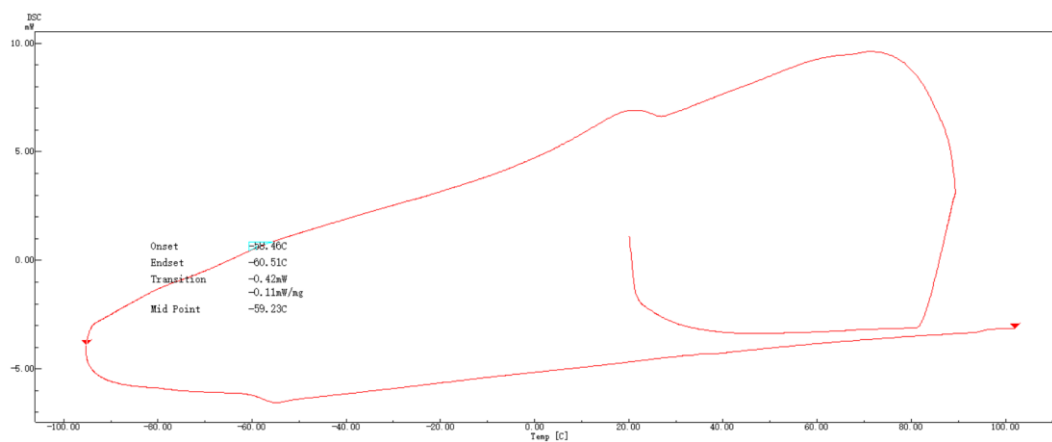
SFigure 27. DSC charts of the polyisoprenes by the 1 /AlEt 3 /[Ph 3 C][B(C 6 F 5 ) 4 ] systems in Table 2, entry 4.
