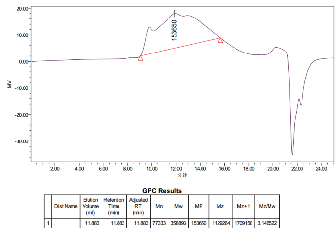
Figure 16. GPC profiles of the polyisoprenes by complexes 1 /AlMe 3 /[Ph 3 C][B(C 6 F 5 ) 4 ] systems in Table 2, entry 6.
