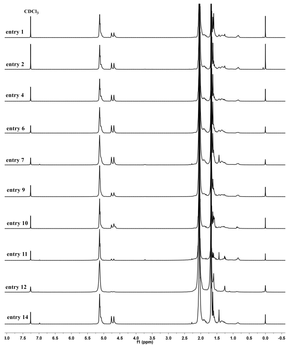
SFigure 10. ^1\text{H} NMR spectra of the polyisoprenes by complexes 1-3 / \text{AlR}_3 /Borate systems in Table 2.
