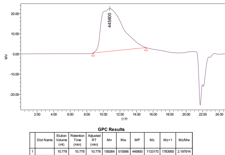
SFigure 14. GPC profiles of the polyisoprenes by complexes 1 /AlEt 3 /[Ph 3 C][B(C 6 F 5 ) 4 ] systems in Table 2, entry 4.
