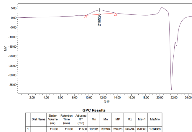
SFigure 19. GPC profiles of the polyisoprenes by complexes 3 / \text{Al}^i\text{Bu}_3 /[Ph 3 C][B(C 6 F 5 ) 4 ] systems in Table 2, entry 9.
