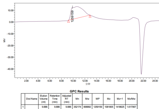
SFigure 22. GPC profiles of the polyisoprenes by complexes 3 /Al i Bu 3 /[Ph 3 C][B(C 6 F 5 ) 4 ] systems at -20 °C in Table 2, entry
