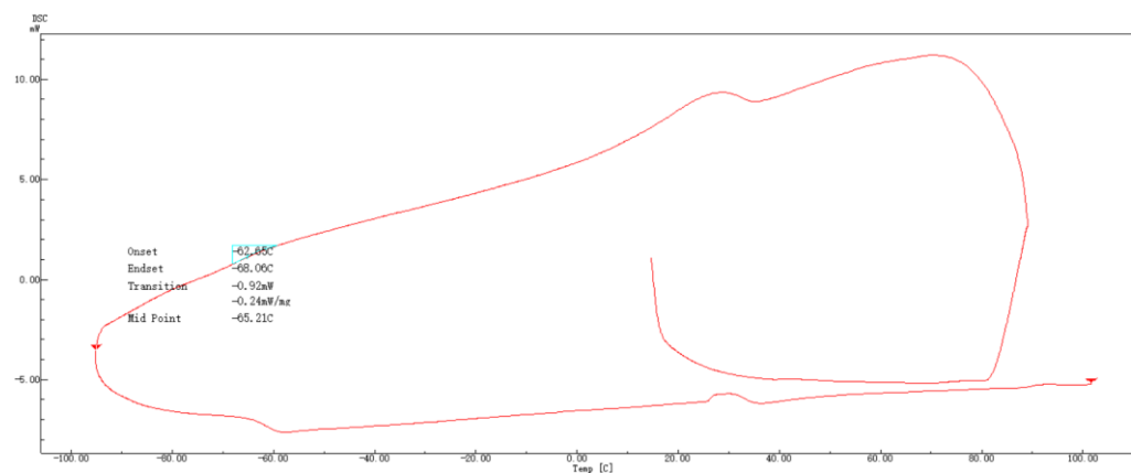
SFigure 30. DSC charts of the polyisoprenes by the 3 /Al i Bu 3 /[Ph 3 C][B(C 6 F 5 ) 4 ] systems at -20 °C in Table 2, entry 12.
