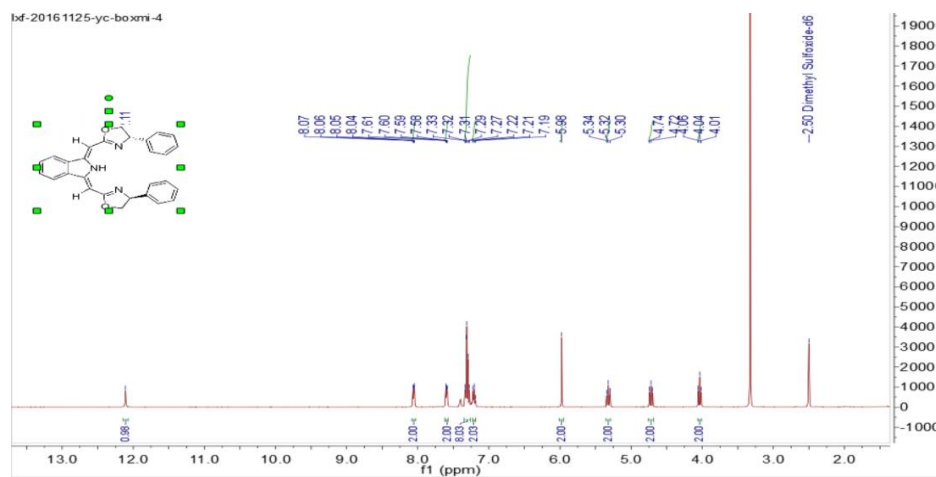
SFigure 3. 1 H NMR spectrum of ligand 4
