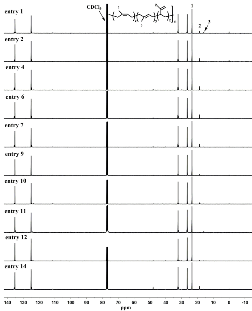
SFigure 11. ^{13}\text{C} NMR spectra of the polyisoprenes by complexes 1-3 / \text{AlR}_3 /Borate systems in Table 2.
