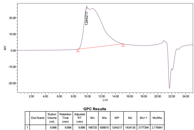
SFigure 24. GPC profiles of the polyisoprenes by complexes 3 /Al i Bu 3 /[Ph 3 C][B(C 6 F 5 ) 4 ] systems at 70 °C in Table 2, entry
