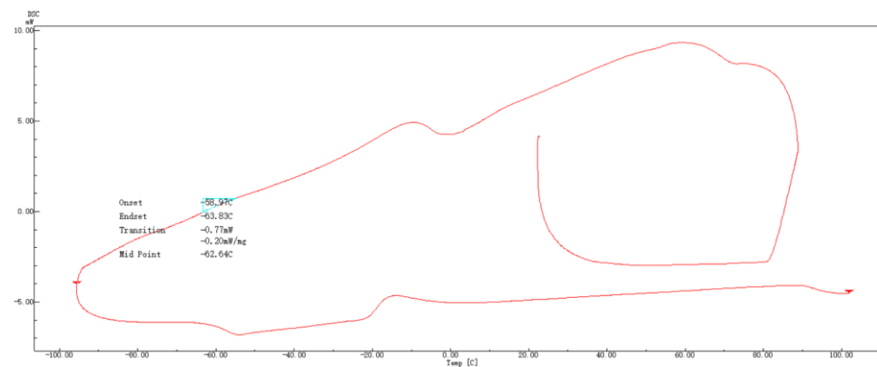
Figure 28. DSC charts of the polyisoprenes by the 1 /AlEt 3 /[PhMe 2 NH][B(C 6 F 5 ) 4 ] systems in Table 2, entry 5.
