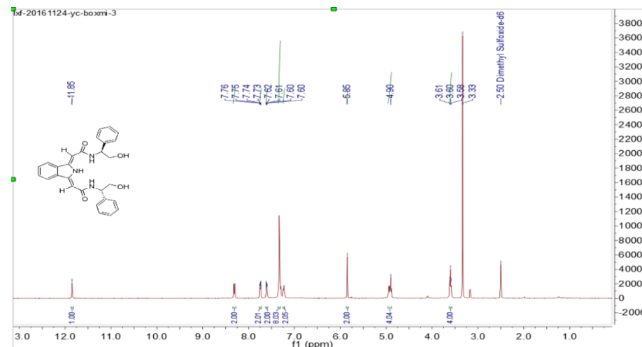
SFigure 2. 1 H NMR spectrum of ligand 5
