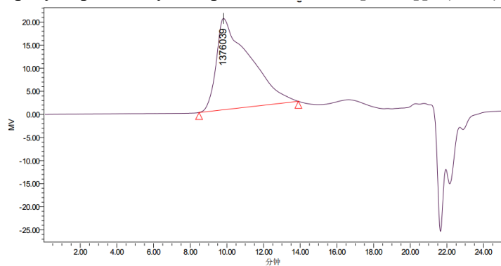
Figure 12. GPC profiles of the polyisoprenes by complexes 1/\text{Al}^i\text{Bu}_3/[\text{Ph}_3\text{C}][\text{B}(\text{C}_6\text{F}_5)_4] systems in Table 2, entry 1.
