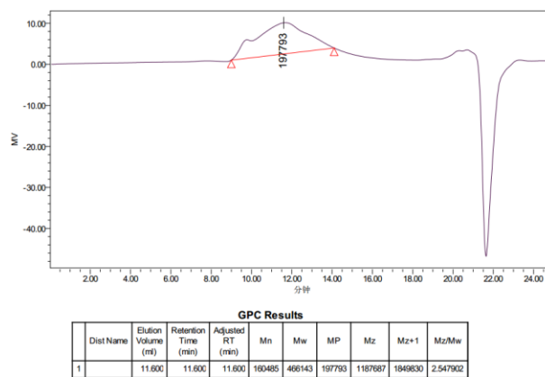
SFigure 23. GPC profiles of the polyisoprenes by complexes 3 /Al i Bu 3 /[Ph 3 C][B(C 6 F 5 ) 4 ] systems at 50 °C in Table 2, entry
