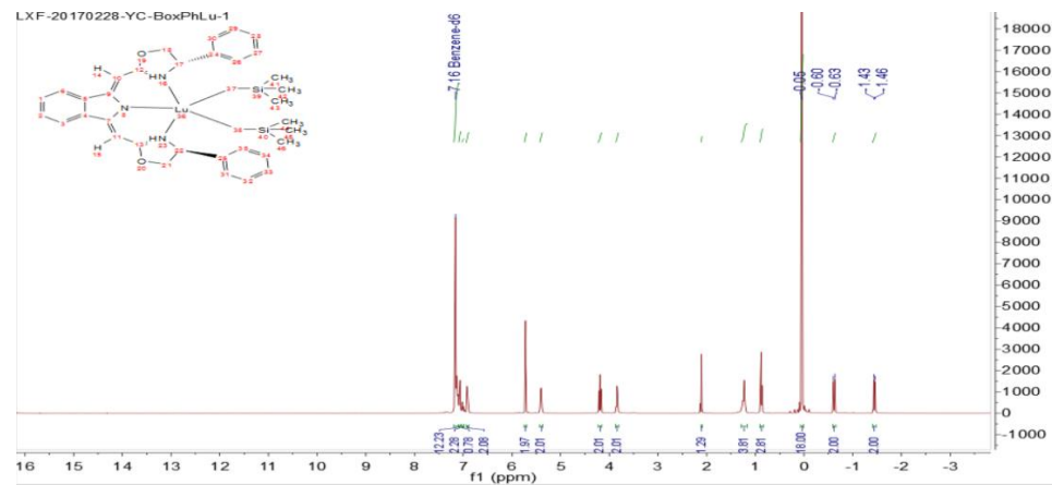
SFigure 6. ^1\text{H} NMR spectrum of complex 2
