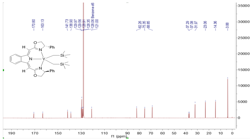
Figure 9. 13 C NMR spectrum of complex 3
