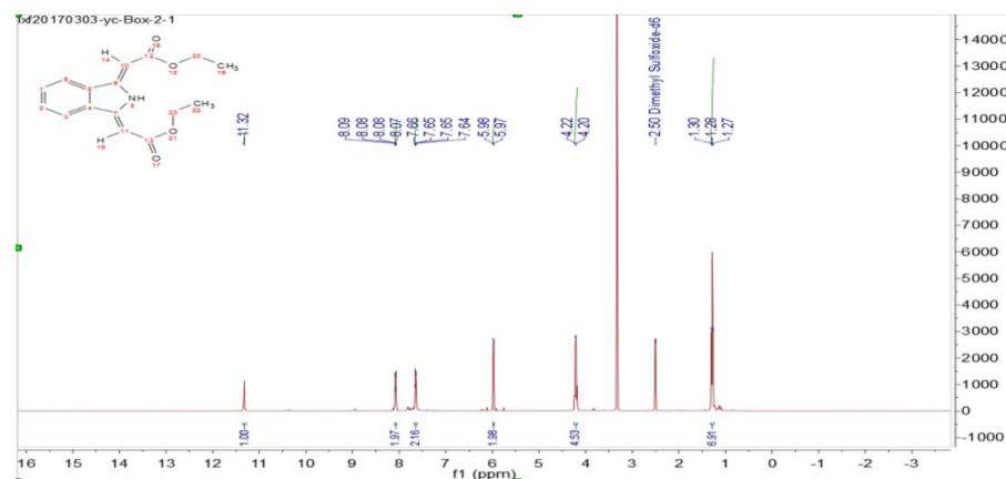
SFigure 1. 1 H NMR spectrum of ligand 6
