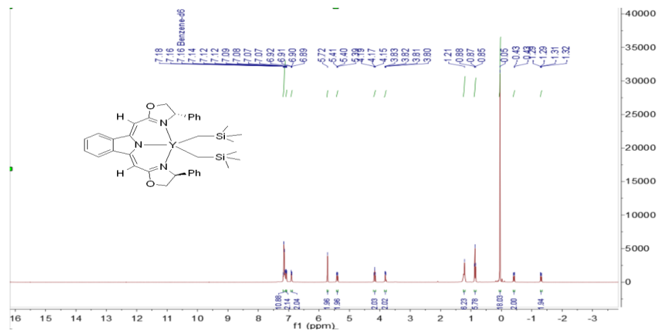
Figure 8. 1 H NMR spectrum of complex 3
