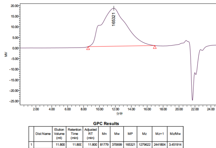
SFigure 18. GPC profiles of the polyisoprenes by complexes 2 / \text{Al}^i\text{Bu}_3 /[PhMe 2 NH][B(C 6 F 5 ) 4 ] systems in Table 2, entry 8.
