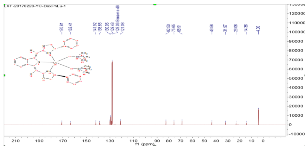
SFigure 7. ^{13}\text{C} NMR spectrum of complex 2
