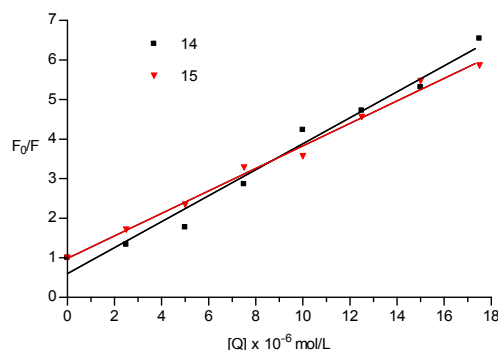
Figure 6: Stern–Volmer plots of BSA ( 1.00 \times 10^{-5} \text{ mol L}^{-1} ) quenched by CM14 and CM15 at 22 °C. The plots show a good linear relationship within the investigated concentrations of CM14 and CM15 .
