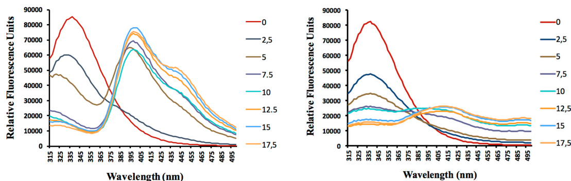
Figure 5: The effects of CM14 (left) and CM15 (right) on the fluorescence spectra of BSA at 22 °C. \text{ex} = 295 \text{ nm} ; c(\text{BSA}) = 1.00 \times 10^{-5} \text{ mol L}^{-1} ; c(\text{Q})/(\times 10^{-6} \text{ mol L}^{-1}) . Final concentrations of CM14 and CM15 = 0, 2.5, 5.0, 7.5, 10, 12.5, 15.0, and 17.5 \times 10^{-6} \text{ mol L}^{-1} , respectively.
