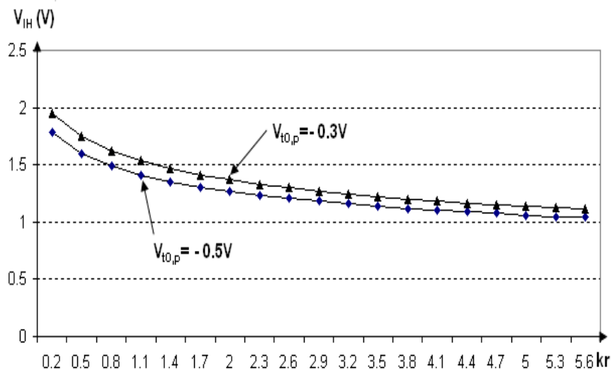
Figure 7. The dependence of voltage critical value V_{IH} on MOS transistors transconductance parameters ratio k_r for two parametric values of PMOS transistor threshold voltage, when NMOS transistor threshold voltage remains constant V_{t0,n} = 0.5V .
