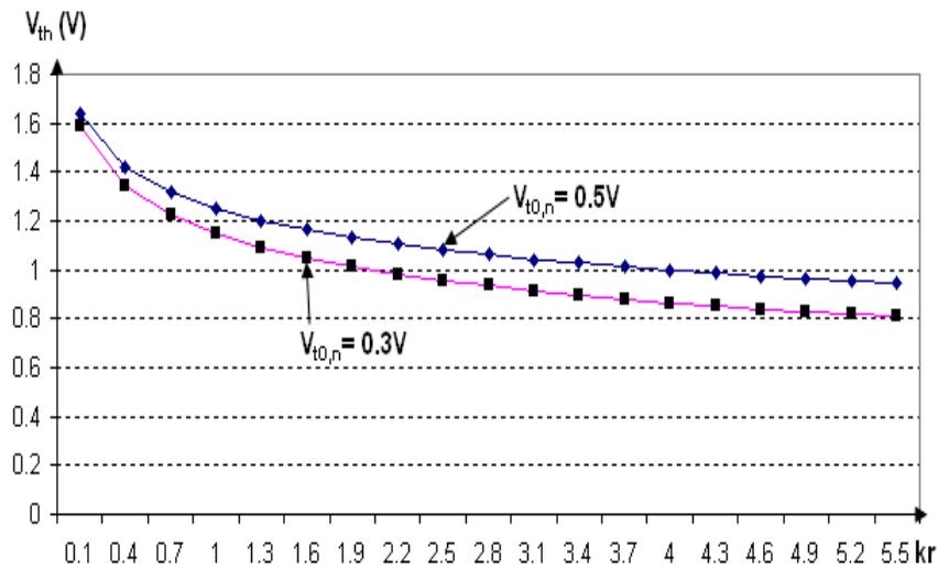
Figure 8. The impact of the transconductance parameters ratio ( kr ) of MOS transistors (NMOS and PMOS) on value of the CMOS inverter threshold voltage (on value of CMOS inverter switching threshold voltage) for two different values of the NMOS threshold voltage, when V_{t0,p} = -0.5 V and source voltage V_{DD} = 2.5 V.
