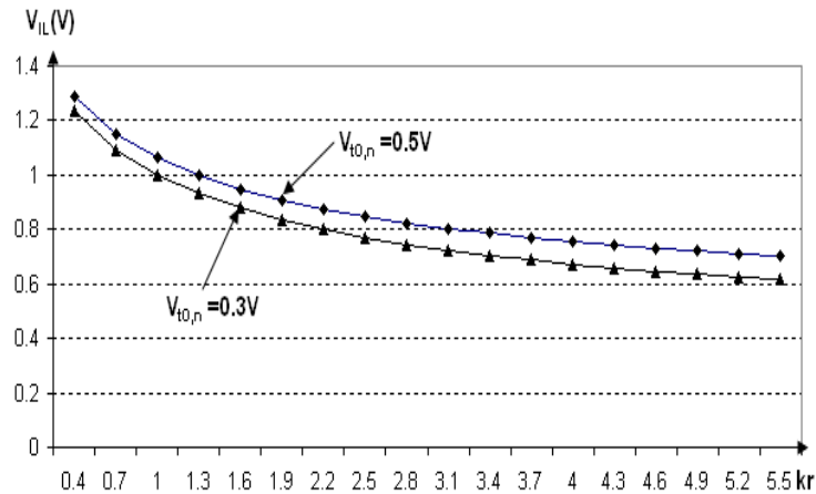
Figure 3. The dependence of input voltage critical value V_{IL} on ratio of MOS transistor transconductance parameters (the ratio of NMOS transconductance parameters on PMOS transconductance parameters) k_r for two different values of NMOS threshold voltage ( V_{t0,n} ), when threshold voltage of PMOS transistor has a constant value of V_{t0,p} = -0.5V .
