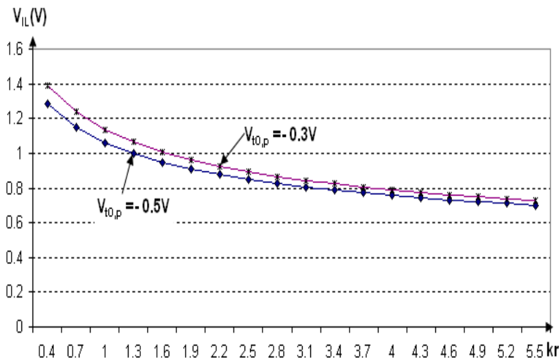
Figure 4. The dependence of input voltage critical value V_{IL} on the ratio of MOS transistor transconductance parameters k_r for two different values of PMOS threshold voltage ( V_{t0,p} ), when threshold voltage of NMOS transistor has constant value of V_{t0,n} = 0.5V .
