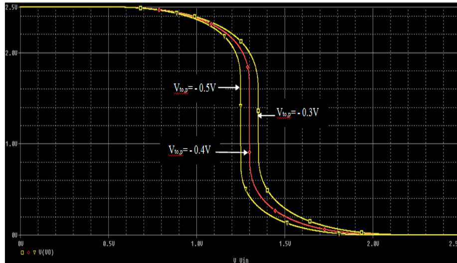
Figure 14. The impact of PMOS transistor threshold voltage ( V_{to,p} ) on CMOS inverter VTC shape, when NMOS transistor threshold voltage value is V_{to,n} = 0.5\text{ V} , and transistors have identical dimensions.
