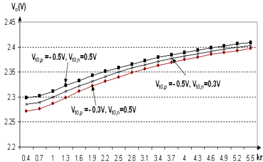
Figure 5. Influence of MOS transistor transconductance parameters ratio ( k_r ) on output voltage value V_o , when the input terminal of CMOS inverter is biased by voltage V_{in} = V_{IL} , for several parametric values of complementary MOS transistor threshold voltage.
