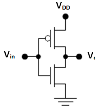
Figure 1. The structure of the CMOS inverter which contains two complementary enhancement-type MOS transistors.
