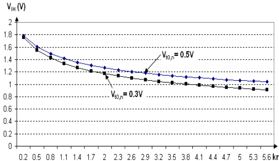
Figure 6. The dependence of the voltage critical value V_{IH} on MOS transistors transconductance parameters ratio k_r for two parametric values of NMOS transistor threshold voltage, when PMOS transistor threshold voltage remains constant V_{t0,p} = -0.5 V.
