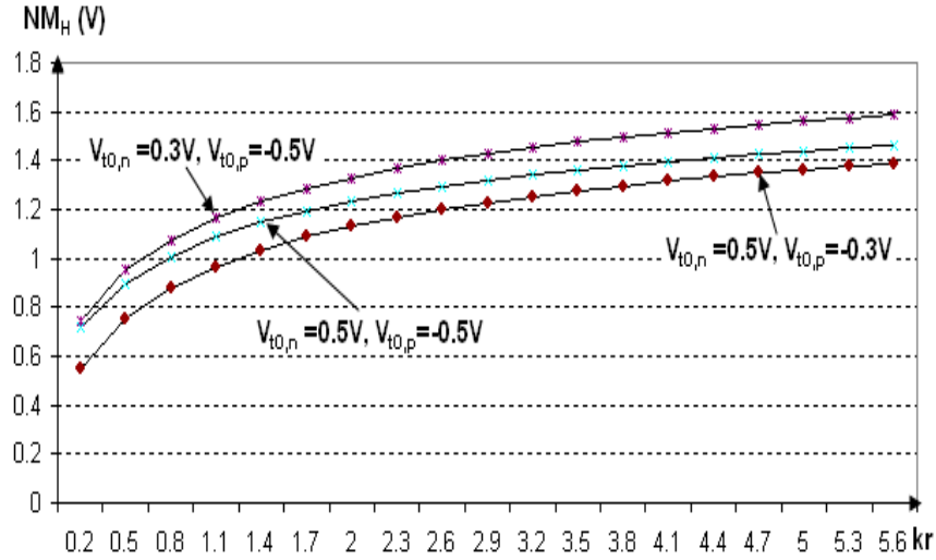
Figure 11. The dependence of the noise margins for high logic level NM_H on complementary MOS transistors transconductance parameters ratio k_r , for three cases of different MOS transistor threshold voltage (NMOS and PMOS transistors), when V_{DD} = 2.5 V.
