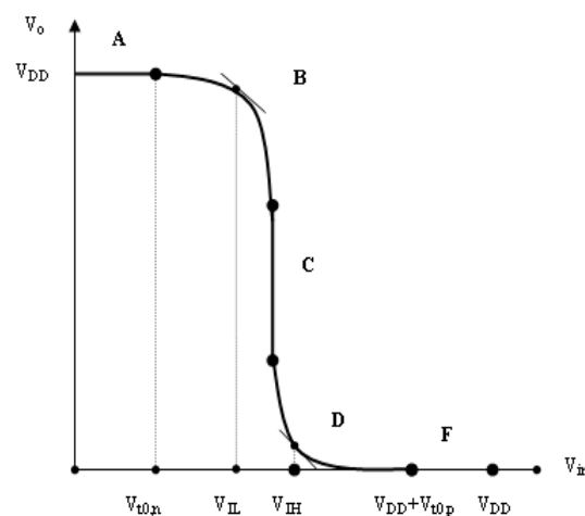
Figure 2. The typical VTC of the CMOS inverter.
