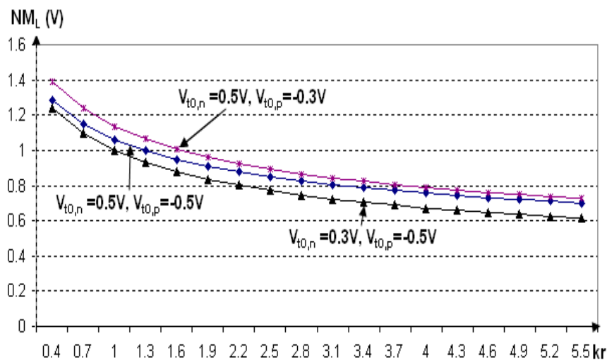
Figure 10. The dependence of the noise margins for low logic level NM_L on complementary MOS transistors transconductance parameters ratio k_r , for three cases of different MOS transistor threshold voltage (NMOS and PMOS transistors), when V_{DD} = 2.5 V.
