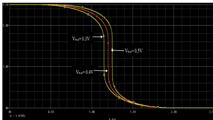
Figure 13. The impact of the NMOS transistor threshold voltage ( V_{t0,n} ) on VTC shape, when PMOS transistor threshold voltage is V_{t0,p} = -0.5 V, and transistors have identical dimensions.
