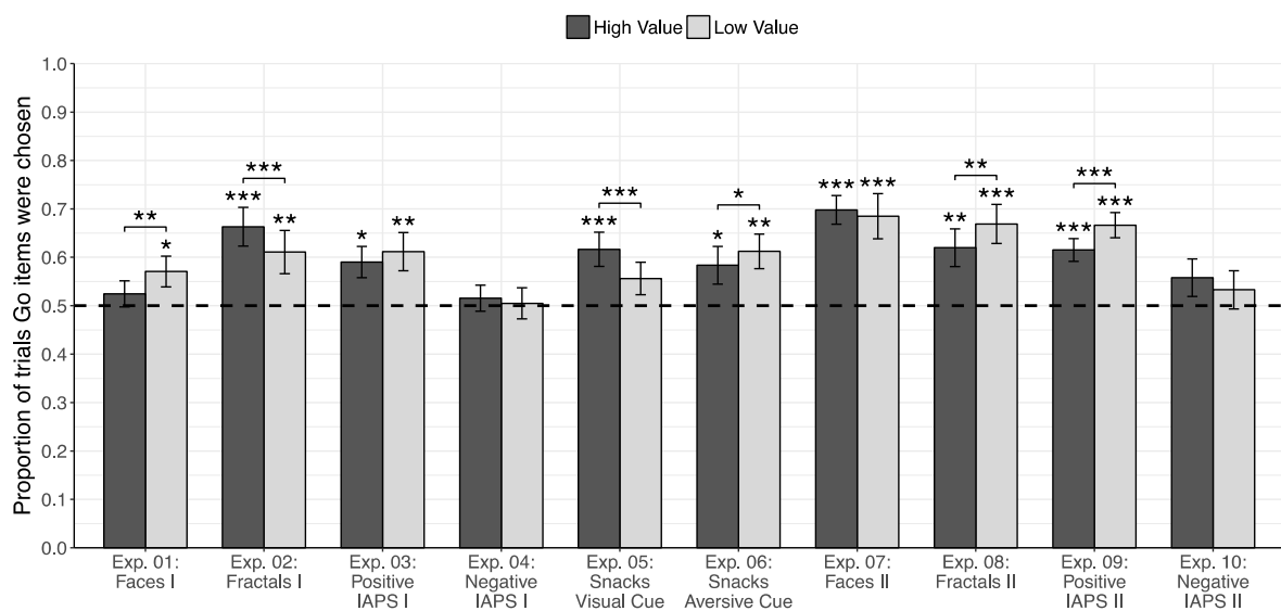
Figure 3. Probe results of Experiments 1-10.
