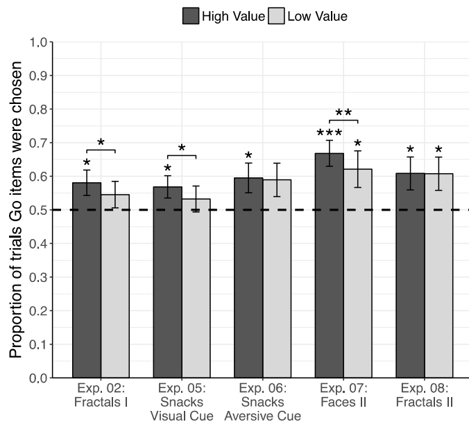
Figure 4. Probe results of follow up sessions.
