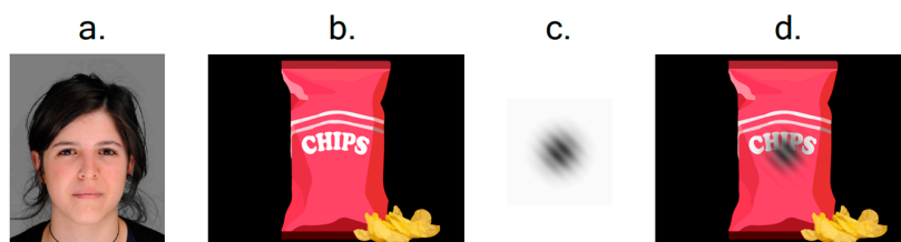
Figure 1. Stimuli and cue examples. 1a. Example of a face stimulus with neutral expression used in Experiment 7. 1b. Illustration of snack-food stimulus similar to the ones used in Experiments 5-6. 1c. Semi-transparent Gabor used as a visual cue in Experiments 6 and 9-10. 1d. Example of snack-food stimulus with the visual cue overlaid on it.
