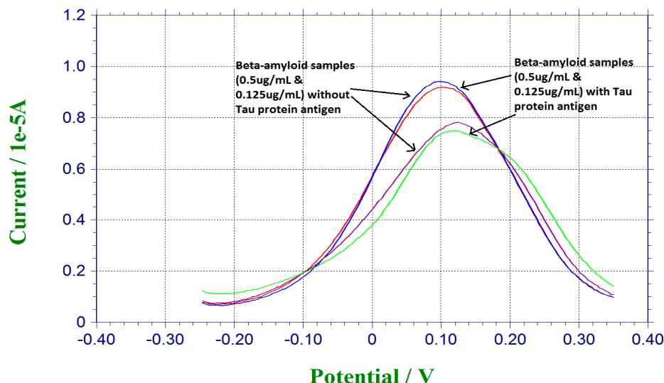
Figure4. Interference study based on Tau protein antigen.
