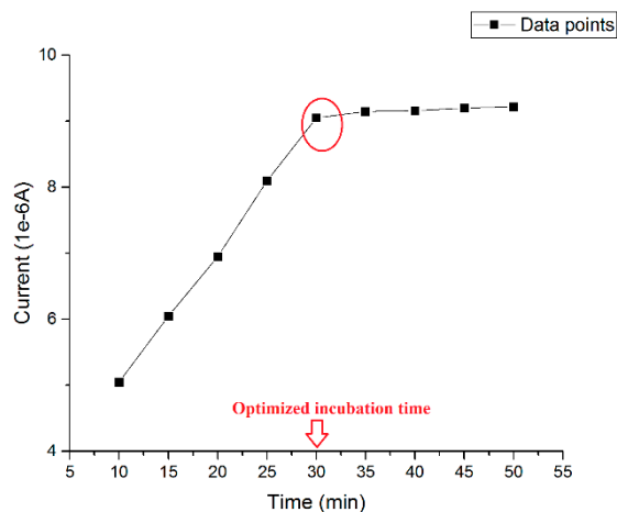
Figure1. Optimized incubation time of \beta -amyloid 42
