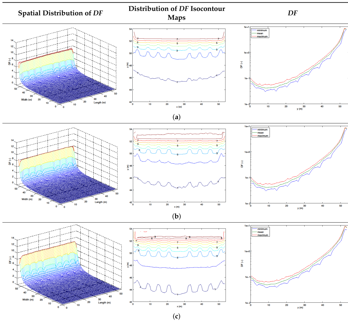
Figure 13. Spatial distribution of daylight factor (DF), distribution of DF isocontour maps, and decrease of illuminance at different windows heights of: (a) 1800 mm; (b) 2100 mm; and (c) 2400 mm using Radiance simulation program.
