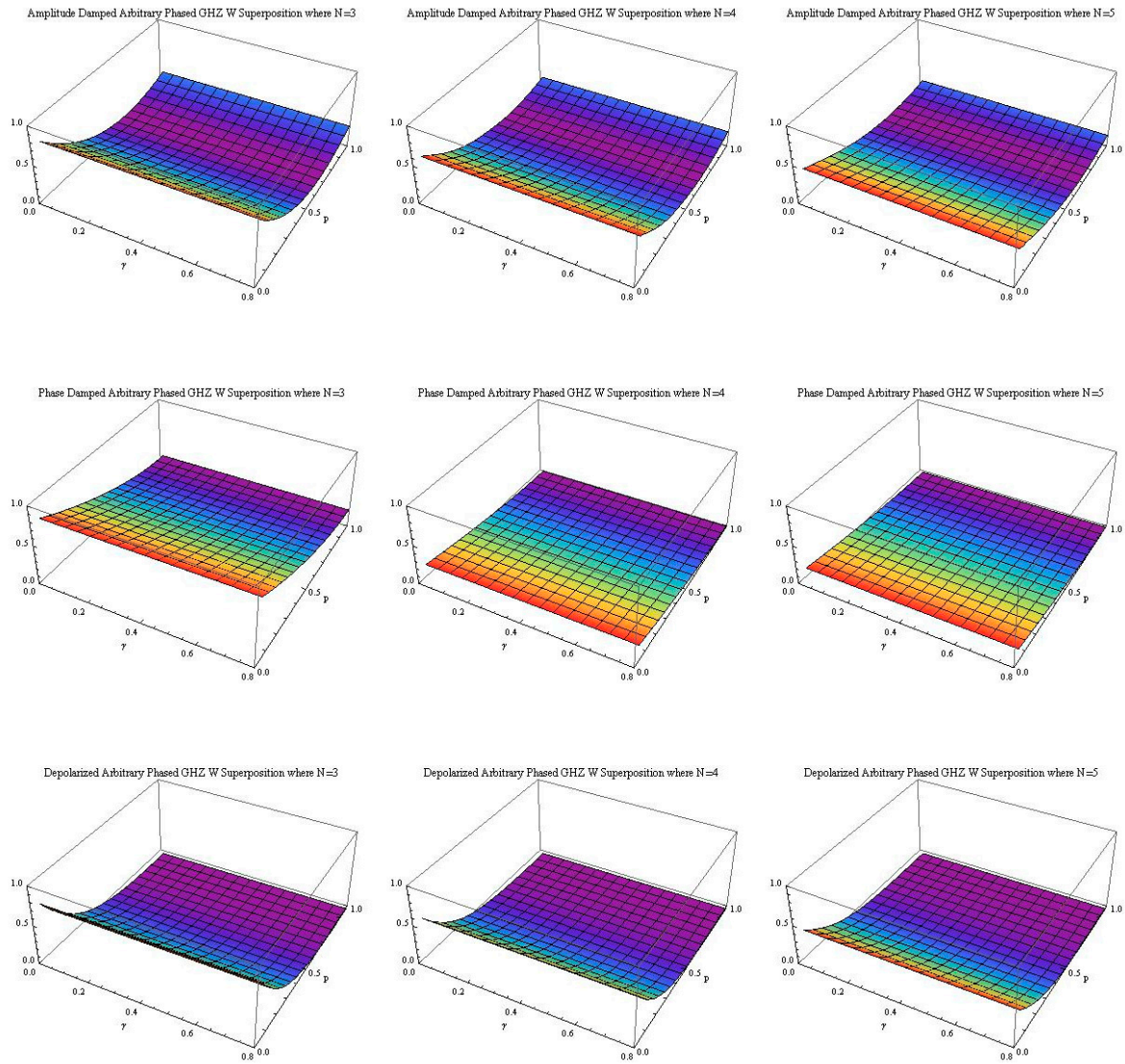
Fig. 4. QFI values as function of \gamma and p (3D plot)
