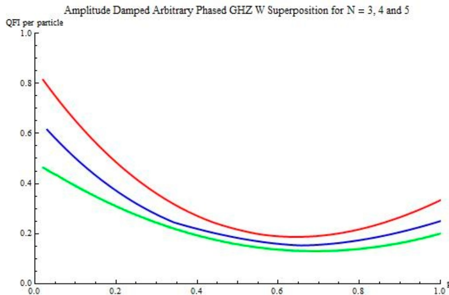
Fig. 1. Changes in QFI per particle for ADC with changing p values (Red: N=3 , Blue: N=4 , Green: N=5 )
