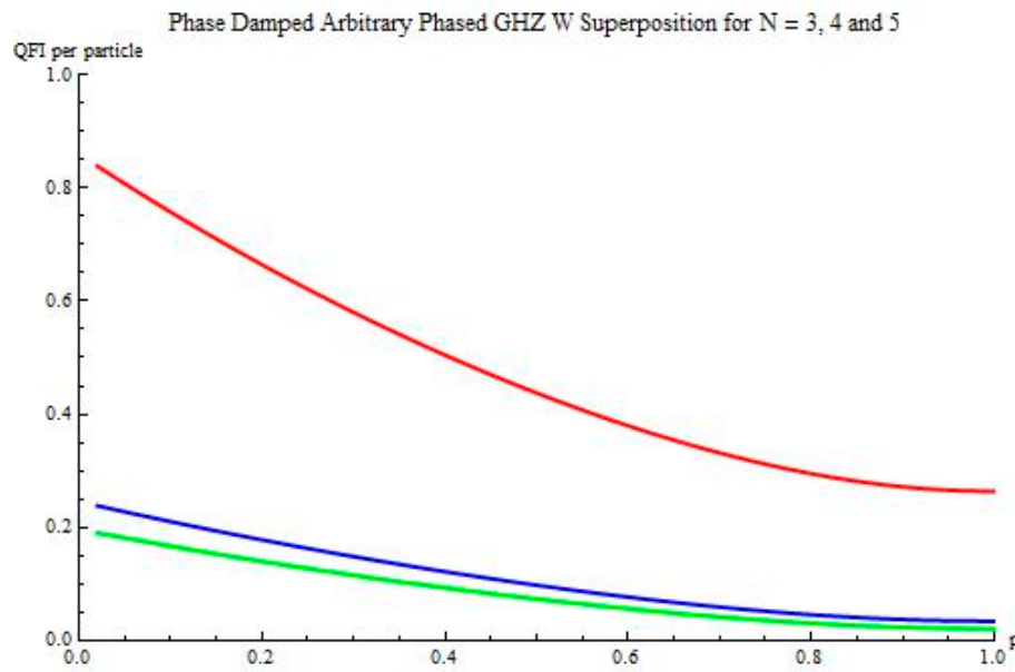
Fig. 2. Changes in QFI per particle for PDC with changing p values (Red: N=3 , Blue: N=4 , Green: N=5 )
