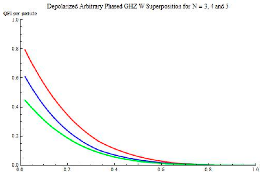
Fig. 3. Changes in QFI per particle for DPC with changing p values (Red: N=3 , Blue: N=4 , Green: N=5 )
