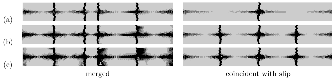
Figure 7: Mesh sensitivity study: Contour plot of maximum principal strain for the fine meshes for merged and coincident with slip approaches in the x - z section at y = 0.05 m at three stages marked in Figures 4 and 5. Black and light grey correspond to large and small maximum principal strains, respectively.
