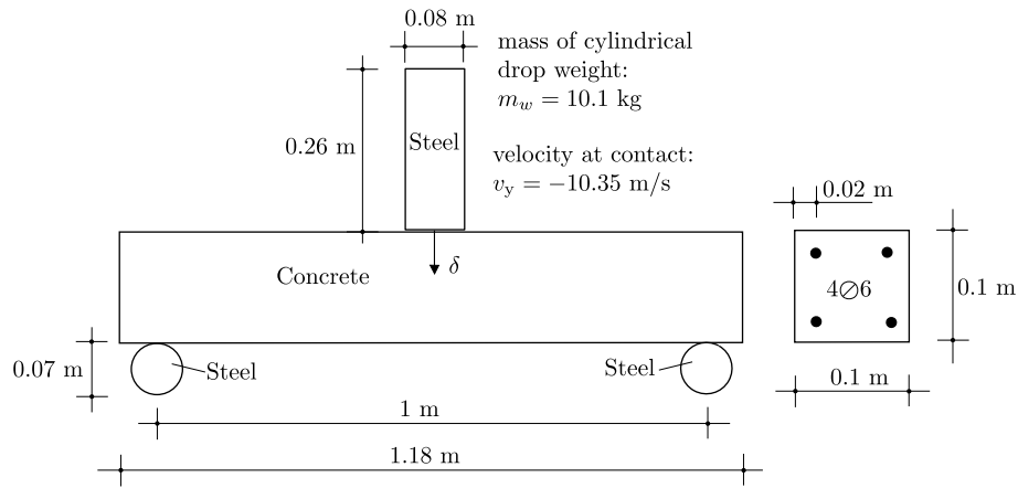
Figure 12: Drop weight impact test: Geometry and loading setup of a drop weight impact test for a reinforced concrete beam in [26, 24].
