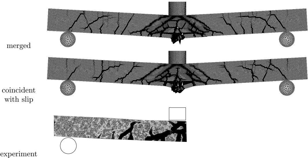
Figure 15: Drop weight impact test: Contour plot of maximum principal strain for merged and coincident with slip approaches compared to DIC results from experiments reported in [26, 24] at 9.5 ms. For the finite element analyses, black and light grey correspond to large and small maximum principal strains, respectively. For the experimental DIC results, black refers to large crack opening.
