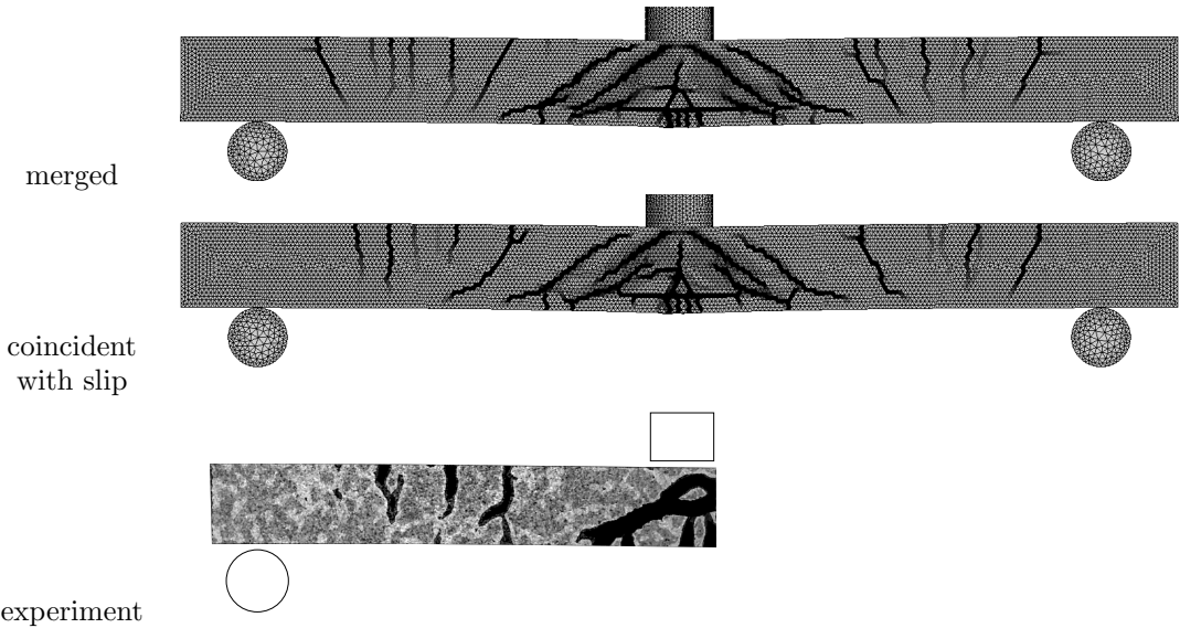
Figure 14: Drop weight impact test: Contour plot of maximum principal strain for merged and coincident with slip approaches compared to DIC results from experiments reported in [26, 24] at 0.8 ms. For the finite element analyses, black and light grey correspond to large and small maximum principal strains, respectively. For the experimental DIC results, black refers to large crack opening.
