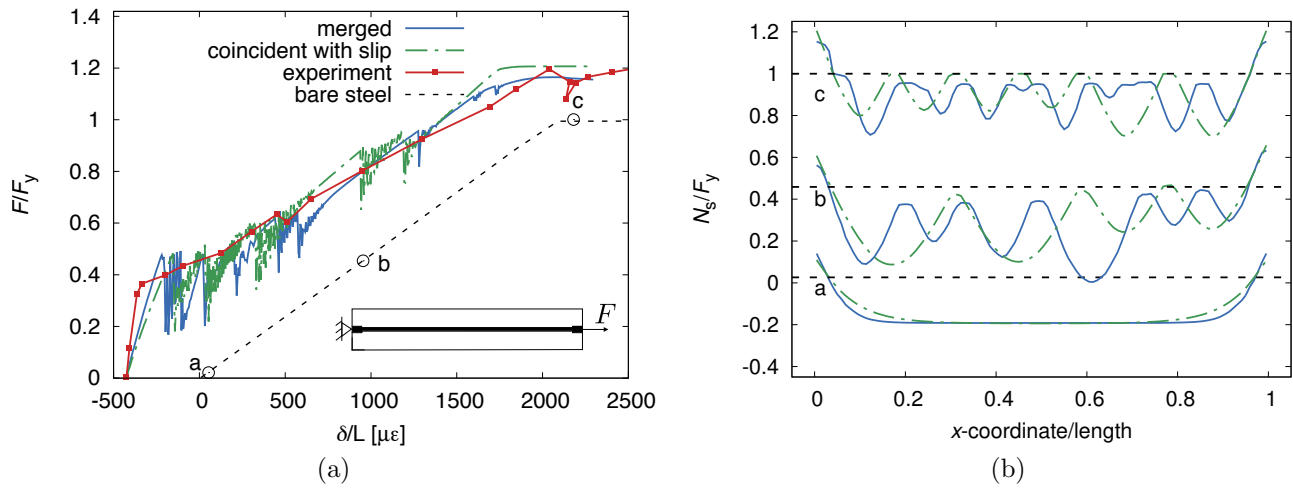
Figure 10: Tension stiffening experiment for fibre reinforced concrete: Comparison of finite element results with merged and coincident with slip approach compared to experiments reported in [5] in the form of (a) load versus average strain and (b) normalised axial stress in the reinforcement.
