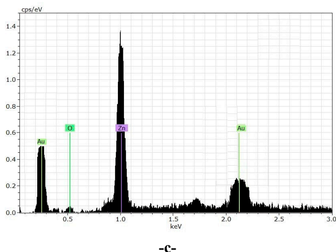
Figure (7) EDX analysis of ZnO thin films prepared by PLA method on glass substrate with energy of a-600 ,b-700, and c-800 mj in methanol solvent.
