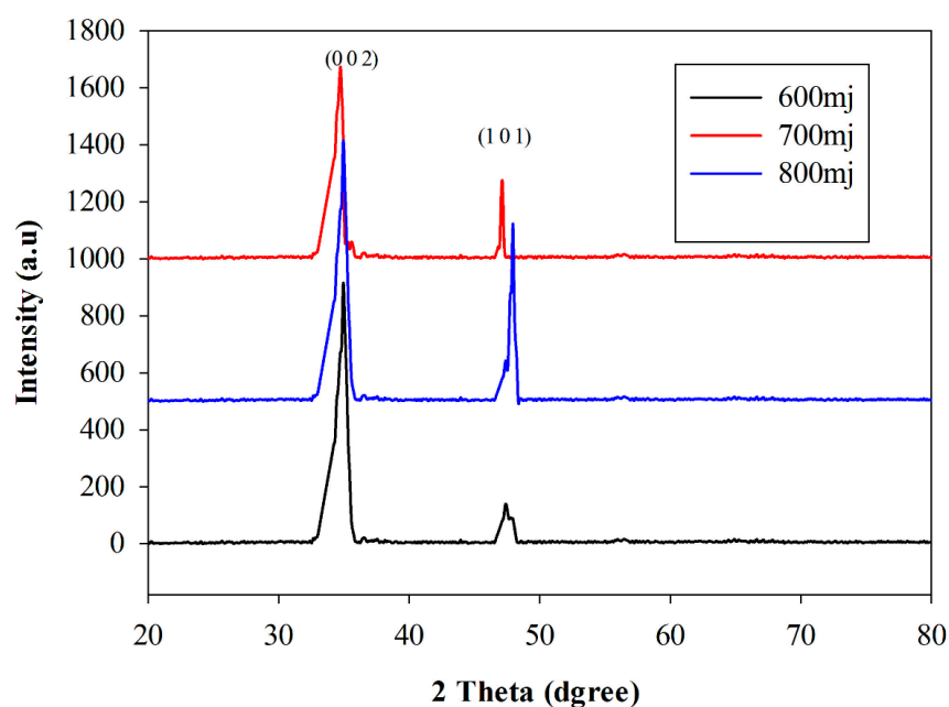
Figure (3): XRD pattern of ZnO nanoparticle on glass substrate with laser pulses number of 1500 pulse at energy 600 mJ, 700 mJ and 800 mJ.
