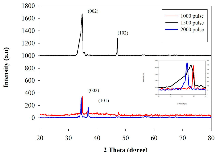
Figure (2): XRD pattern of ZnO nanoparticle on glass substrate with laser pulses number of 1000, 1500, and 2000 pulse at energy 700 mJ methanol solvent
