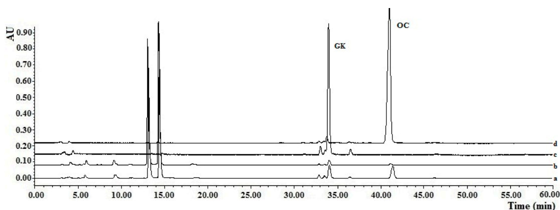
Figure 4. Chromatograms for MISPE using the gradient elution method: (a) Chromatograms of the fruit extracts solutions; (b) Chromatogram of elution fractions from the OC-MISPE column after gradient elution (Methanol-water, 35:65, v/v); (c) Chromatogram of elution fractions from the OC-MISPE column after gradient elution (Methanol-water, 50:50, v/v); (d) Chromatogram of elution fractions from OC-MISPE column after gradient elution (Methanol-water, 70:30, v/v).
