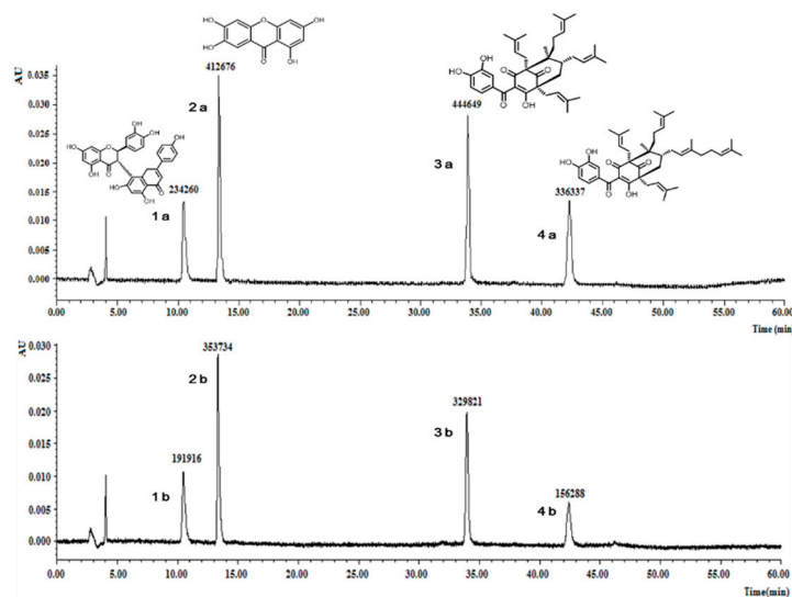
Figure 3. Chromatograms for the selectivity experiment. The peak areas of volkensiflavone (1a and 1b), 1, 3, 6, 7-tetrahydroxyxanthone (2a and 2b), GK (3a and 3b) and OC (4a and 4b) before and after incubation with 10 mg of MIPs C were showed.
