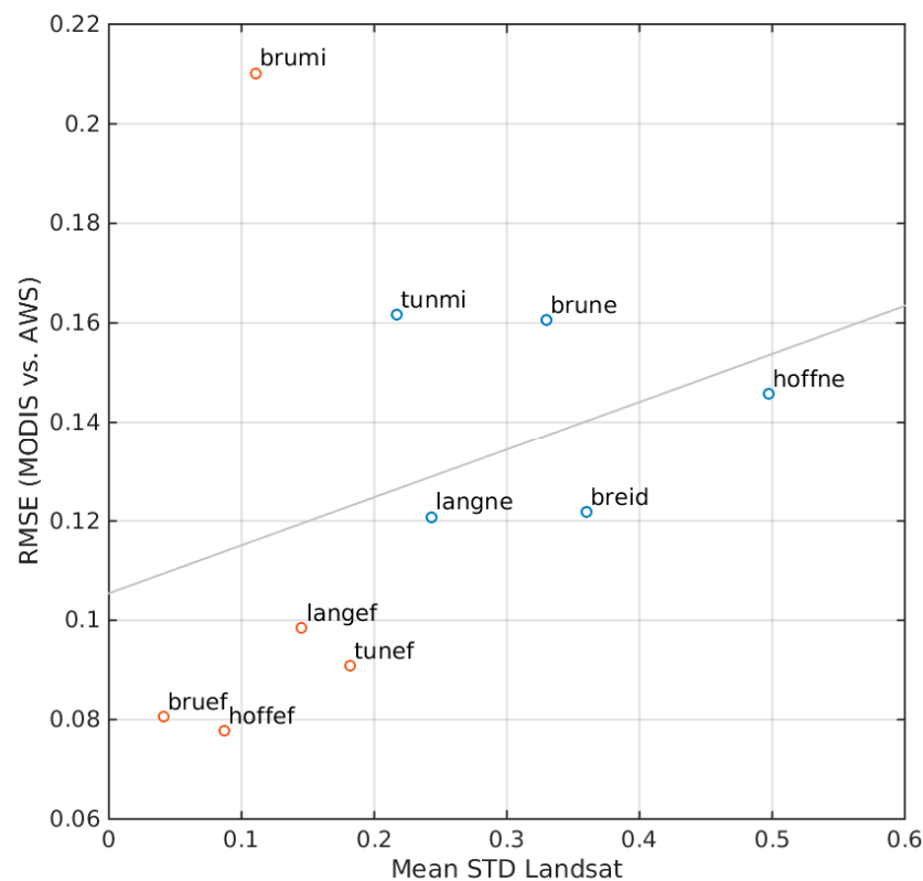
Figure 7. Scatter plot of the RMSE obtained by the comparison of the MODIS albedo with the in situ data (Sect. 3.1) versus the mean of the standard deviations of the Landsat albedo that were sampled within the extent of a MODIS pixel. The mean STD was obtained by averaging the standard deviations computed for every combination of Landsat and AWS in Table 2. The color of the circles indicates if the AWS are in the accumulation area (red) or in the ablation area (blue).
