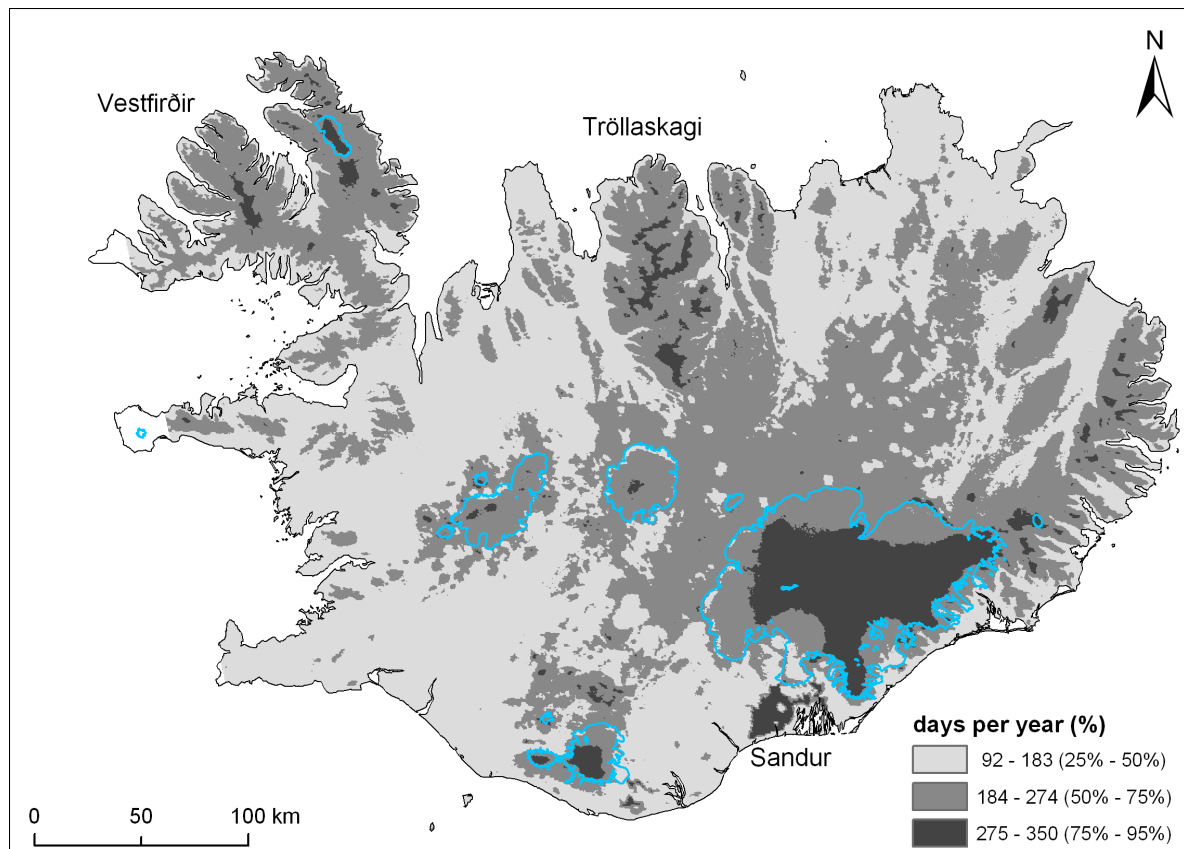
Figure 3. Mean annual number of days with missing data during the period 2001-2012 in the MCD43A3 product.
