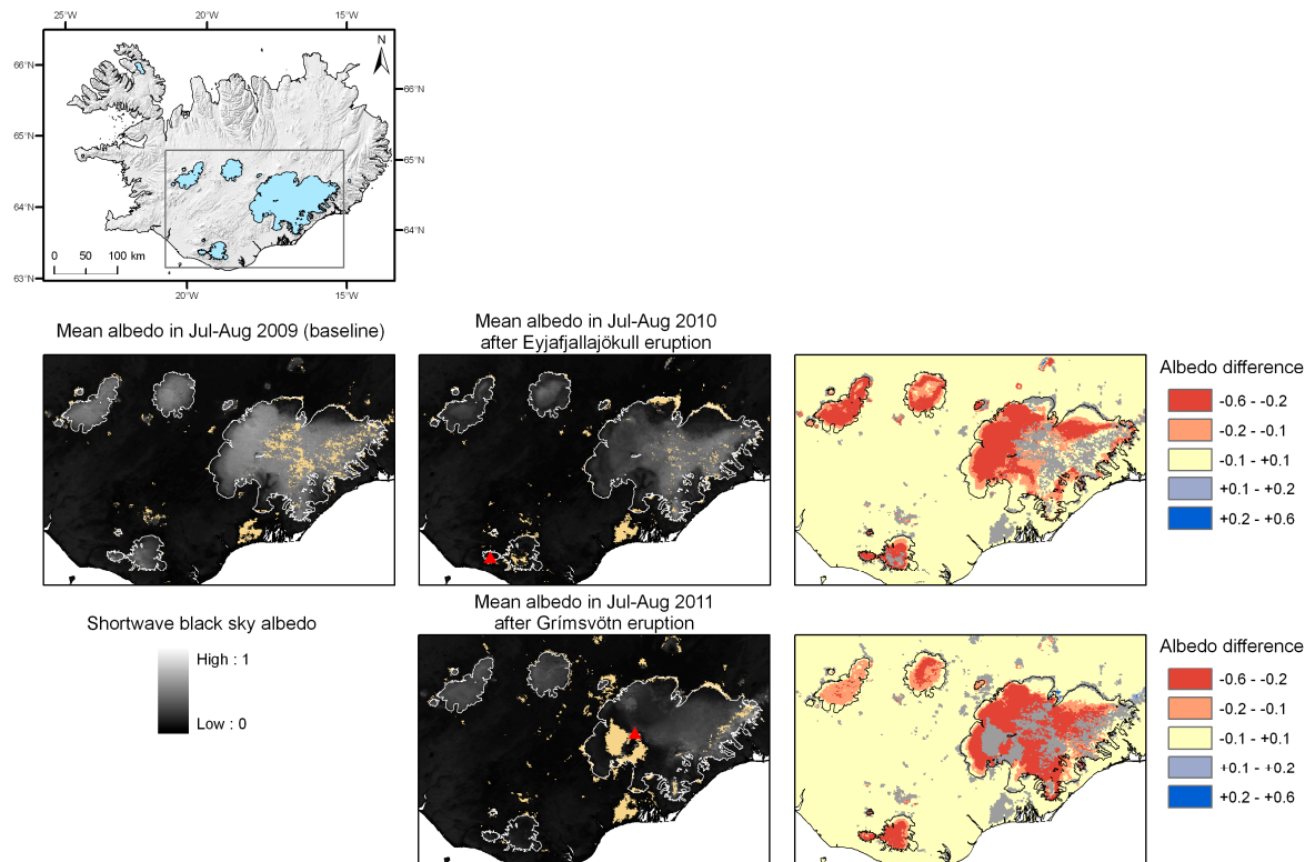
Figure 9. Albedo of the main ice caps before and after the Eyjafjallajökull and Grímsvötn eruptions, and associated albedo changes. The volcanoes that erupted in May 2010 and 2011 are marked with red triangles in the middle figures. Here we excluded Drangajökull, which was not significantly affected by the eruptions (Table 4, Figure 9).
