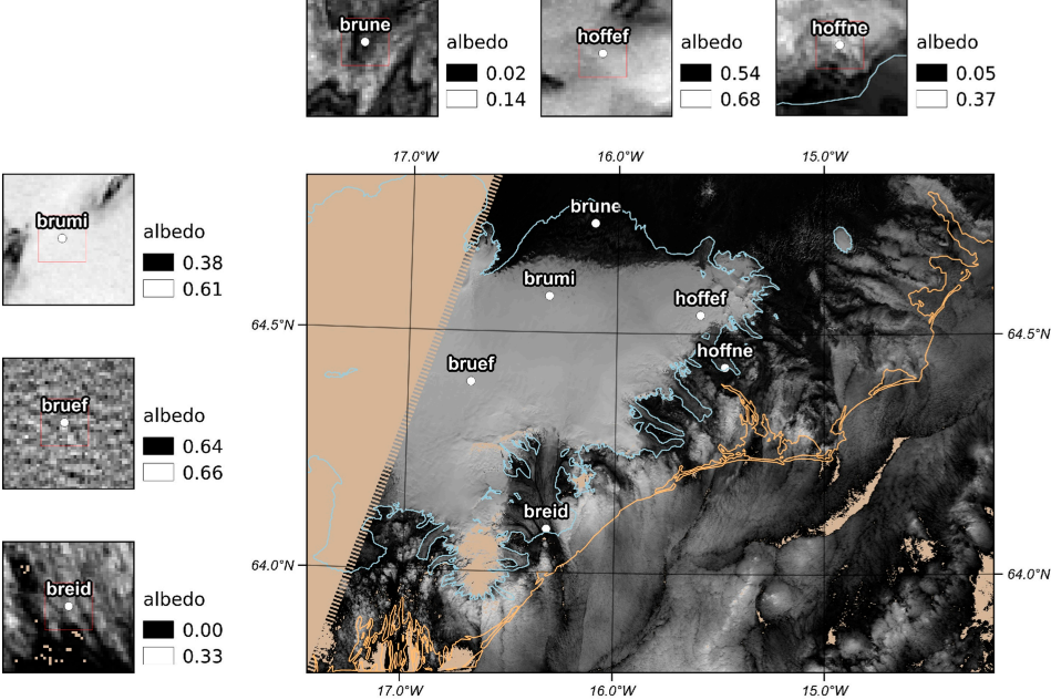
Figure 6. An example of subpixel variability at each AWS site. Three summer Landsat scenes were used to compute albedo maps at 30 m resolution. A red square polygon corresponding to a MODIS pixel is drawn in each subset. Beside each subset is indicated the upper and lower values of the
