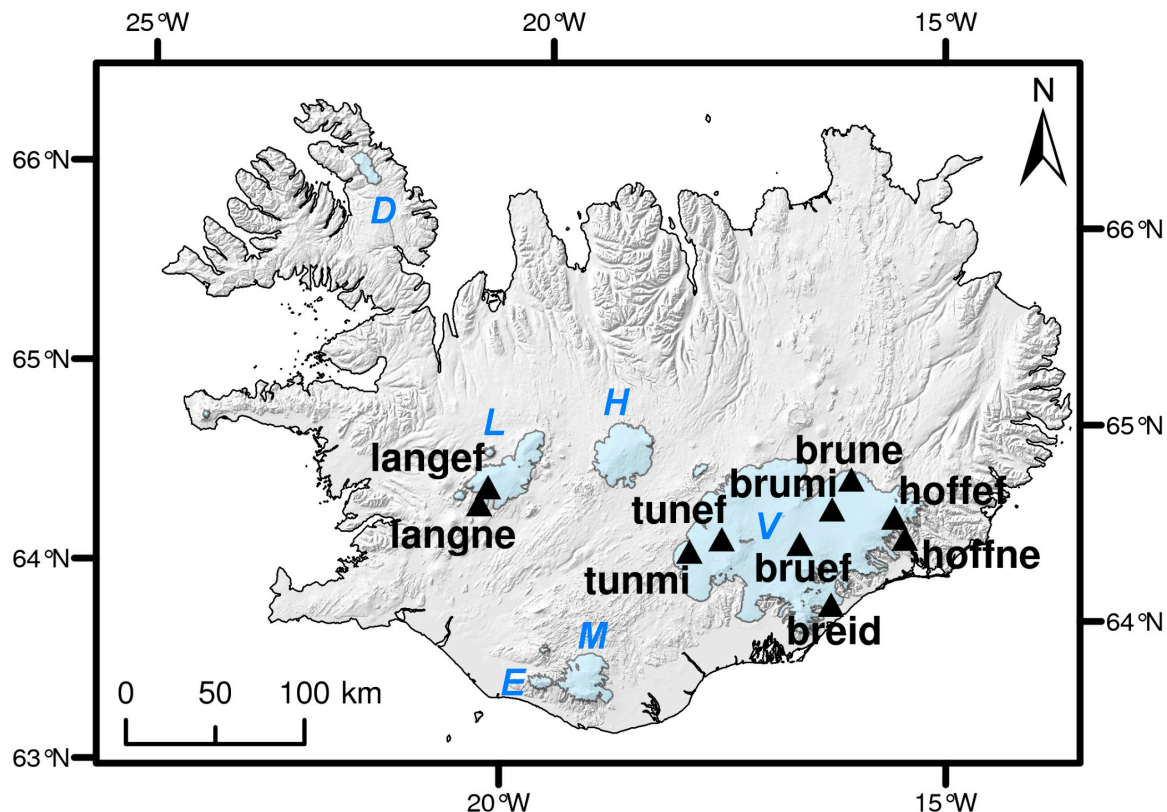
Figure 2. Map of Iceland showing the location of the AWSs on the Vatnajökull (brune, brumi, bruef, breid, tunef, tunmi, hoffef, hoffne) and Langjökull (langef, langne) ice caps. The main ice caps are labeled with a blue capital letter (D: Drangajökull, E: Eyjafjallajökull, H: Hofsjökull, L: Langjökull, M: Mýrdalsjökull, V: Vatnajökull).
