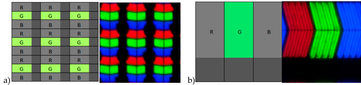
Figure 9: Comparison of idealized subpixel structures (only green glows) on the left with the real subpixel structures on the right. That is shown for a) display 1 (image display) and b) display 2 (color barrier)
