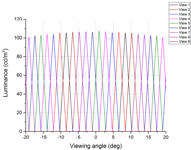
Figure 7: Luminance profiles for the 9-views of the multiview display design
