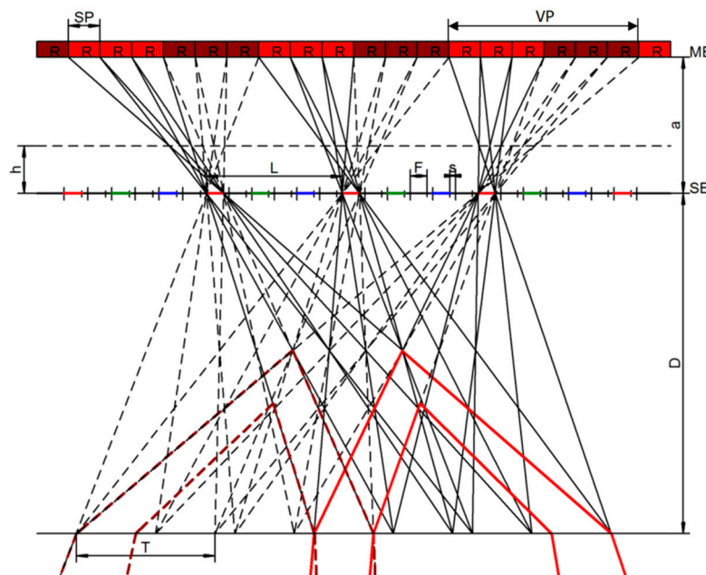
Figure 3: Top view, horizontal cross section of the display design for single-user mode. The left and the right view share always six red subpixels per group VP [19]
