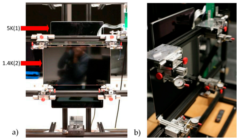
Figure 8: Demonstrator, with 90° crossed display panel, mounted at a metal frame and calibration fixture
