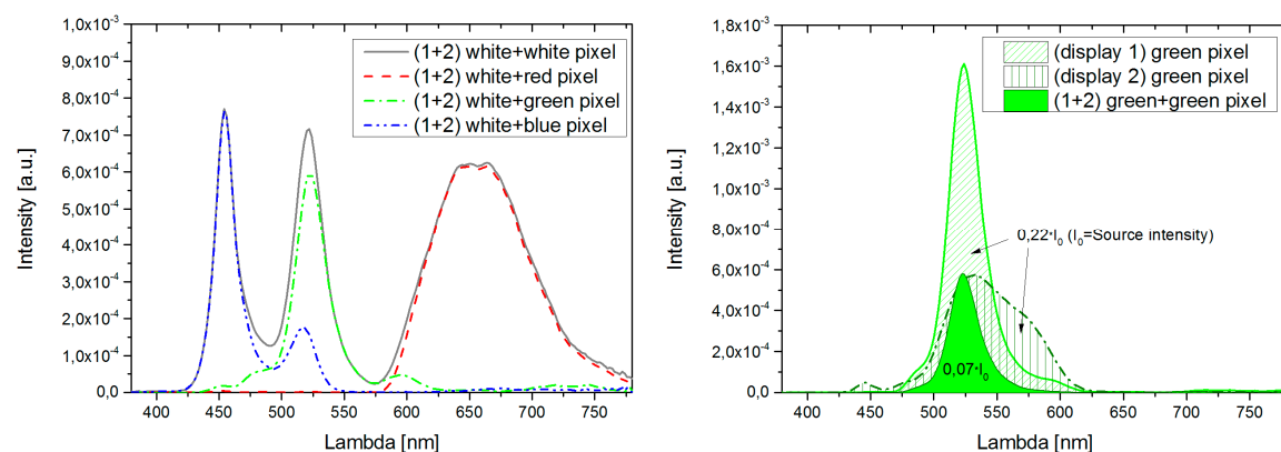
Figure 10: Left: 5K-display1 with white spectrum and 90° tilted 1.4K display 2 with single prime-colors, visible crosstalk of blue in green; Right: Spectral intensity of the green color primaries from both panels
