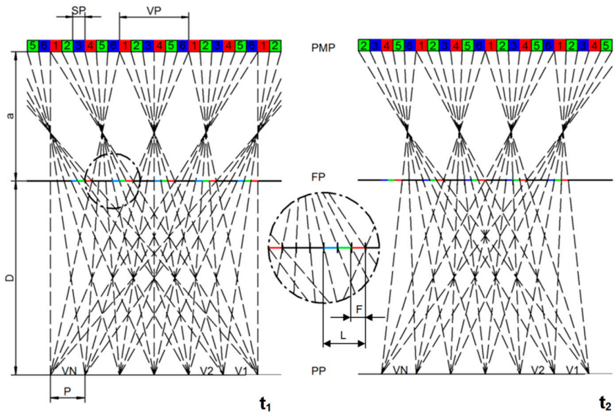
Figure 1: Principle of time-sequential operation of a wavelength-selective multiview 3D-display at the state on t_1 and t_2 with resolution enhancement in the same positioned viewing zones V1 to VN
