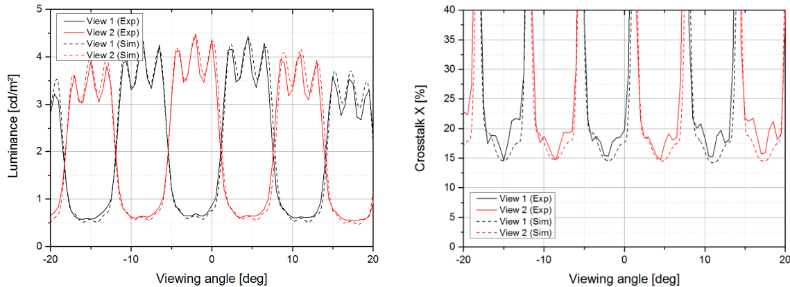
Figure 13. Simulated and experimental luminance and crosstalk of green, 3 channels green/3 channels black
