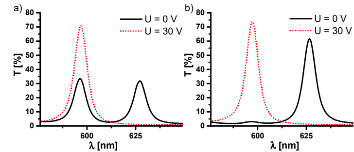
Figure 15: Transmission of device I in the off-state (—) and in the on-state (···) measured with non-polarized (a)) and with linear polarized (b)) incident light.
