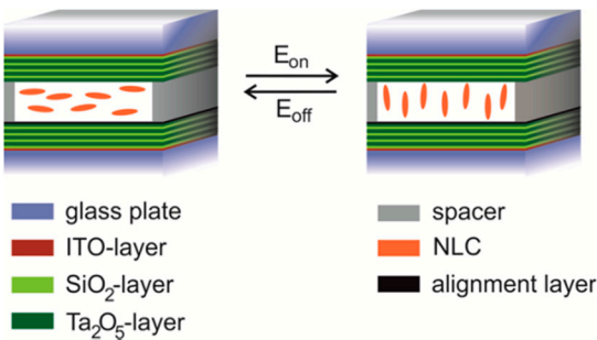
Figure 14: Overview of the basic configuration of the NLC Fabry-Pérot color filter and principle of the switching in an electric field E.
