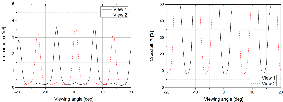
Figure 11. Experimental measured luminance and crosstalk green, 1 channel green/1 channel black
