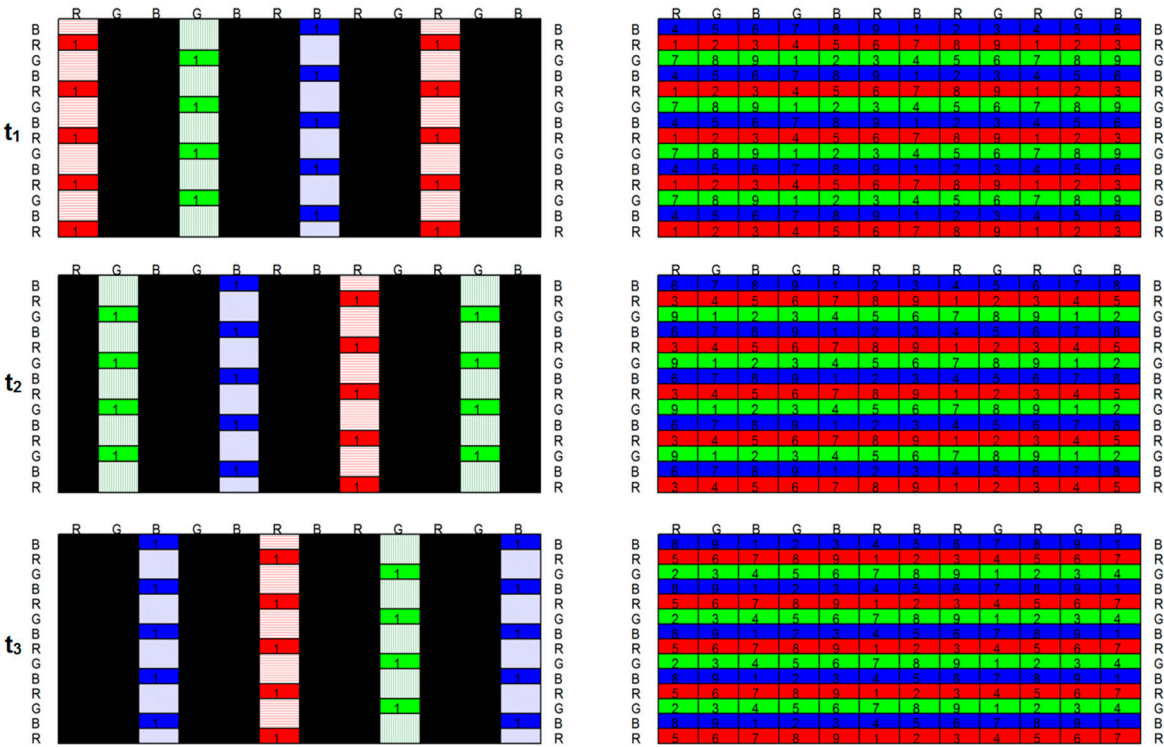
Figure 6: Multiview mode with special color filter scheme by using 9 views and 3 switching stages ( t_1 , t_2 , t_3 ); on the left illustrated the color filters and on the right the corresponding interleaving pattern.
