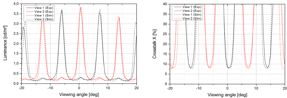
Figure 12. Simulated and experimental luminance and crosstalk of green, 1 channel green/1 channel black
