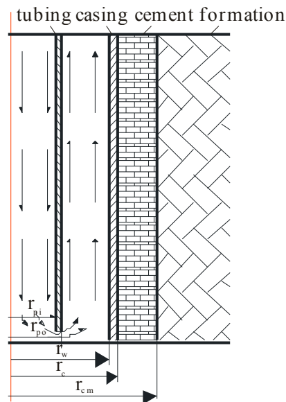
Figure 1. Circulation model parameter in the wellbore.
