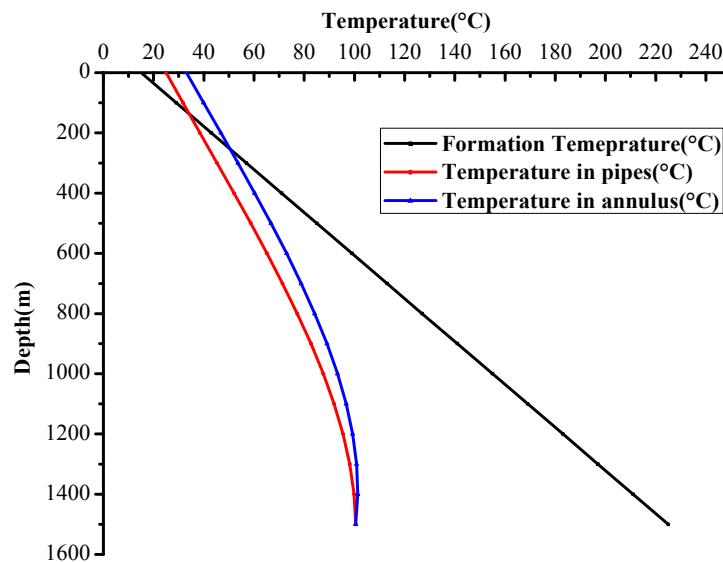
Figure 5. The temperature profile in the pipe and annulus (circulating 1 h).
