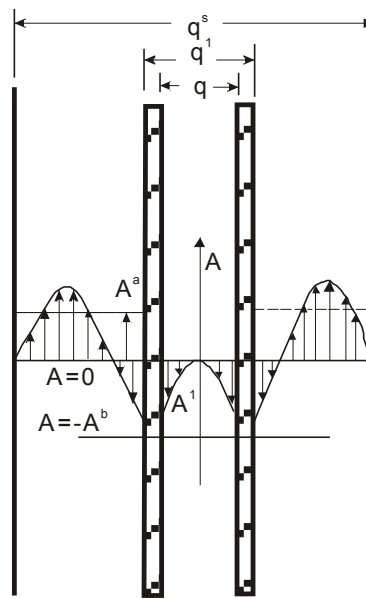
Figure 3. Velocity profiles for the laminar flow pattern when the pipe is pulled out of the well [28].
