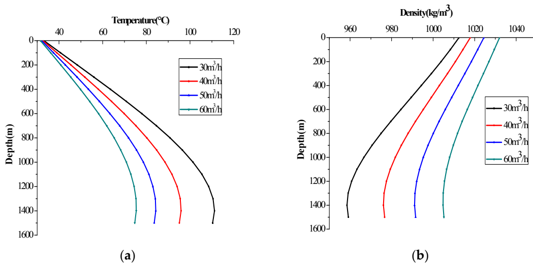
Figure 7. Temperature (a) and ECD (b) in the annulus with the flow rate (circulating 8 h).
