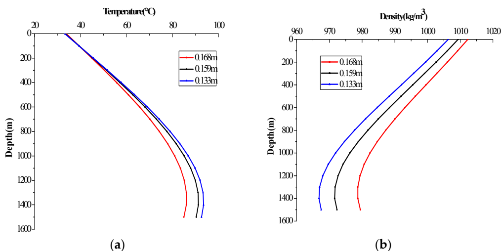
Figure 9. Temperature (a) and ECD (b) in the annulus with the outer diameter of the pipe (circulating 8 h).
