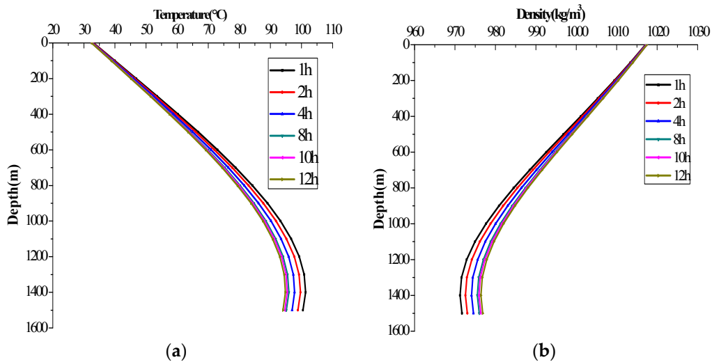
Figure 6. (a) Temperature in the annulus with the circulation time; (b) the ECD in the annulus with the circulation time.
