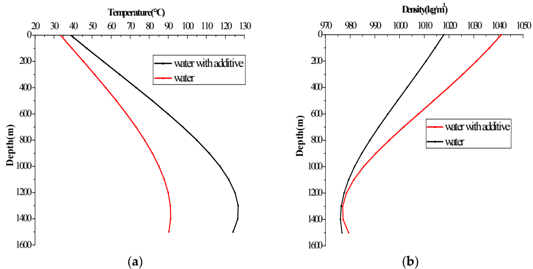
Figure 10. Temperature (a) and ECD (b) in the annulus with the rheological model of the pipe (circulating 8 h).
