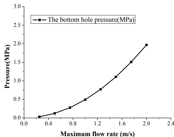
Figure 11. The bottom hole pressure with different rates of trip in.
