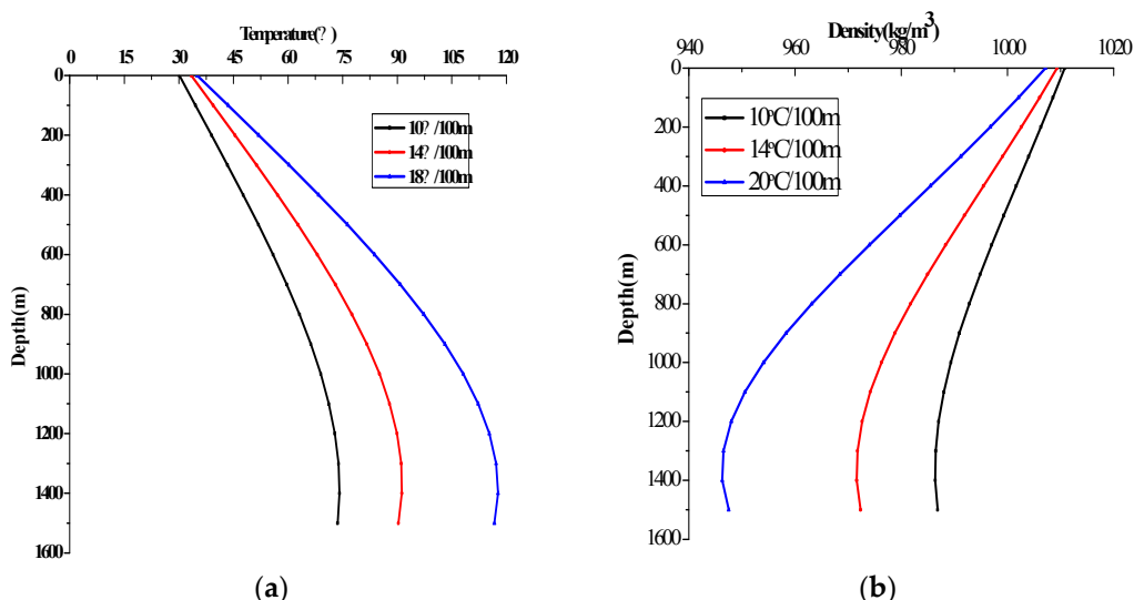
Figure 8. Temperature (a) and ECD (b) in the annulus with the geothermal gradient (circulating 8 h).
