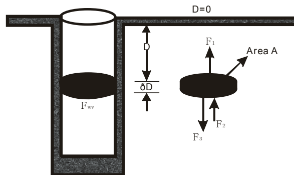
Figure 2. Forces acting on a fluid element [28].
