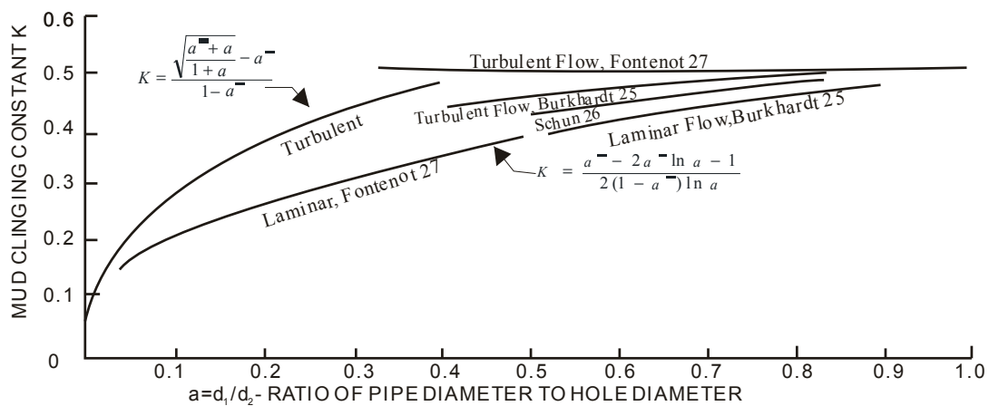
Figure 4. Drilling fluid clinging constant, K , for computing surge- and swab- pressure [29].
