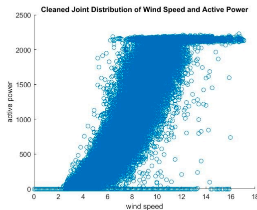
Figure 3. Power curve from the cleaned dataset
