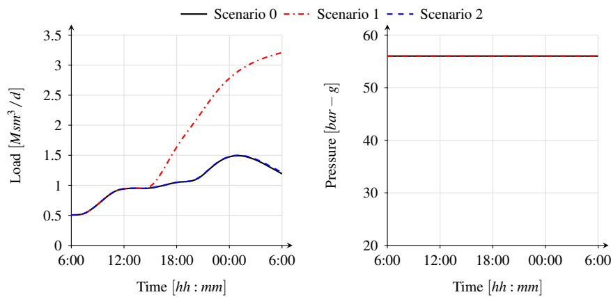
Figure 12. Time evolution of withdrawal rate and pressure at UGS facility for the computed scenarios
