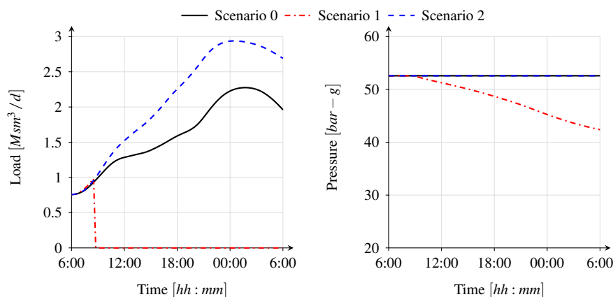
Figure 10. Time evolution of gas supply and pressure at the production field for the computed scenarios
