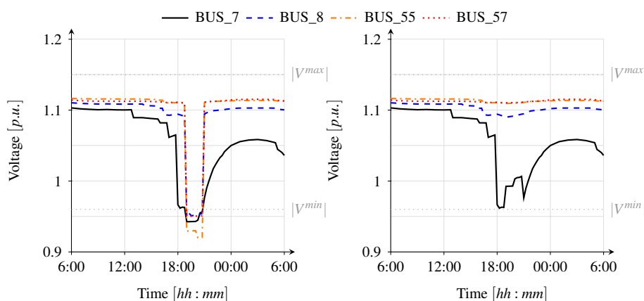
Figure 16. Time evolution of bus voltages before load shedding (left) and after (right) for scenario 2. Load shedding was applied at 15 buses. Among these buses are the 4 buses from scenario 1, which are shown in this figure.
