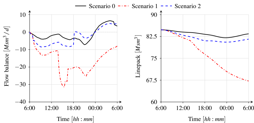
Figure 8. Time evolution of flow balance (sum of inflow minus sum of outflow) and line pack for the computed scenarios
