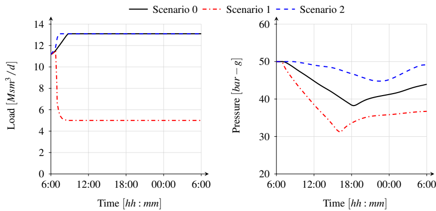
Figure 11. Time evolution of regasification rate and pressure at the LNG terminal for the computed scenarios
