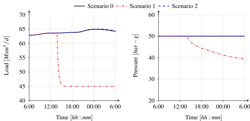
Figure 9. Time evolution of gas supply and pressure at the CBI node for the computed scenarios
