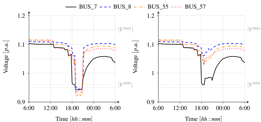
Figure 15. Time evolution of bus voltage before load shedding (left) and after (right) for scenario 1. All 4 buses where load shedding was applied are shown in this figure.
