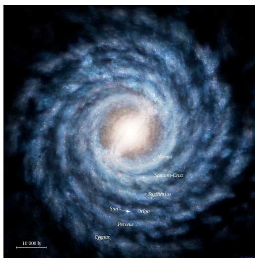
Figure 3: Milky Way (from http://www.atlasoftheuniverse.com/milkyway2.jpg )
