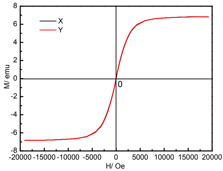
Figure s2 The different direction VSM of Fb at room temperature
