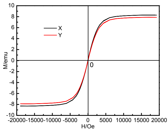
Figure s3 The different direction VSM of Fc at room temperature
