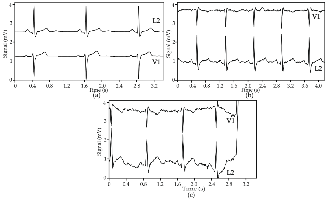
Figure 11. ECG signals obtained in ambulatory with holter monitoring device and patient ID = 1: (a) gel electrodes, rate 50 BPM; (b) textile electrodes, rate 74 BPM; (c) textile electrodes, rate 71 BPM, showing motion artifact interference leading to lost of signals .
