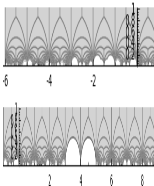
Figure 2. A schematic of the hyperbolic polygon on 765 tiles corresponding to the near polygon arising from the permutation group of O_8^-(2) . Pairs of edges of the same color have to be identified. The drawing is performed by using the software Sage that allows to visualize (in the hyperbolic half-plane) the permutation representation of a subgroup of PSL(2, \mathbb{Z}) [12, p. 752].
