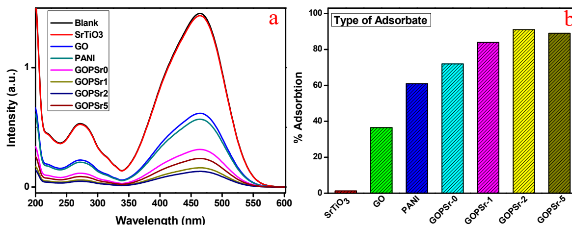
Figure 6. (a) UV-vis absorption spectra of MO aqueous in the presence of various adsorbents and (b) percentage removal of MB in the presence of various adsorbents (initial MO concentration: 20 mg·L -1 ; amount of adsorbent: 0.5 mg·mL -1 ; pH 7; time: 30 min; at room temperature).
