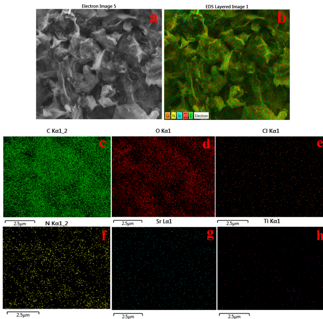
Figure 2. (a) FESEM image and (b) EDX elemental mapping of GOPSr-2 nanocomposite on a Si wafer for the following elements: (c) C, (d) O, (e) Cl, (f) N, (g) Sr, and (h) Ti.
