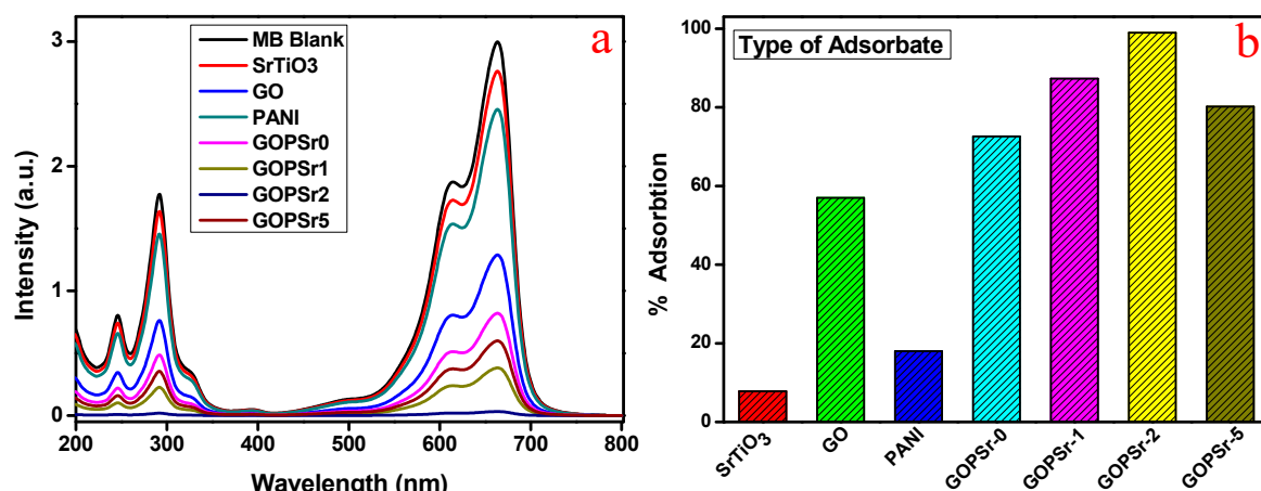
Figure 5. (a) UV-vis absorption spectra of MB aqueous in the presence of various adsorbents and (b) percentage removal of MB in the presence of various adsorbents (initial MB concentration: 20 mg·L -1 ; amount of adsorbent: 0.5 mg·mL -1 ; pH 7; time: 30 min; at room temperature).
