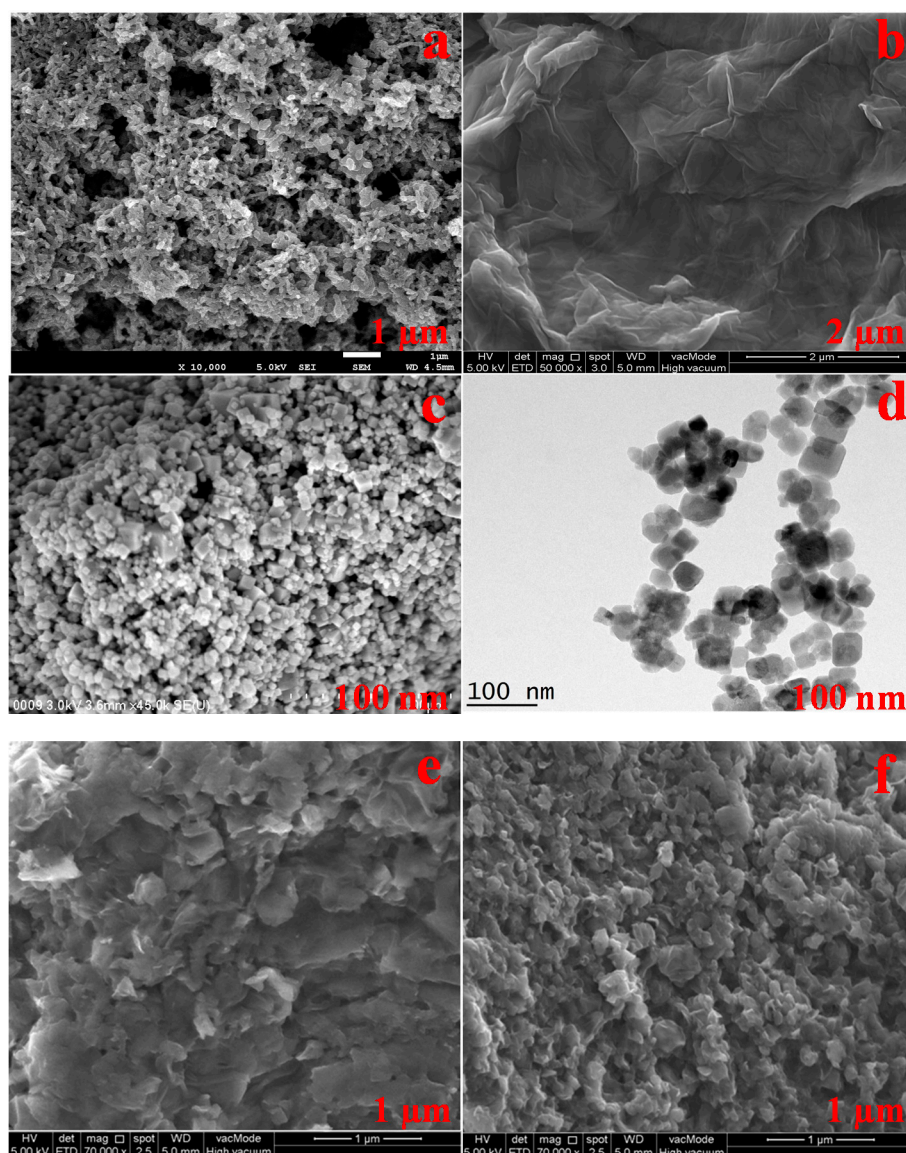
Figure 1. FESEM micrographs of (a) PANI, (b) GO, (c) \text{SrTiO}_3 nanocubes, (e) GOPSr-0, and (f) GOPSr-2 nanocomposite; and (d) TEM image of \text{SrTiO}_3 nanocubes.
