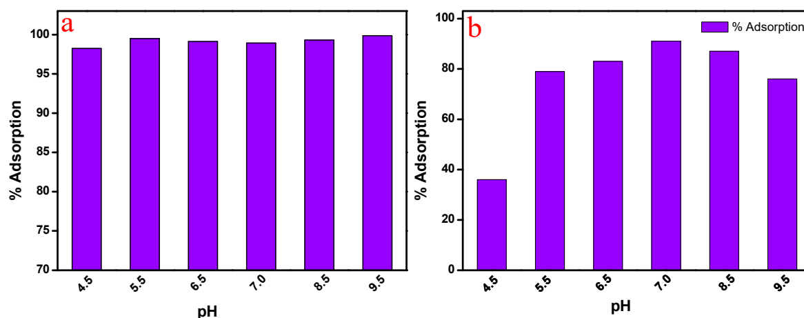
Figure 9. Effect of pH on percentage removal of (a) MB and (b) MO in the presence of GOPSr-2 (initial MB and MO concentration: 20 mg·L -1 ; amount of adsorbent (MB): 0.5mg·mL -1 , (MO): 2 mg·mL -1 ; time: 30 min at room temperature).
