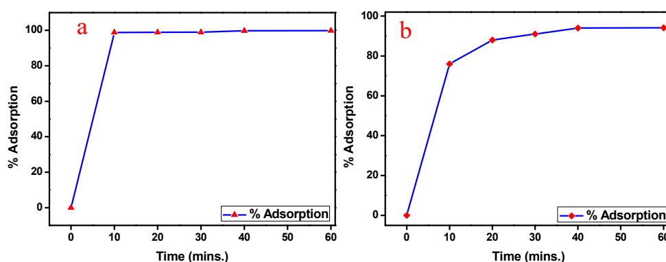
Figure 8. Effect of time on percentage removal of (a) MB and (b) MO in the presence of GOPSr-2 (initial MB and MO concentration: 20 mg·L -1 ; amount of adsorbent (MB): 0.5 mg·mL -1 , (MO): 2 mg·mL -1 ; pH (MB): 9.5, (MO): 7; at room temperature).
