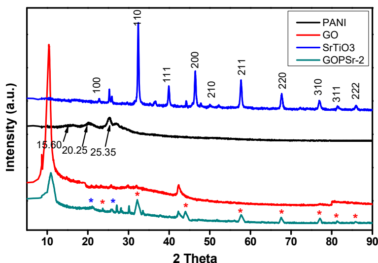
Figure 4. XRD pattern of PANI, GO, \text{SrTiO}_3 , and GOPSr-2.
