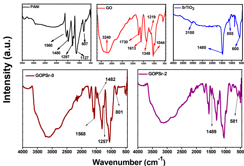
Figure 3. FTIR spectra of PANI, GO, \text{SrTiO}_3 , GOPSr-0, and GOPSr-2.
