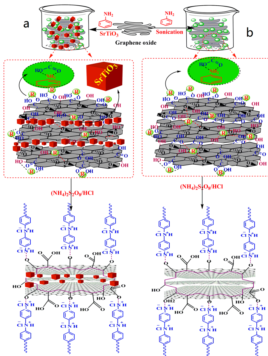
Scheme 1. Reaction pathway for the synthesis of PANI-coated GO nanocomposite (a) doped with \text{SrTiO}_3 and (b) without \text{SrTiO}_3 (dotted lines represent hydrogen bonding, \pi - \pi interactions, and electrostatic interactions of PANI with GO).
