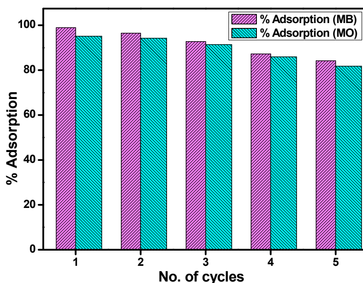
Figure 11. Reproducibility cycles of GOPSr-2 for (a) MB and (b) MO adsorption (initial MB and MO concentration: 20 mg·L -1 ; amount of adsorbent (MB): 0.5 mg·mL -1 , (MO): 2 mg·mL -1 ; pH (MB): 9.5, (MO): 7; at room temperature).
