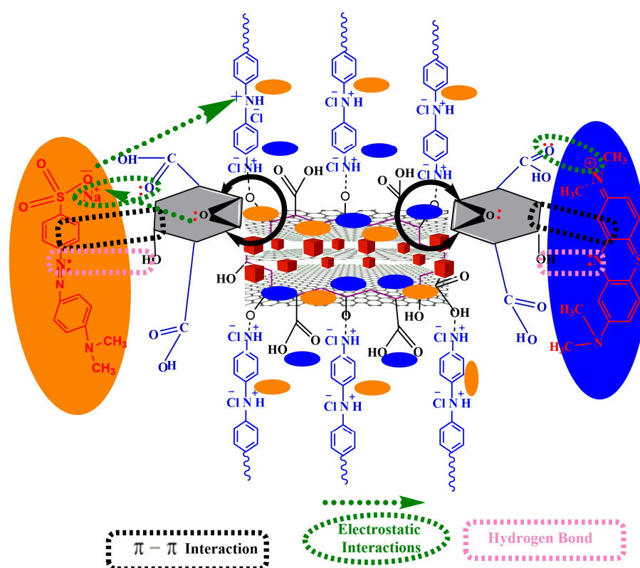
Scheme 2. Proposed mechanism for the adsorption of MB and MO on the surface of GOPSr-2.
