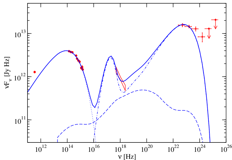
Figure 2. Fit to the SED of the LBL AO 0235+164 (data from [3]), with \eta_1 = 225 and \alpha = 3 . Note that the soft X-ray excess (Big Blue Bump) is reproduced by the bulk Compton emission of the thermal electron population. From [4].
