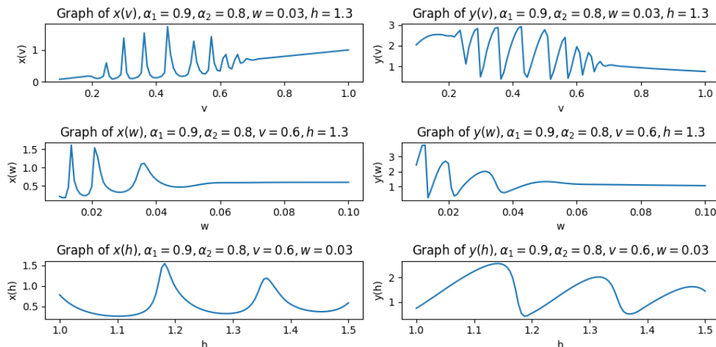
Figure 8. Bifurcation diagrams of the dependence of the solution x and y on various values of the model parameters.
