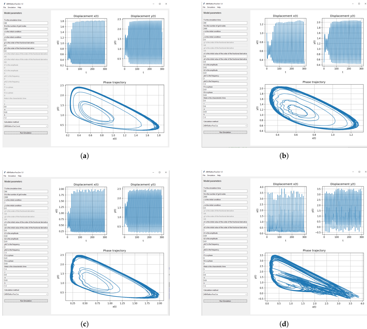
Figure 2. Calculation results: (a) \alpha_1 = 0.8, \alpha_2 = 0.9, \theta = 1 [4]. (b) \alpha_1 = 0.8, \alpha_2 = 0.9, k_1 = 0.02, k_2 = 0.01, \phi_1 = 3, \phi_2 = 1.5, f_1 = 0.01, f_2 = 0.03, \theta = 0.5 . (c) \alpha_1 = 0.8, \alpha_2 = 0.9, k_1 = 0.02, k_2 = 0.01, \phi_1 = 3, \phi_2 = 1.5, f_1 = 0.01, f_2 = 0.03, \theta = 1.5 . (d) \alpha_1 = 0.8, \alpha_2 = 0.9, k_1 = 0.02, k_2 = 0.01, \phi_1 = 3, \phi_2 = 1.5, f_1 = 0.01, f_2 = 0.03, \theta = 3 .
