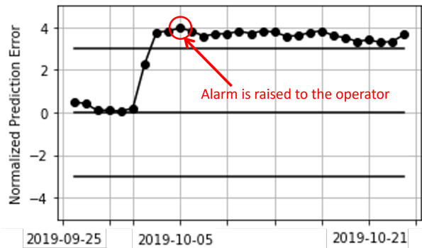
Figure 4. Calculated prediction error for an inverter fan malfunction for the NBM model. The algorithm sends daily alarms to the operator until the problem is corrected and the error returns to the acceptable range.
