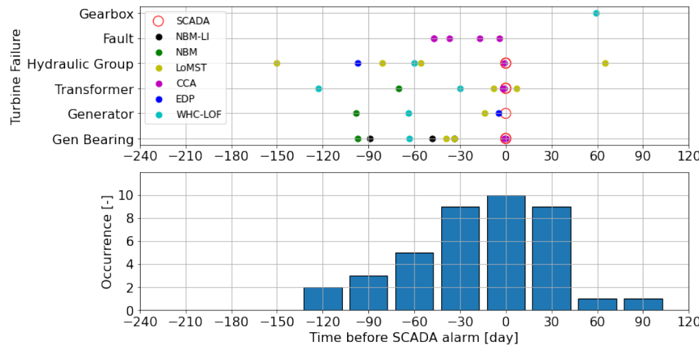
Figure 11. Time before annotated failure for each model and the its distribution.
