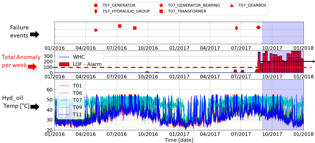
Figure 6. Time series of hydraulic oil temperature of the five turbines and the total anomaly per week detected by WHC-LOF method (red bar). The red dashed line is the threshold alarm when the cumulative anomaly event is above 100/week. The black arrow indicates the expected failure in the next weeks.
