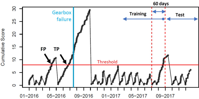
Figure 5. . Illustration of how the combined LoMST and cumulative sum of anomaly score (LoMST-CUSUM) is used to establish failures detection. In this example, the blue line indicates the time at which a gearbox failure happened. The parameters are defined based on the training data in five turbines.
