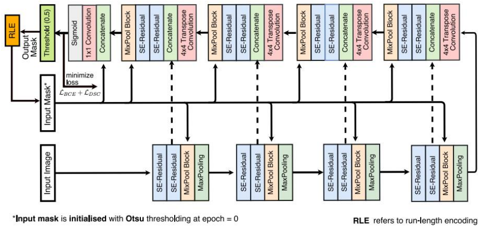
Figure 3. FANet Framework.
