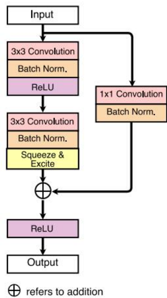
Figure 1. SE-Residual Block.
