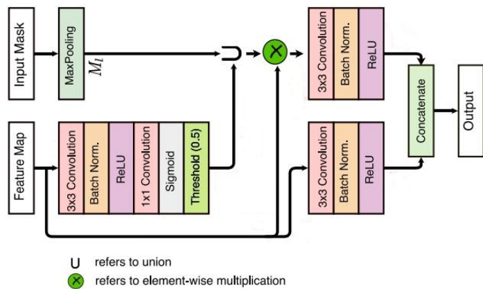
Figure 2. MixPool Block.
