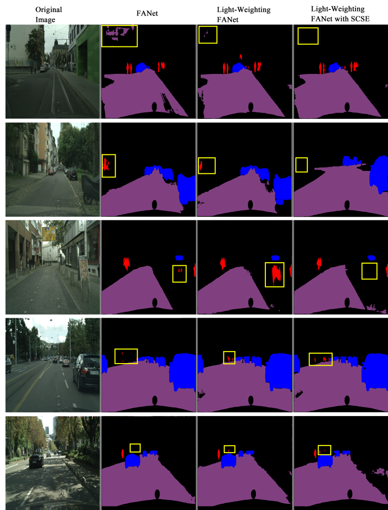
Figure 11. Visulization Results.
