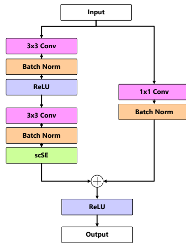
Figure 8. Structure of scSE-Residual.
