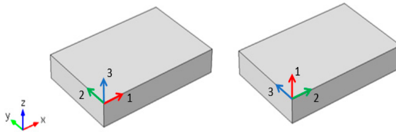
Figure 3. Piezoelectric material poling direction on COMSOL Multiphysics.
