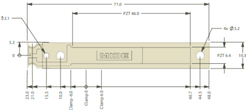
Figure 2. Detailed dimensions for MIDE PPA-1021 and layers composition.
