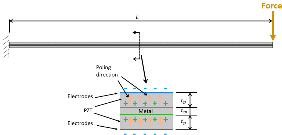
Figure 10. A schematic for the modeled triple-layer bender for Park & Moon [9] and Wang & Cross [10].
