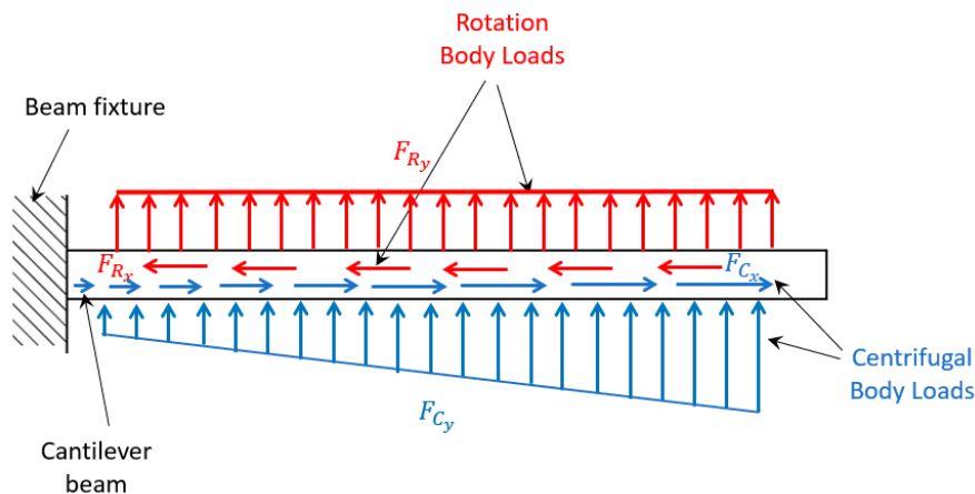
Figure 5. Effect identification of the different force across the harvester on COMSOL Multiphysics.
