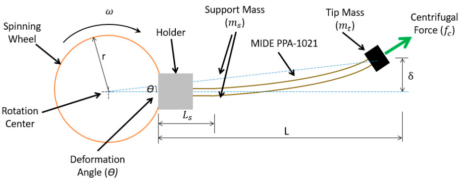
Figure 1. Harvester detailed construction.
