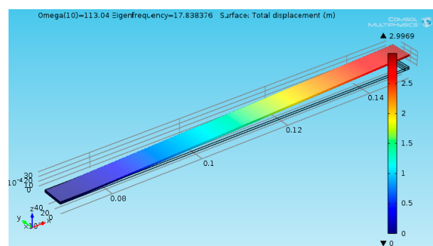
Figure 12. Numerical model using COMSOL Multiphysics.
