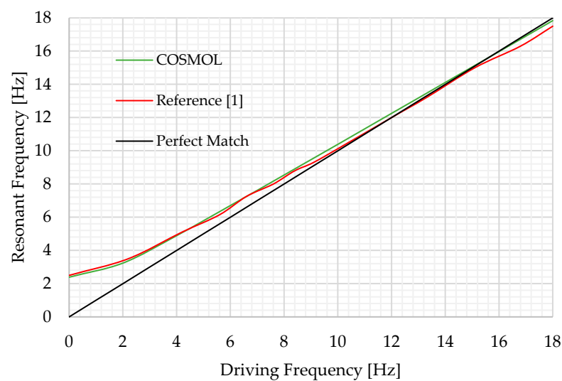
Figure 11. Data comparison between finite element numerical model, reference [1] and perfect match line.
