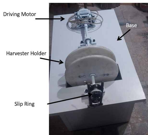
Figure 8. Experimental setup.
