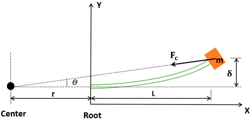
Figure 9. Effect of centrifugal force on beam tip deflection [1].
