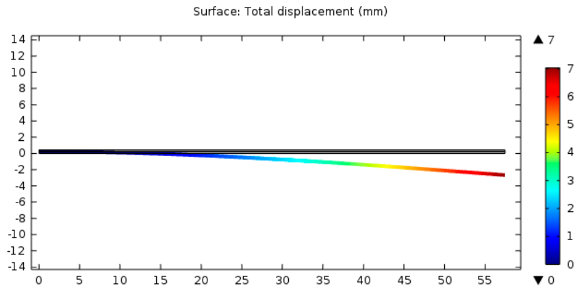
Figure 13. Simulated tip deformation mm due to applied tip force N and voltage difference (V) on numerical model.
