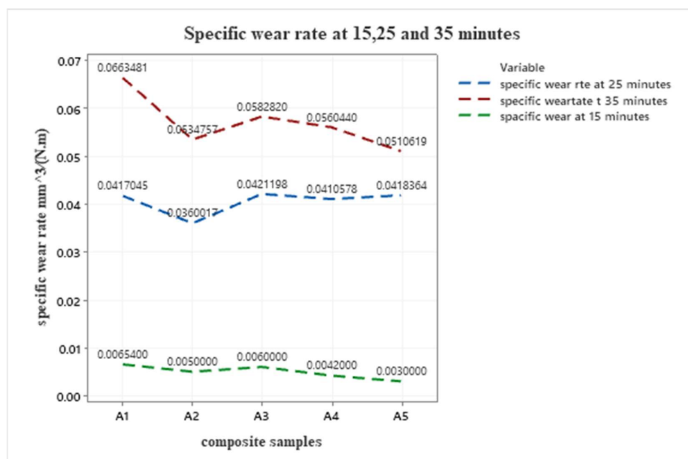
Figure 3. The specific wear rate of the hybrid composite samples at 15, 25, and 35 minutes of testing time.
