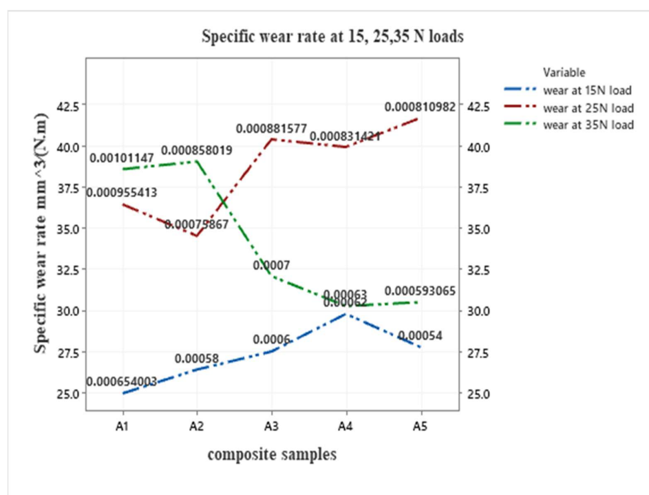
Figure 2. Specific wear rate of the hybrid composite at 15, 25, and 35 N applied loads.
