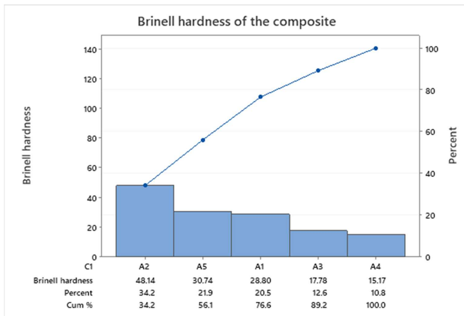
Figure 8. Brinell hardness results of the composite materials.
