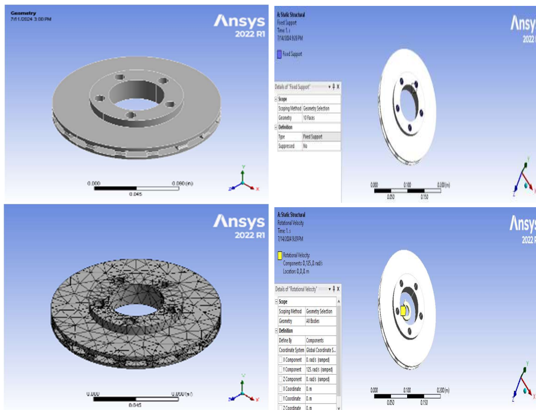
Figure 9. ANSYS model, meshing and constraints of the disk brake.
