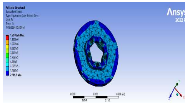
Figure 11. Von misses stress of the hybrid composite disk brake.
