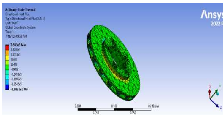
Figure 16. Steady state directional heat flux of the composite disk brake.
