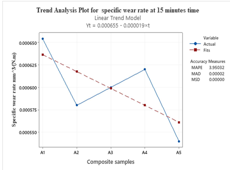
Figure 4. Linear trend model at 15 min of the specific wear rate.
