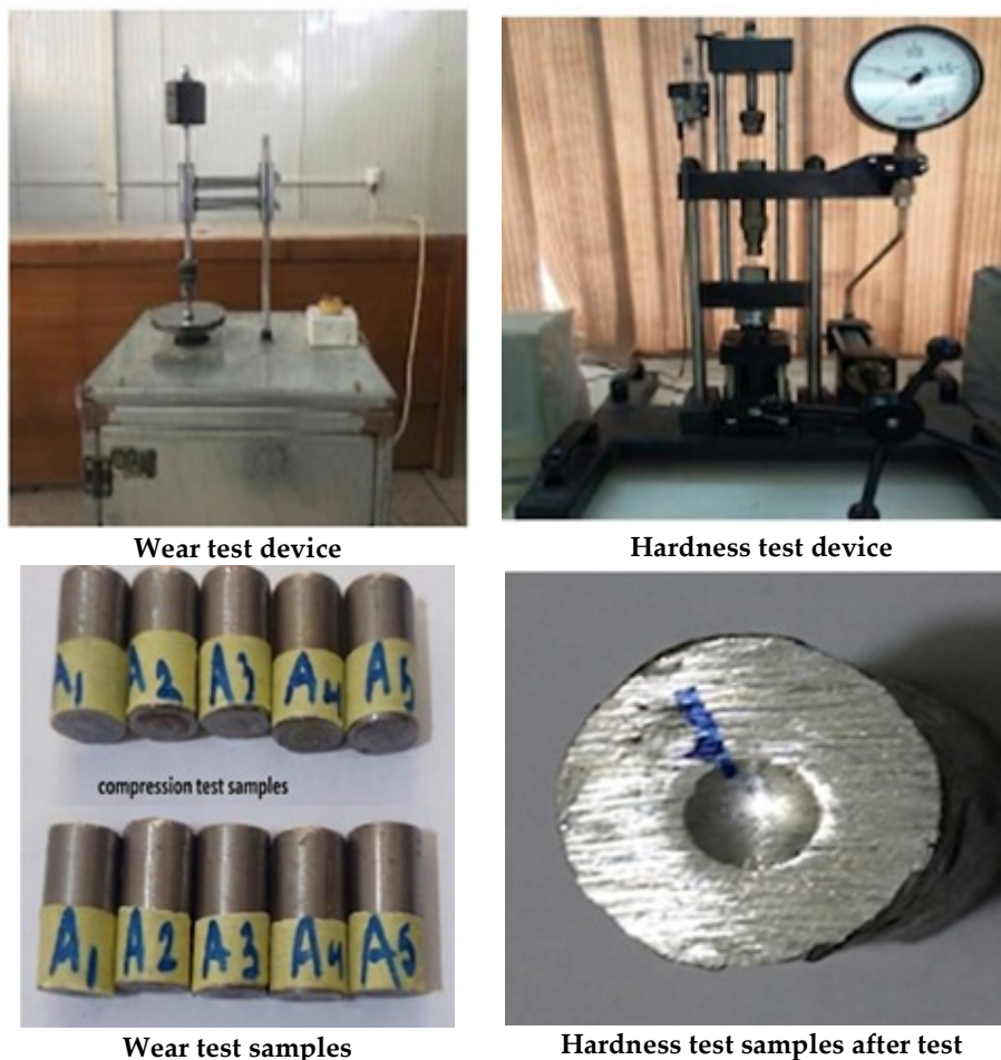
Figure 1. The aluminum-based hybrid composite compression, wear, BHN hardness tests samples, and wear, hardness test devices.
