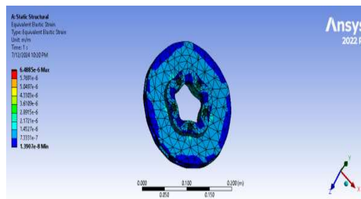
Figure 13. Equivalent elastic strain of disk brake composite.
