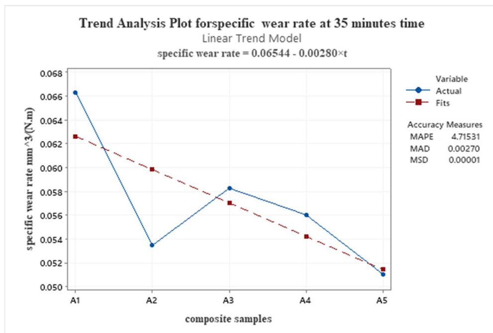
Figure 6. The trend analysis of specific wear rate.
