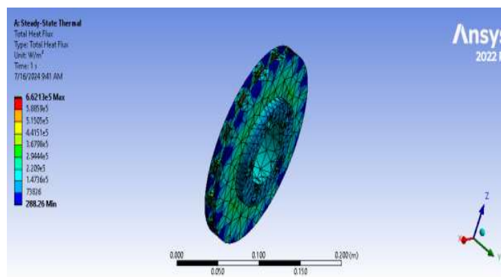
Figure 15. Total heat flux of the hybrid composite disk brake.
