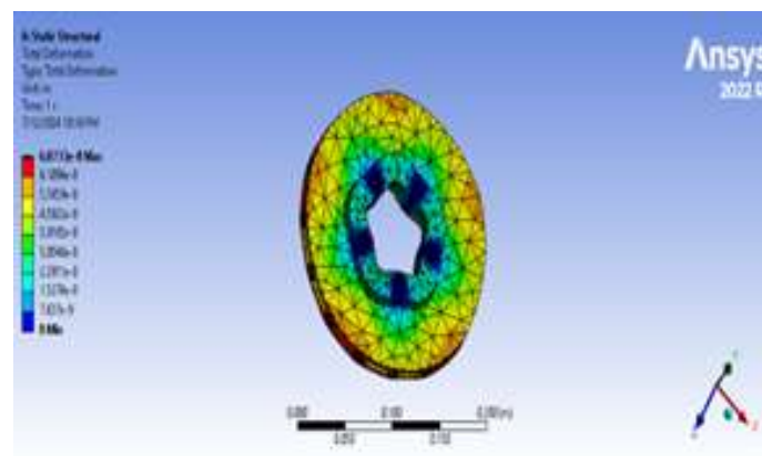
Figure 12. Total deformation of the hybrid composite disk brake.
