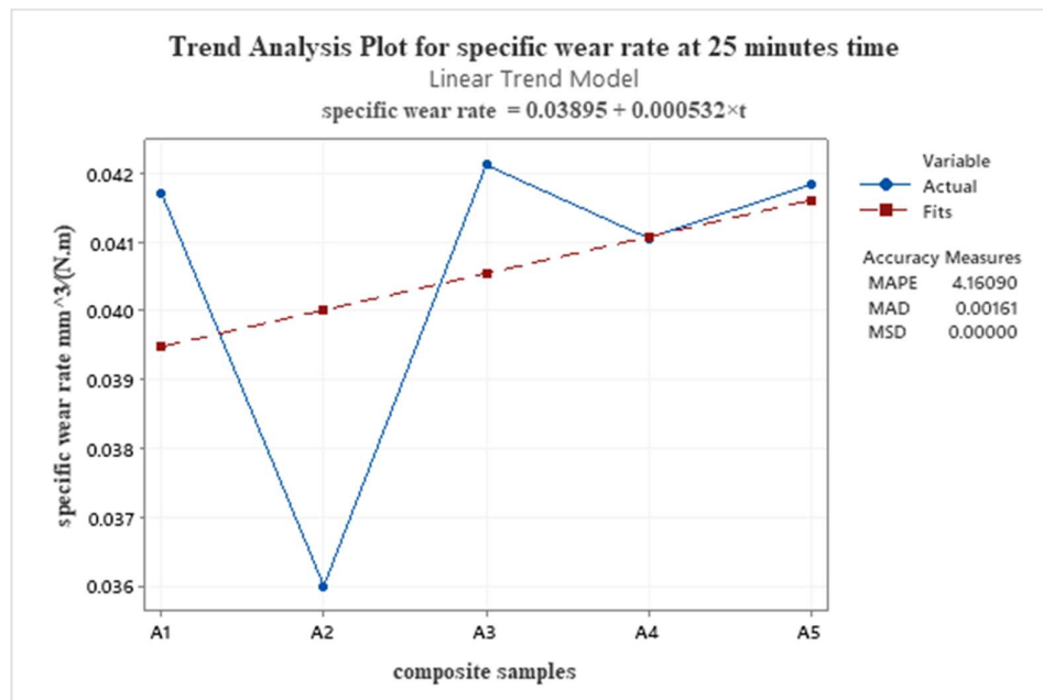
Figure 5. The linear trend model of the specific wear rate at 25 min time.
