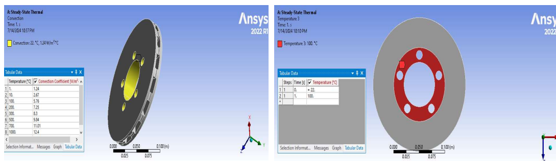
Figure 10. Thermal loads of the hybrid composite disk brake.
