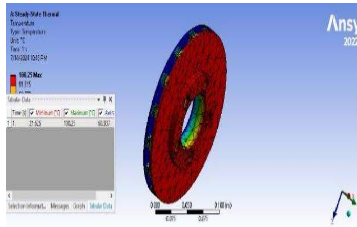
Figure 14. Temperature distribution of the hybrid composite disk brake.
