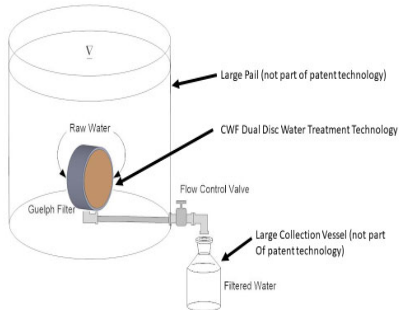
Figure 5. Schematic of Large Raw Water Pail, with GWF Treating the Water and Delivery of Water to the Filtered Water Retainer.
