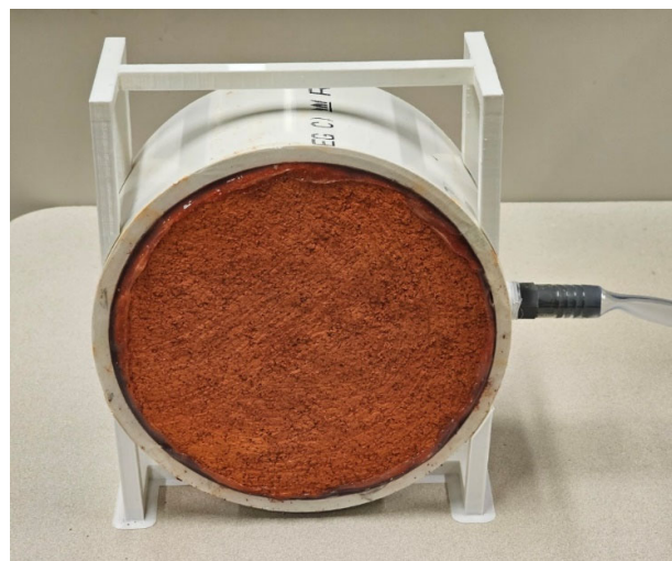
Figure 6. Photo of GWF of Ceramic Filter showing the Stand, the Handle (on top), and the Exit Tube which Carries the Treated Water to the Filtered Water Container.
