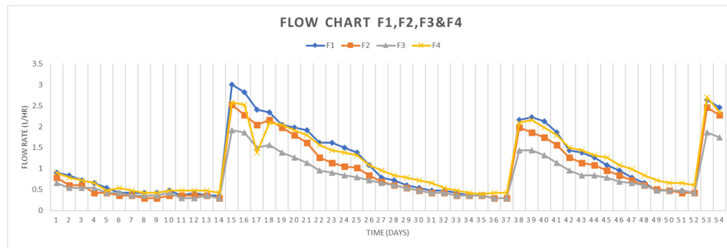
Figure 7. Flow Rates Through Four Ceramic Disks Versus Time.
