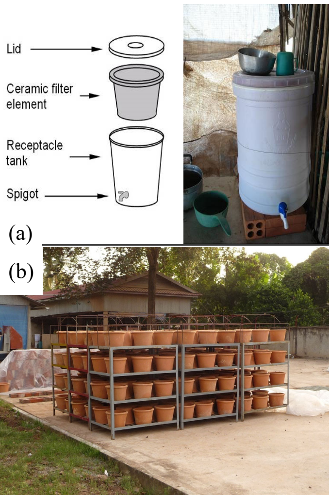
Figure 2. (a) CPF in Receptacle Tank;(b) Air-Drying After Firing of CPF (at RDI, Cambodia).
