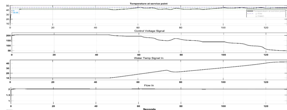
Figure 10: Performance of the fuzzy controller with Linear increase of Central Heater water temperature at maximum flow.
