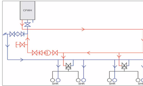
Figure 2. Example of a circulating warm water system controlled by a continuous flow water heater.
