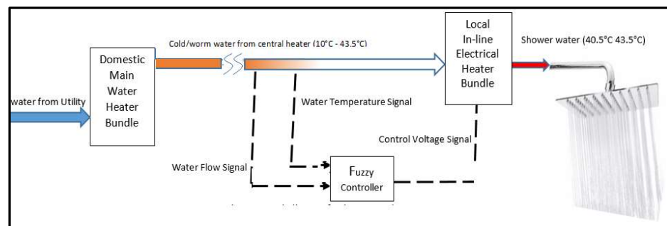
Figure 5. Block diagram for the proposed system.
