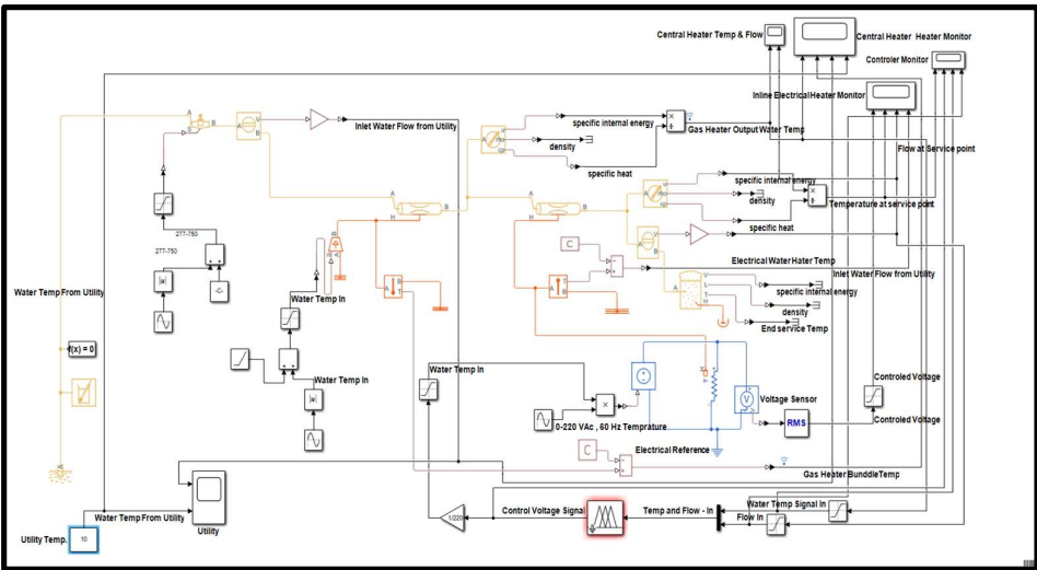
Figure 6. Simulink model
