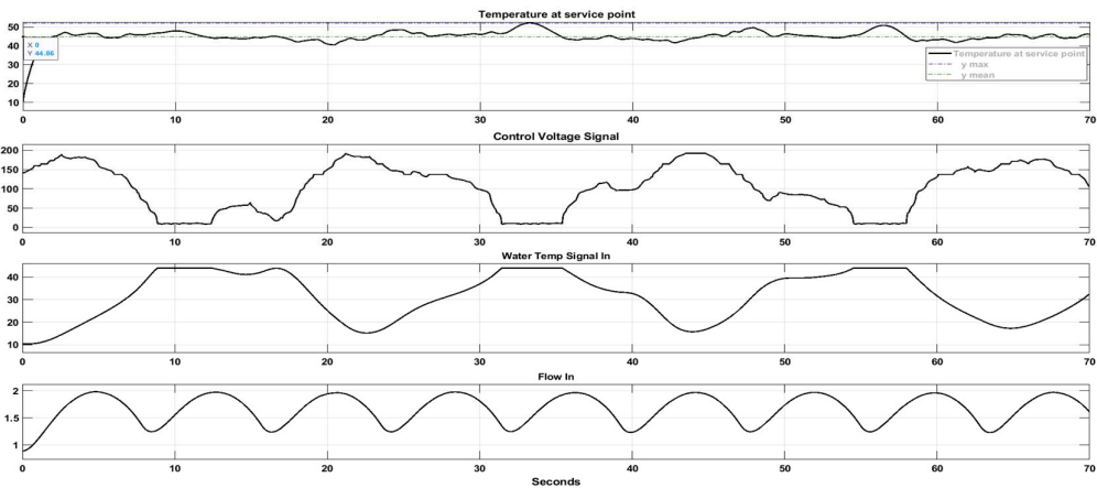
Figure 8. Nonlinear “Fast” flow fluctuation performance of the fuzzy controller
