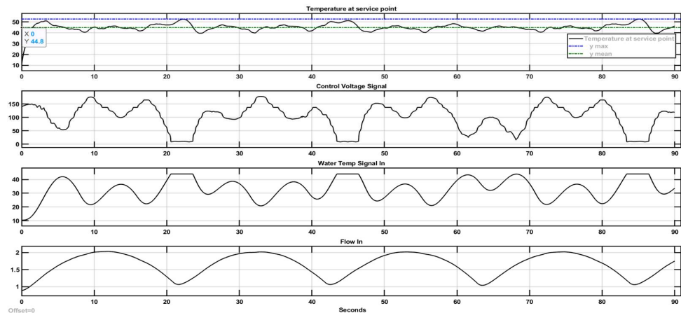
Figure 7. Nonlinear “slow” flow fluctuation performance of the fuzzy controller.
