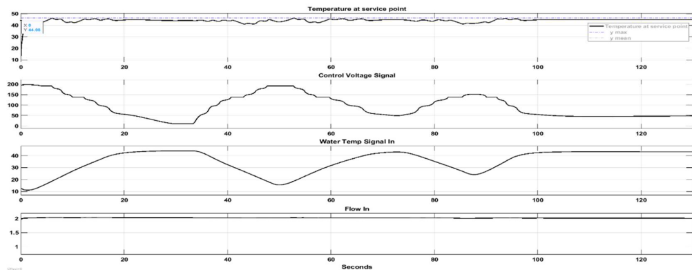
Figure 9: Performance of the fuzzy controller with Central Heater Fluctuation at maximum flow.
