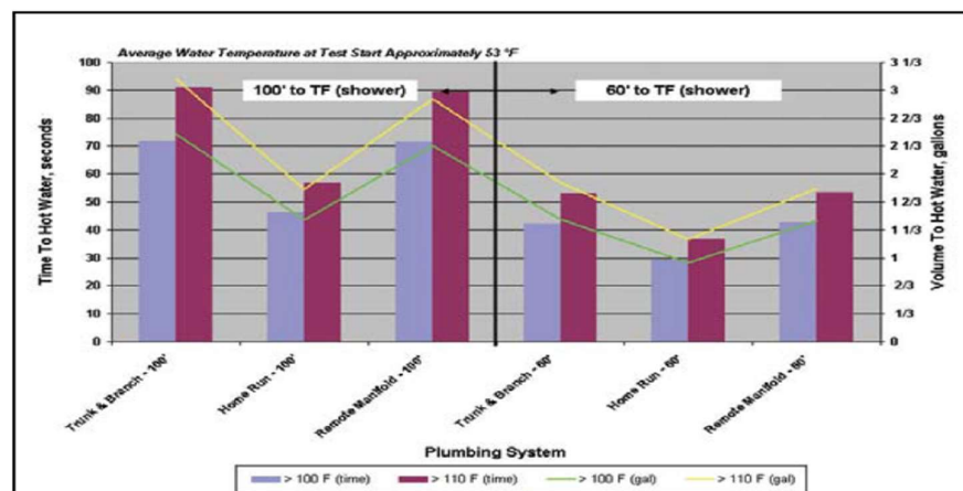
Figure 4. Comparison of Hot Water Delivery Time
