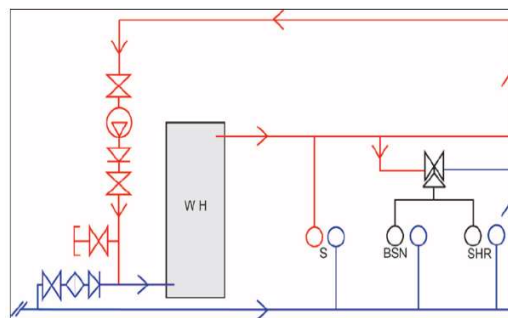
Figure 1. Example of a circulating warm water system controlled by a thermostatic mixing valve
