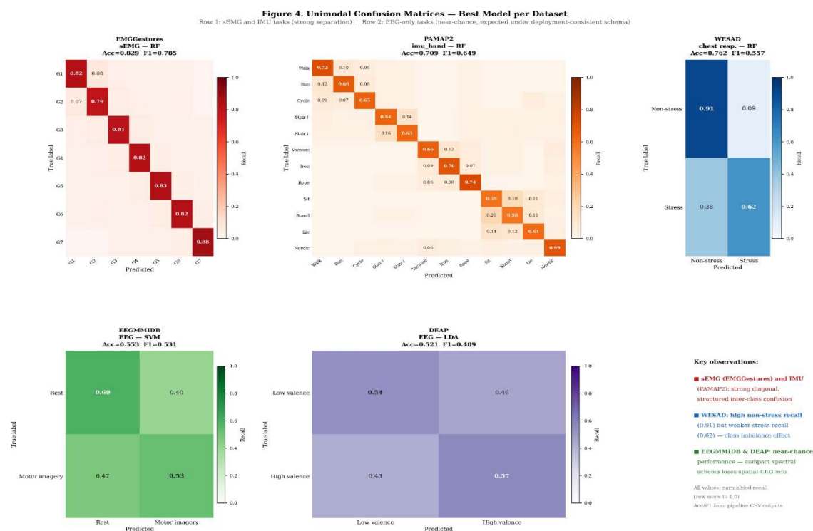
Figure 4. Representative confusion summaries for the strongest unimodal configurations across the evaluated public repositories. The panels illustrate class-wise prediction structure under subject-disjoint evaluation and highlight the contrast between higher-separation sEMG/IMU tasks and lower-separation EEG-only tasks under the deployment-consistent feature schema.
