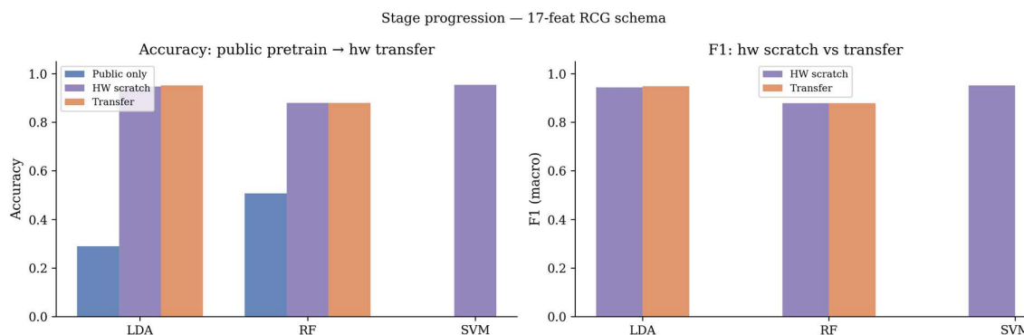
Figure 7. Stage progression of the RCG adaptation pipeline under the final 17-feature schema. The left panel compares public-only, hardware-scratch, and transfer accuracies for LDA, RF, and SVM, whereas the right panel contrasts hardware-scratch and transfer macro-F1 values for the same classifiers. The figure shows that public pretraining preserves a schema-consistent analytical starting point, but the final deployment-facing behaviour remains determined by hardware-aligned learning under session-disjoint evaluation across five bench sessions.
