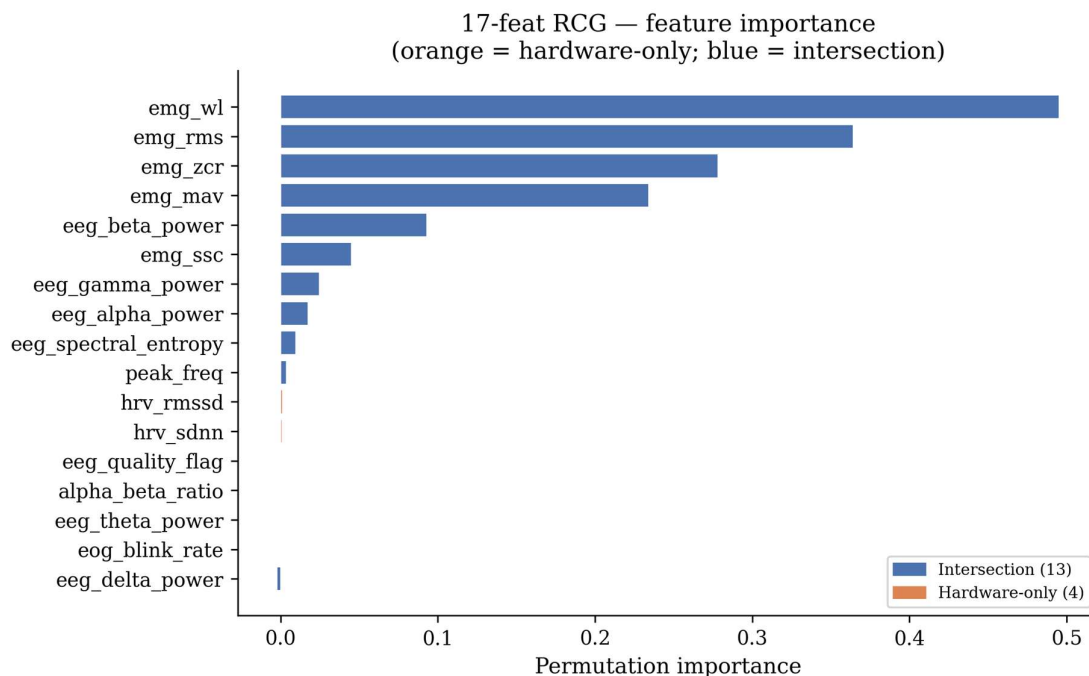
Figure 9. Feature importance for the final 17-feature RCG hardware branch, shown as permutation importance and grouped by intersection features versus hardware-only variables. The dominant contributors are emg_wl , emg_rms , emg_zcr , and emg_mav , followed by eeg_beta_power . In contrast, the hardware-exclusive variables related to HRV, EOG blink rate, and EEG quality remain negligible under the current bench-acquired data regime.
