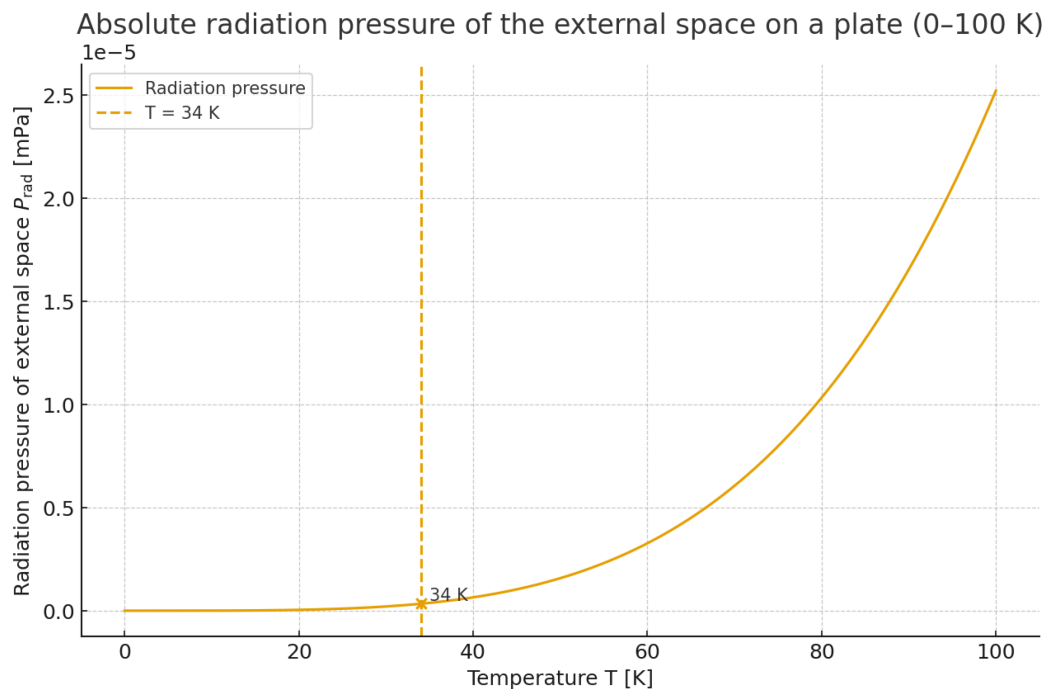
Figure A1. Absolute radiation pressure of the external space, inferred from the Casimir force on a plate, as a function of temperature. The dashed vertical line marks the thermal suppression scale at T \approx 34 K, below which thermal modes no longer contribute significantly to the vacuum spectrum.
