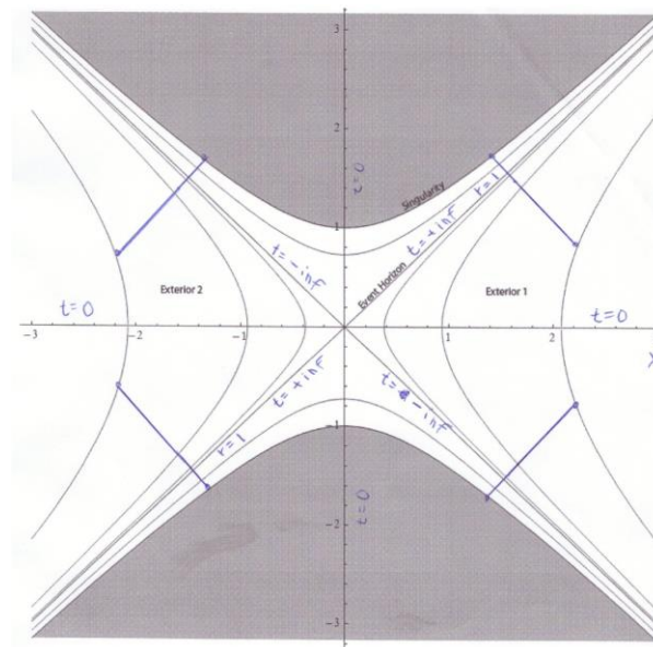
Figure 3b. A Kruskal-chart (T,X) with four alternatives of a world-line of a photon that falls into a black hole.
