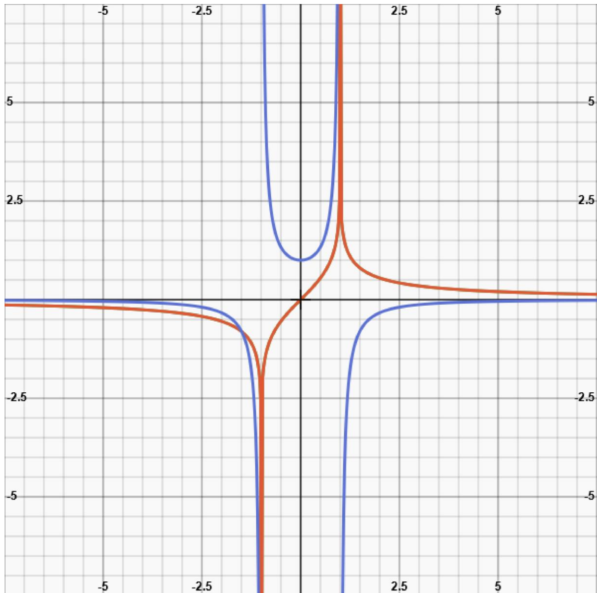
Figure 2a. World-line in red colour (in a t,r -diagram) of a radio signal sent off from the Milky Way. The cosmic event horizon is at r=1 . The area to the left of the vertical axis has no significance, since a negative r does not exist.
