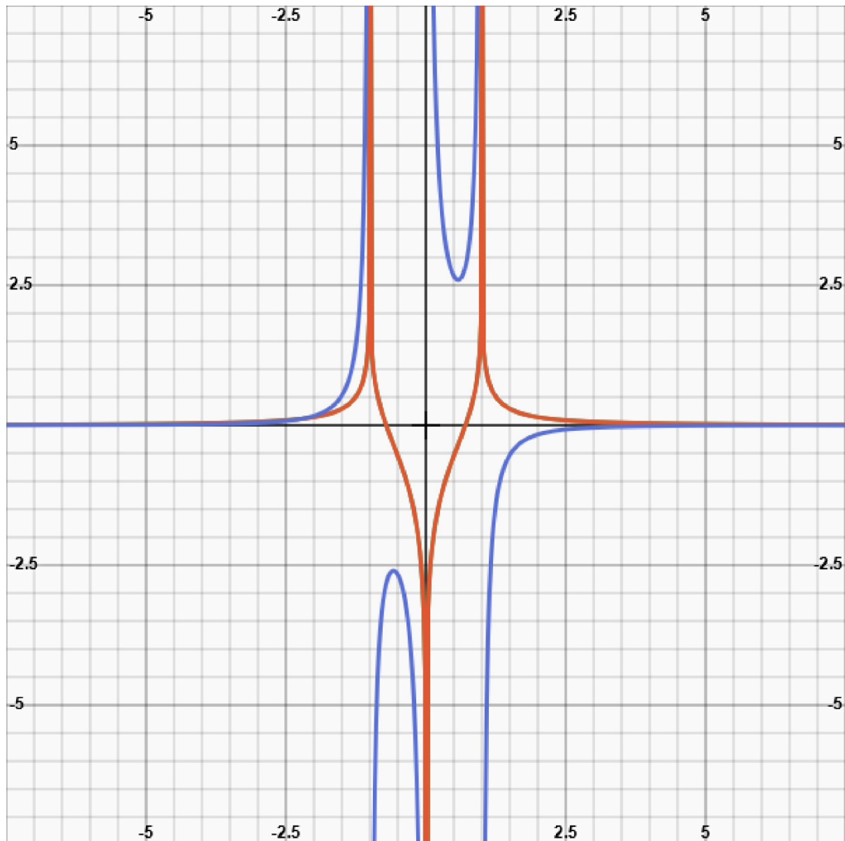
Figure 1a. World-Line Of An Escaping Galaxy In A T,R-Diagram In Red Colour. The Cosmic Event Horizon Is At R=1 . The area to the left of the vertical axis has no significance, since a negative r does not exist.
