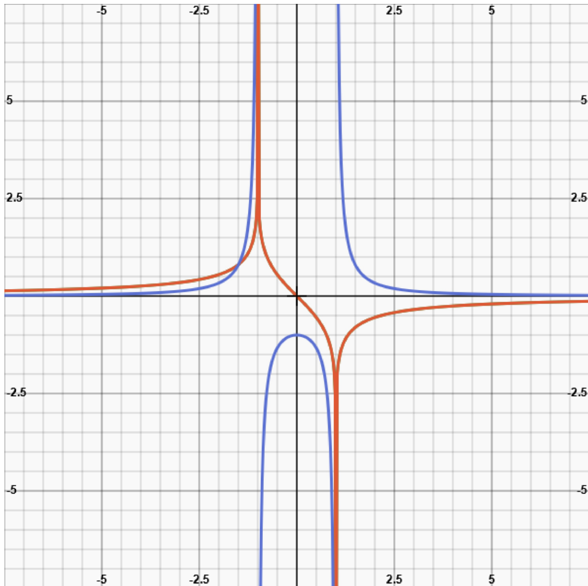
Figure 2b. World-line (in a t,r -diagram) sent to the Milky Way from beyond the Milky Way's cosmic event horizon. The area to the left of the vertical axis has no significance, since a negative r does not exist.
