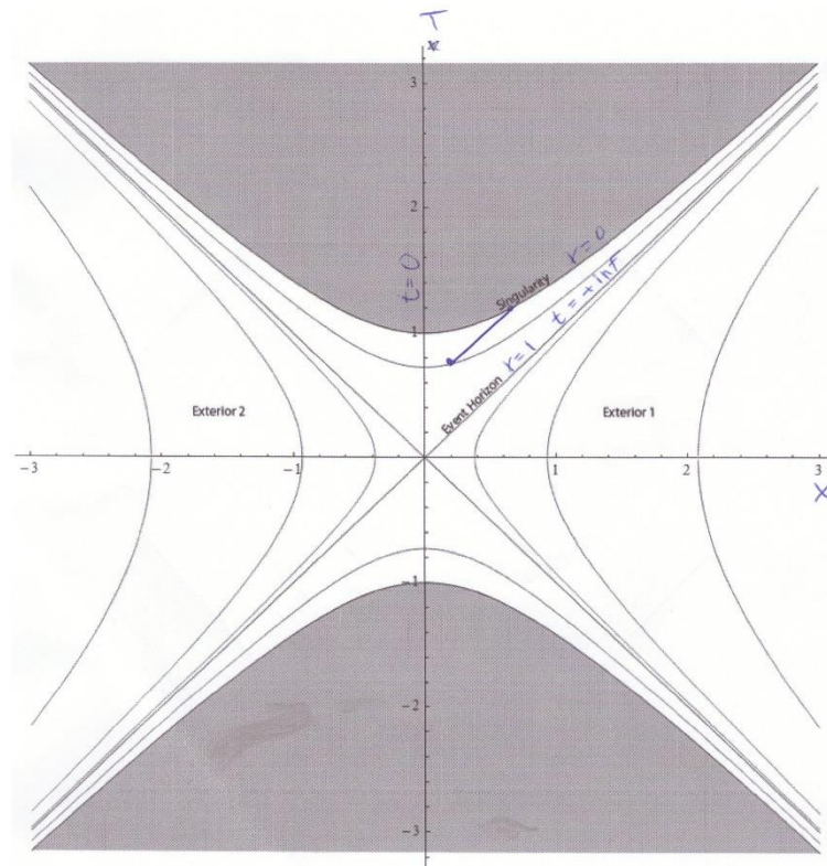
Figure 4. World-line in a Kruskal-chart of an outgoing photon that is believed to be doomed to end up at r=0 no matter where beyond the Schwarzschild horizon it is starting its journey
