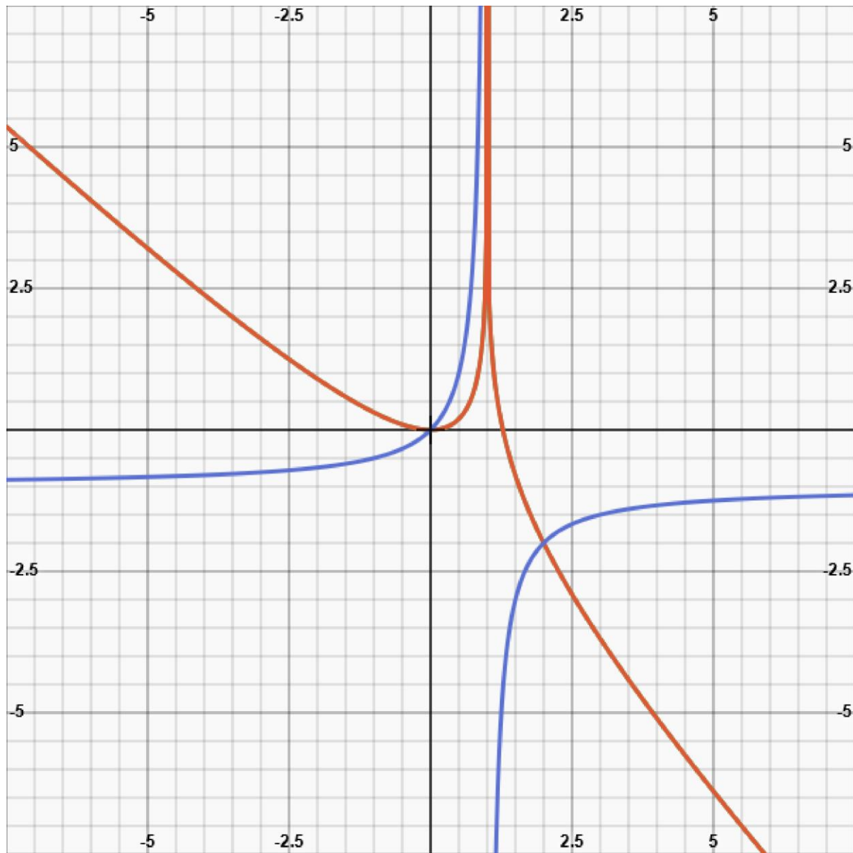
Figure 3a. The world-line (in a t,r -diagram) of a photon that falls into a black hole. The Schwarzschild horizon is at r=1 . The area to the left of the vertical axis has no significance, since a negative r does not exist.
