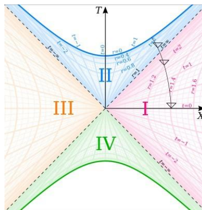
Figure 2c. A Kruskal-chart taken from Wikipedia. The numbering I, II, III, IV does not match with the numbering of quadrants used in this article.
