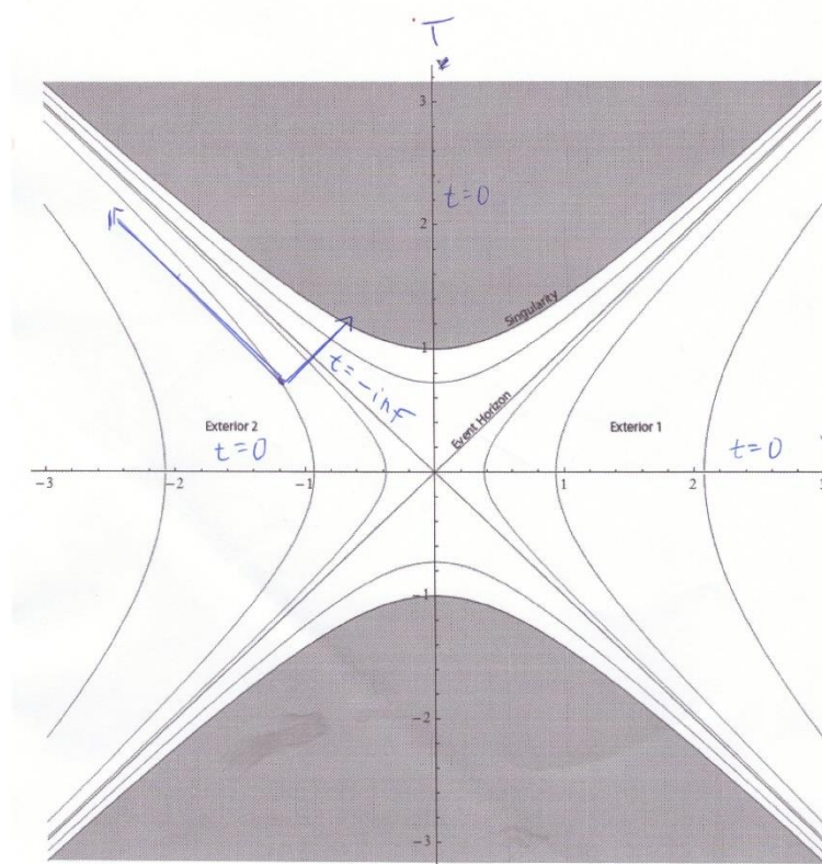
Figure 5. A wrong way of using Kruskal-charts for the world-line of an INGOING photon. The photon appears to go backward in time outside of the Schwarzschild radius, no matter which of the two paths are chosen. outside.
