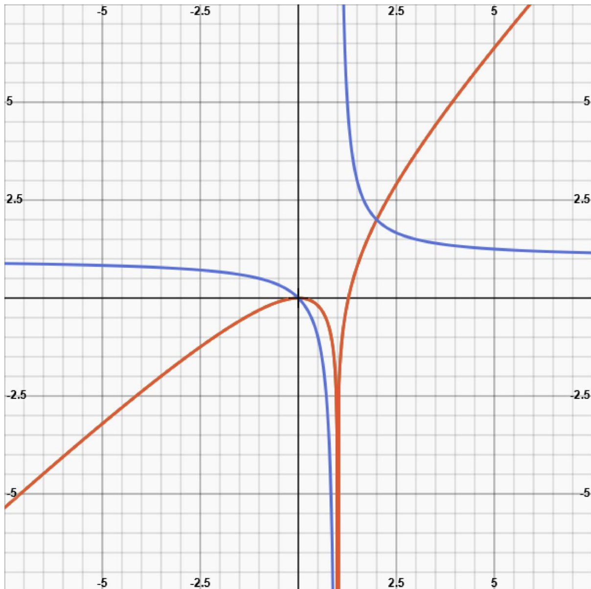
Figure 3c. World-line (in a t,r -diagram) of a photon that leaves a black hole. The area to the left of the vertical axis has no significance, since a negative r does not exist.
