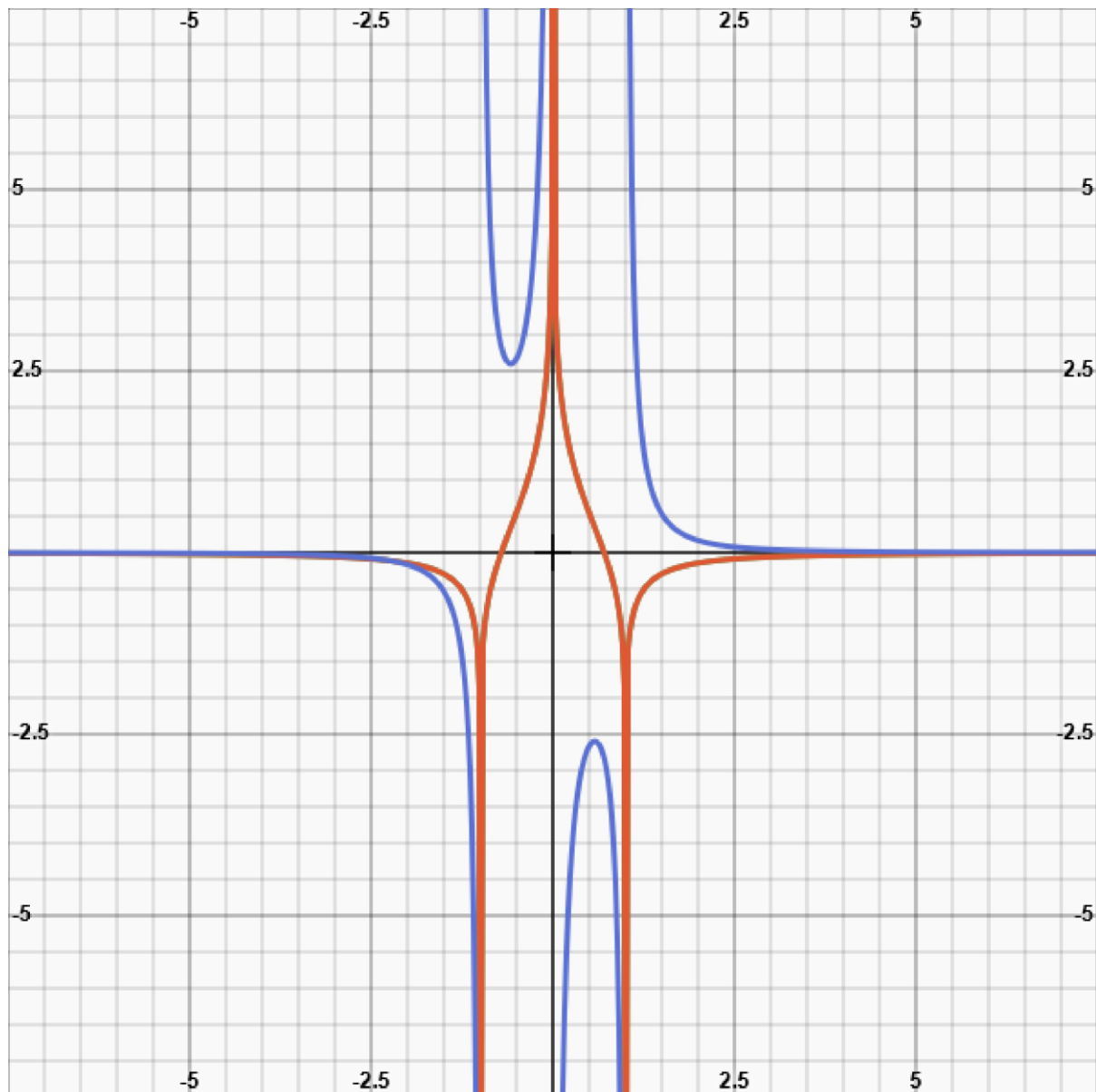
Figure 1b. World-Line Of Galaxy (In A T,R-Diagram) In Red Colour That Is Approaching The Milky Way Due To A hypothetical contraction of space. The area to the left of the vertical axis has no significance, since a negative r does not exist.
