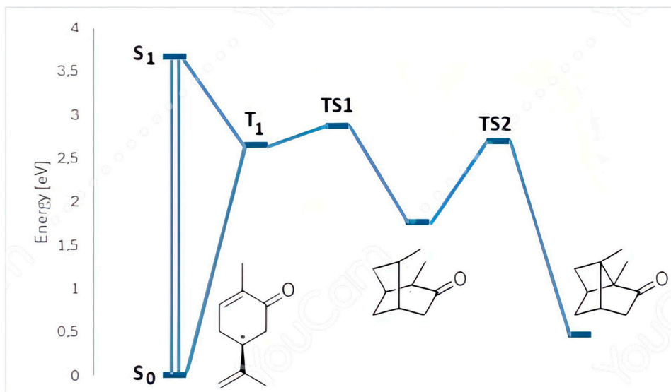
Figure 4. DFT calculations on carvone photoisomerization.
