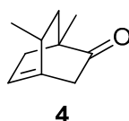
Figure 3. Hypothetical isomerization product resulting from 6.
