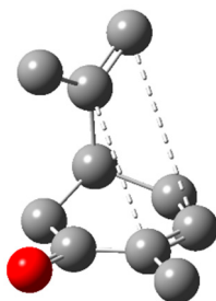
Figure 2. Possible interaction between the olefinic carbon atoms of carvone.
