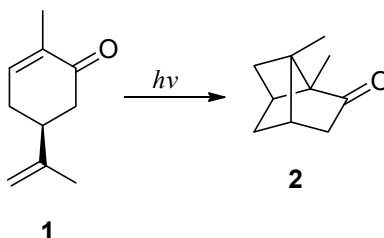
Scheme 1. Photochemical isomerization of carvone.
