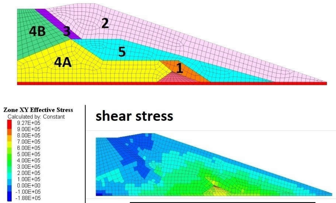
Figure 8. FLAC2D computation of shear stress in 2025 East Dam cross section A1 shows the shear stress in the vicinity of the starter dam and its foundation exceeds 100kPa. Dam zone labels 1:compacted cycloned sand, 2:uncompacted cycloned sand, 3:tailings sand + cyclone overflow, 4:tailings slimes, 5:water saturated cycloned sand.
