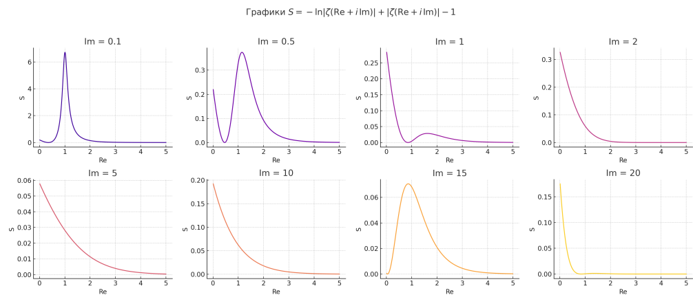
Figure 5. Graphs of S = |\zeta(Re + i \cdot Im)| - \log |\zeta(Re + i \cdot Im)| - 1 at various Im values
