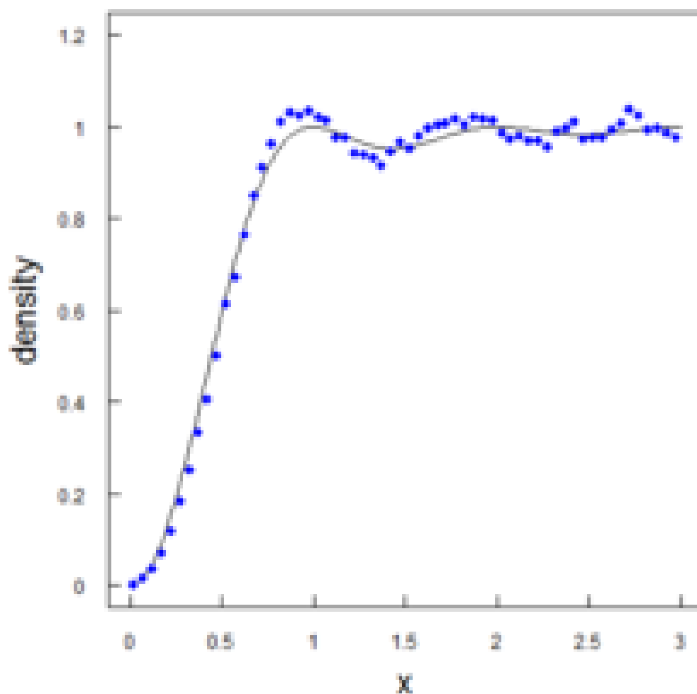
Figure 3. Connection between zeta zeros and quantum statistics.
