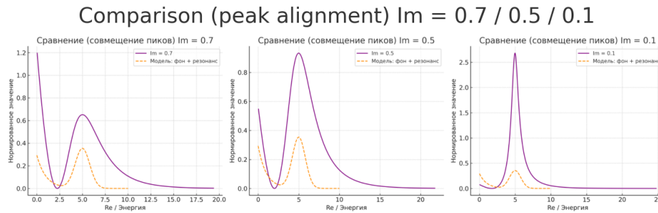
Figure 6. Graphs of S = |\zeta(\text{Re} + i \cdot \text{Im})| - \log |\zeta(\text{Re} + i \cdot \text{Im})| - 1 at various \text{Im} values.
