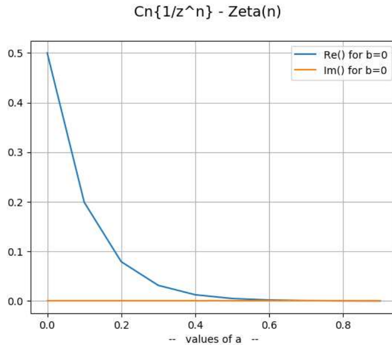
Figure 4a. Where a=\text{Re}(z) and b=\text{Im}(z) .
