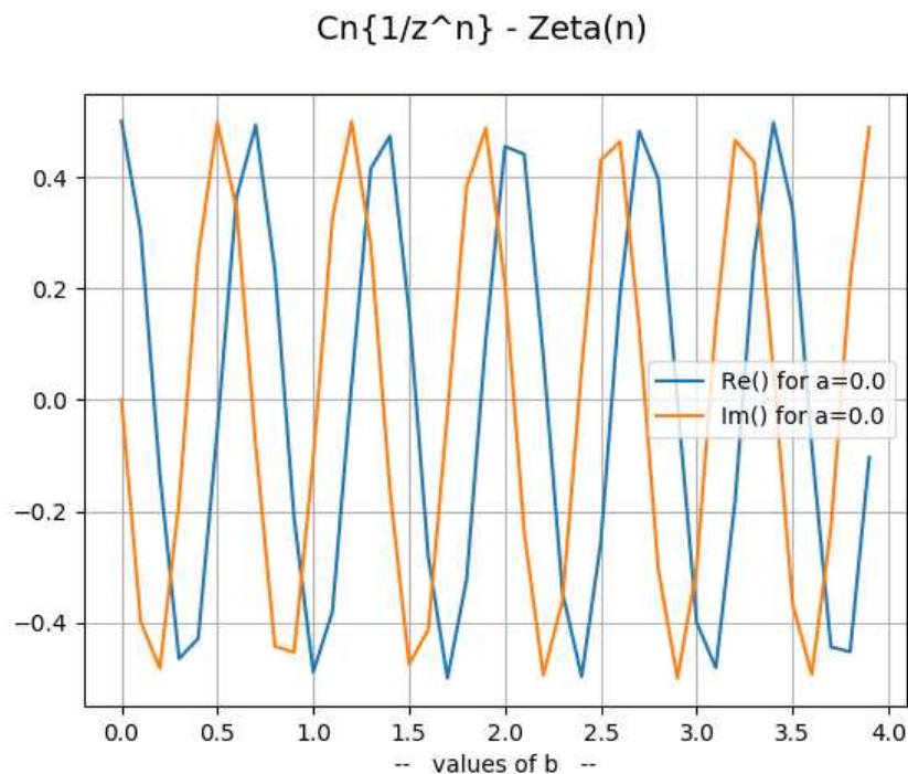
Figure 4b. Where a=\text{Re}(z) and b=\text{Im}(z) .
