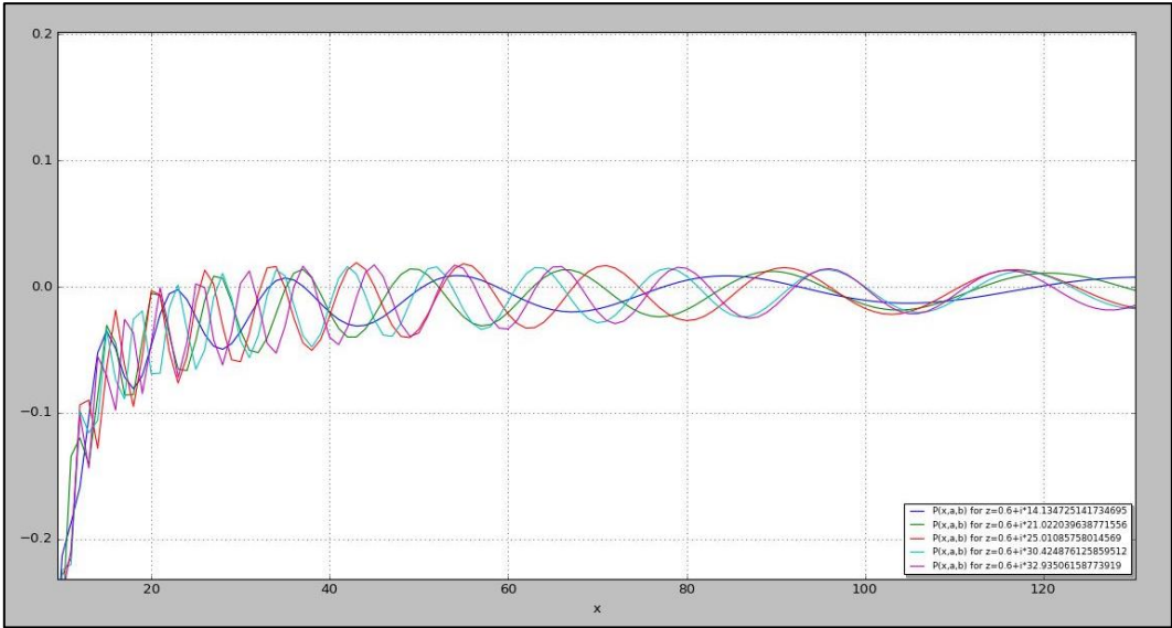
Figure 23. C_2(n, a, b) for a=0.6 and variable b .
