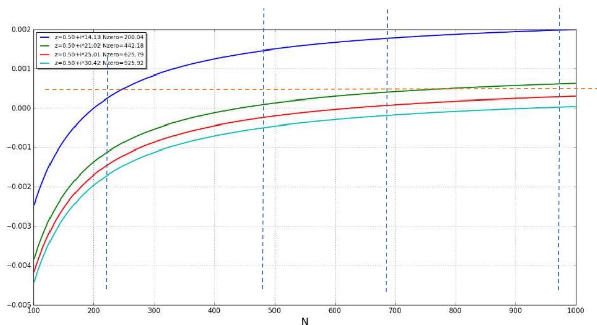
Figure 24. C_2(n, 1/2, b) such that \zeta(1/2+b*i)=0 .
