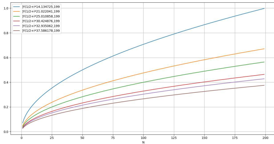
Linear representation for |Y(z, n)|^2 for (z) a nontrivial zero of Riemann Zeta. [Figure. 16]
