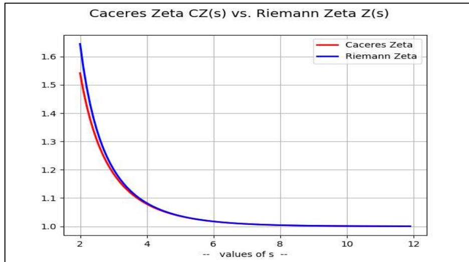
Figure 2. Caceres' approximation for the Riemann Zeta function in R.
