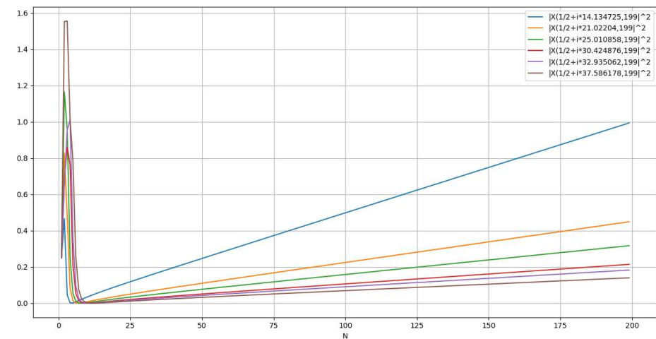
Linear representation for |X(z,n)|^2 for (z) a nontrivial zero of Riemann Zeta. [Figure. 13]
