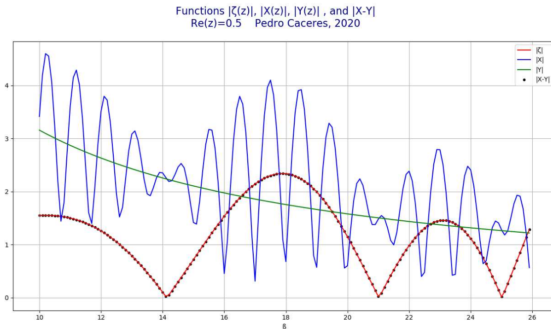
Figure 25. for \zeta(z) = X(z) - Y(z) = 0 \rightarrow |X(z)| = |Y(z)| for \text{Re}(z) = 1/2 .
