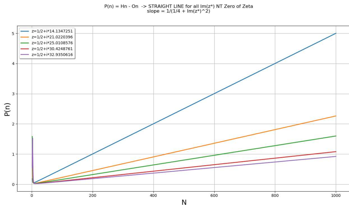
Figure 26. Straight Lines P(n) .
