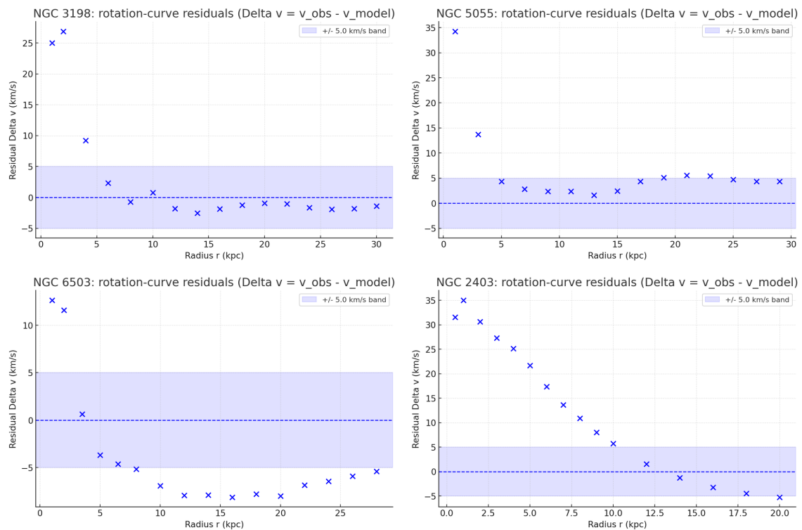
Figure A9. Residuals \Delta v = v_{\text{obs}} - v_{\text{model}} for the four representative galaxies under the shared-parameter configuration (cf. Table 3). Shaded bands mark \pm 5 \text{ km s}^{-1} .
