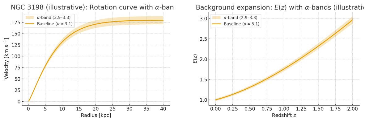
Figure A2. Allowed \alpha band from (left) rotation-curve outer tails and (right) E(z) slope. The overlap yields 3.0 \lesssim \alpha \lesssim 3.2 ; shading indicates stability range.
