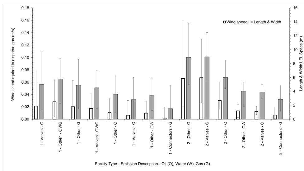
Figure 2. Blank bars show the calculated wind speeds required to disperse gas from fugitive emission types reported in the BOEM 2017 Gulfwide Emission Inventory Study. Grey bars show the length and width of spaces where methane concentrations from? can build up to LEL during zero wind condition.
