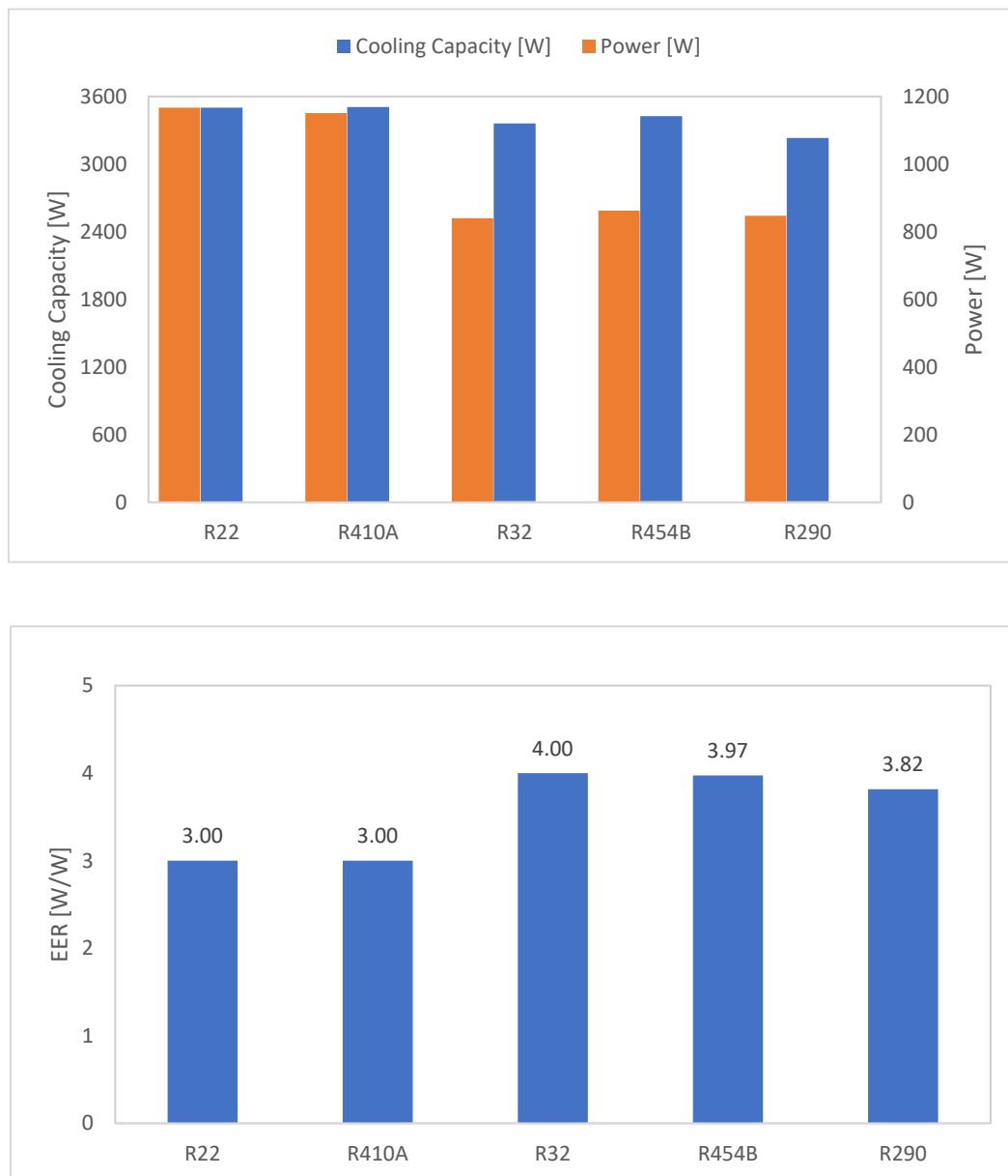
Figure 5. Energy efficiency performance for the optimized R32, R454B, and R290 mini-split units (full capacity cooling).
