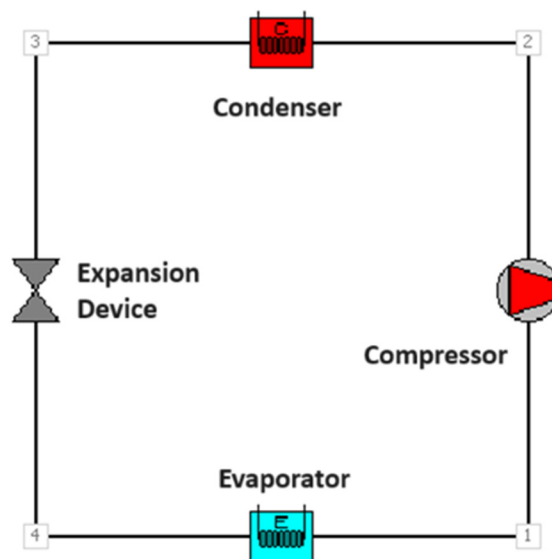
Figure 1. Air conditioner system diagram in VapCyc.
