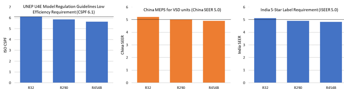
Figure 6. Seasonal energy performances of three prototype AC units.
