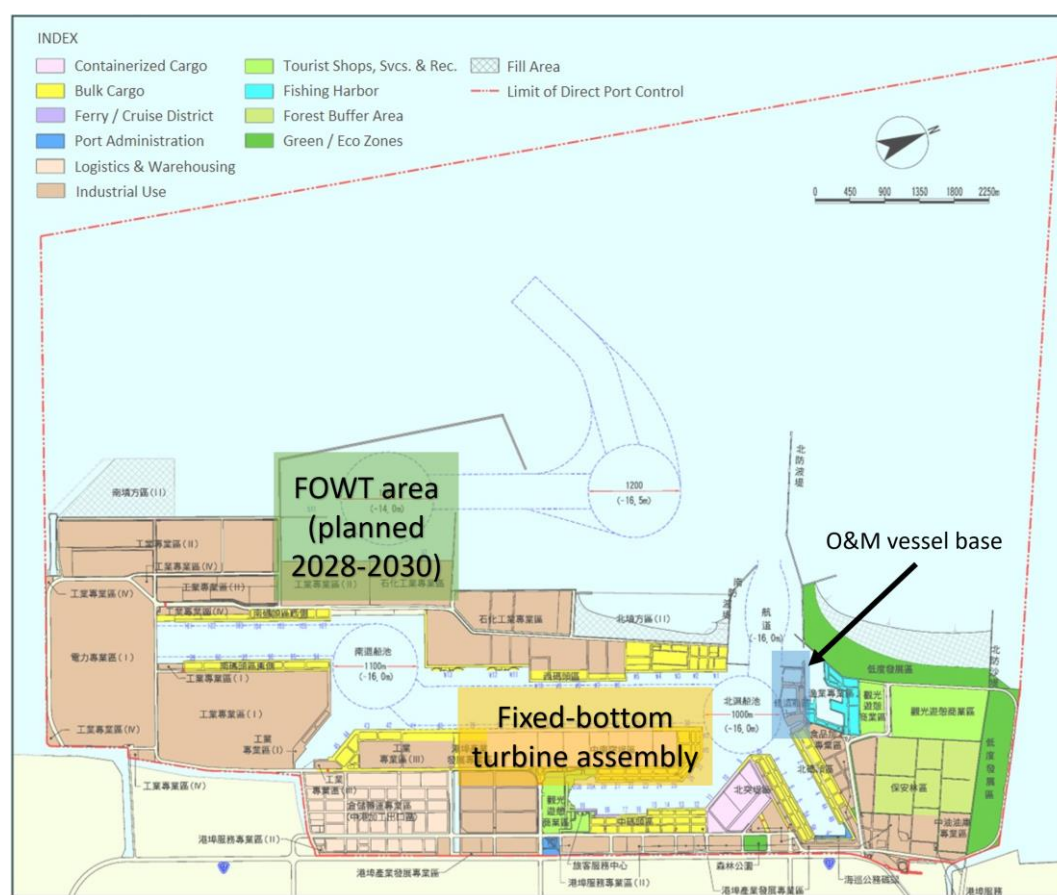
Figure 1.1. Future arrangements for accommodating the integration and assembly of floating wind turbines, using Taichung port as an example. Reworked based on a picture from [13].
