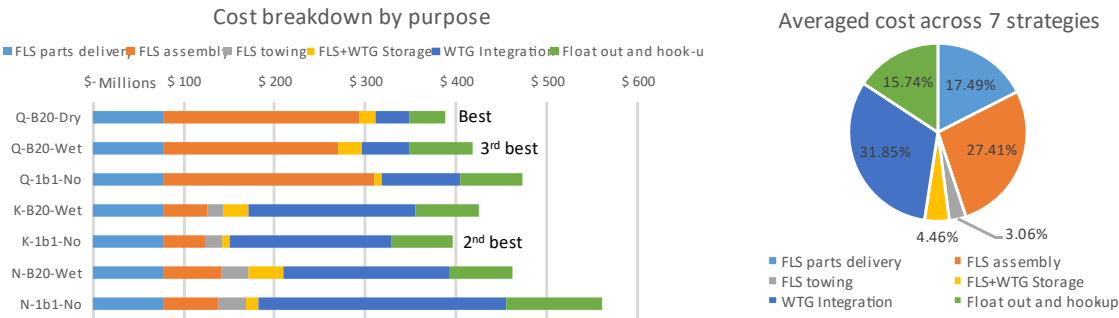
Figure 5.3. Assembly cost breakdown charts, with Q-B20-Dry being the best overall.
