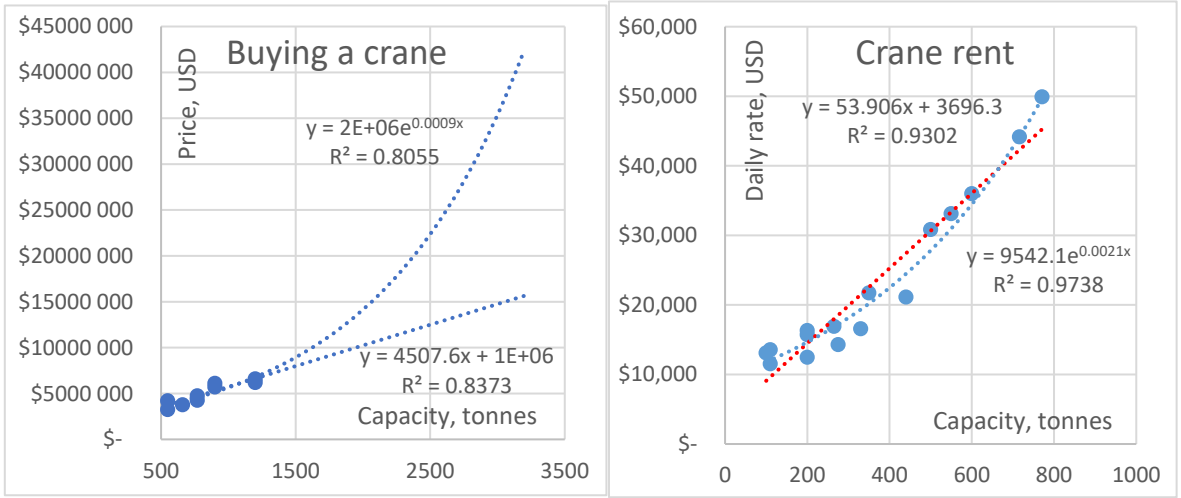
Figure 4.1. Crane price extrapolation.
