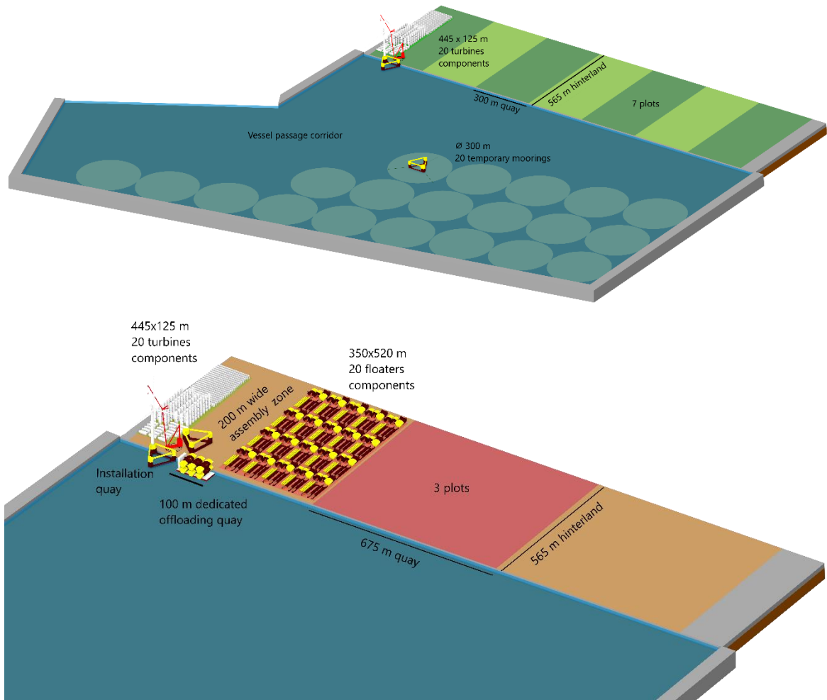
Figure 5.2. Possible wet (top) and dry (bottom) floater storage arrangements in Taichung port.
