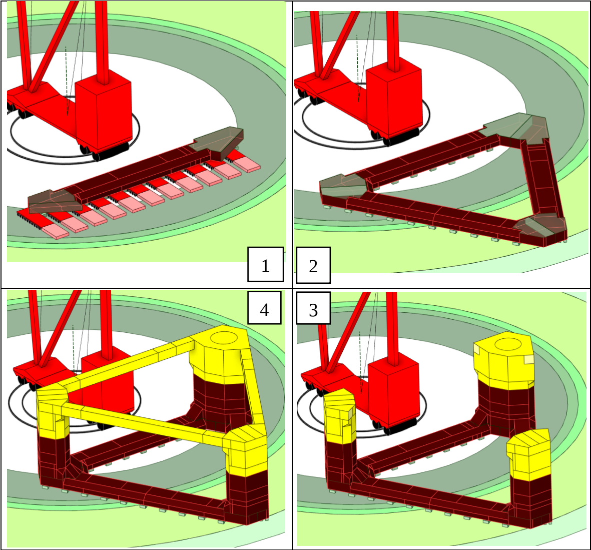
Figure 3.2. Floater quayside block assembly, steps 1 to 4.
