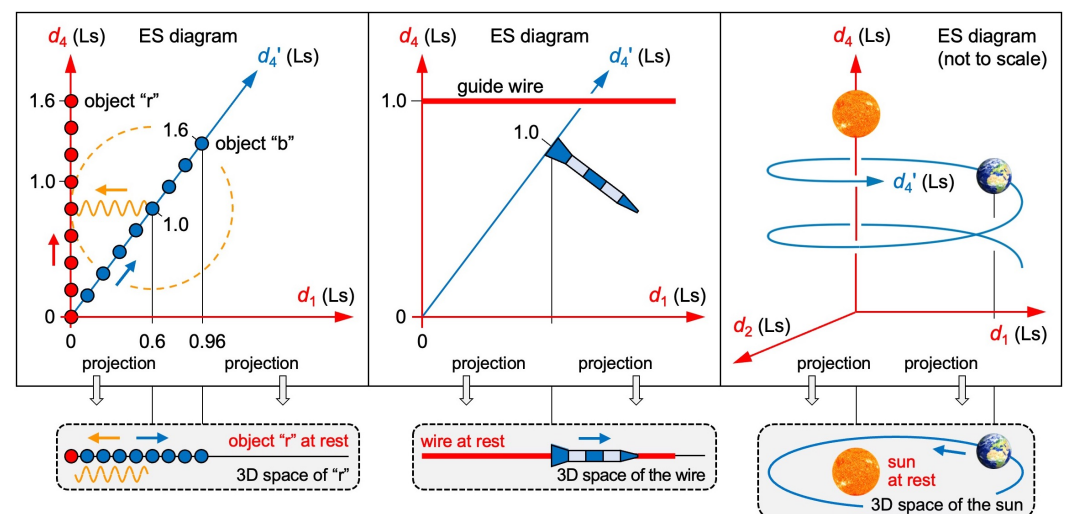
Fig. 5 Three instructive problems. Left: In ES, an energy taking a detour (blue/orange arrow) cannot collide with an energy moving straight (red arrow). In 3D space, it can. The orange circle shows where a radio signal emitted by "b" is after 0.6 s. Center: In ES, the wire escapes from the rocket. In 3D space, it does not. Right: In ES, the sun escapes from Earth's orbit. In 3D space, it does not.
