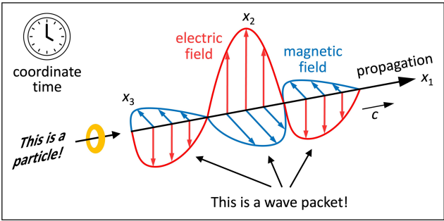
Fig. 8 Illustration of a single wavematter. In an observer's view, it reduces to a wave packet or else a particle. As a wave packet (shown here), it propagates and it oscillates as a function of his coordinate time. In the wavematter's view (view through the yellow pinhole), it is a particle at rest.
