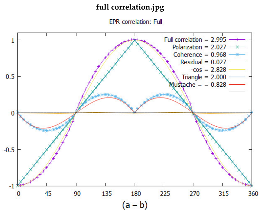
Figure 7. Plotting intensity versus the angle difference ( \theta_a - \theta_b ). The results of the simulation are given by the blue points. The CHSH values are listed. The full correlation is the sum of that from polarization, the triangle, and coherence, the mustache. Note the hardly discernible residual quaternion correlation along the horizontal axis.
