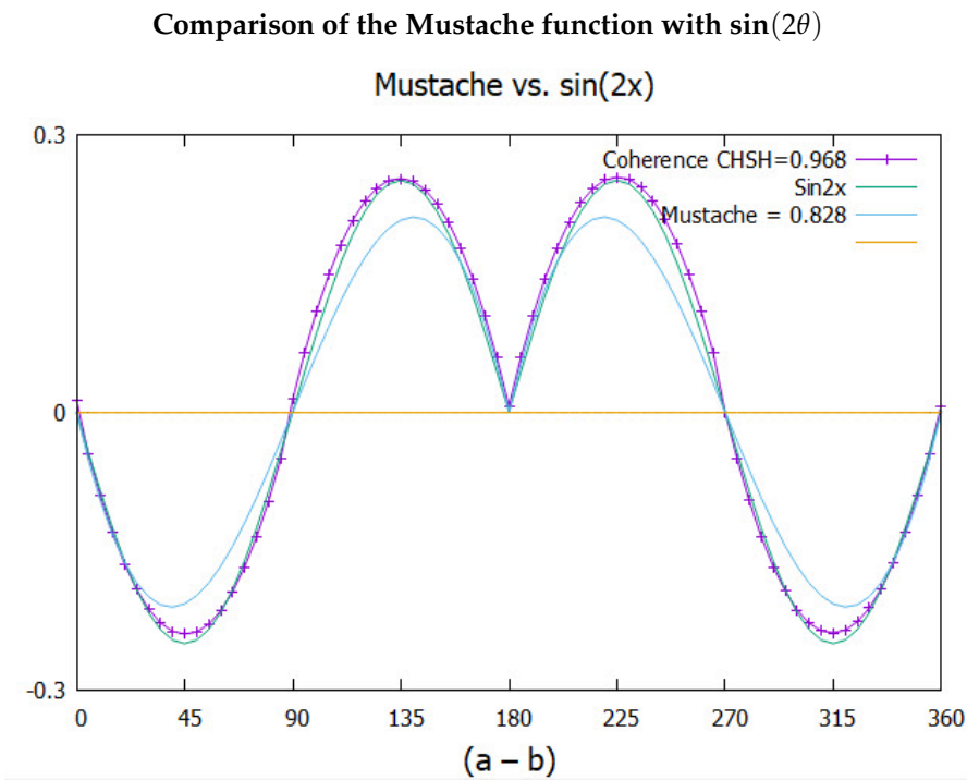
Figure 9. The E_q function given in Equation (34) compared to the simulation. Also shown is the correlation from quantum theory.
