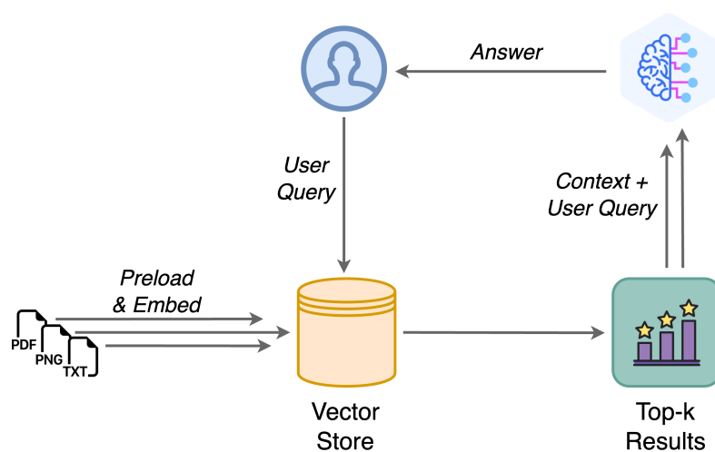
Figure 1. LangChain pipeline architecture showcasing the retrieval-augmented generation process. Documents in various formats (e.g., PDF, text, images) are preloaded and embedded into a vector store. When a user submits a query, the system retrieves the top-k most relevant documents based on vector similarity. These documents are combined with the query to provide contextual information to the language model (LLM), which then generates an accurate and contextually enriched answer. This architecture enhances the model's ability to produce factually grounded responses by incorporating relevant knowledge from the vector store.
