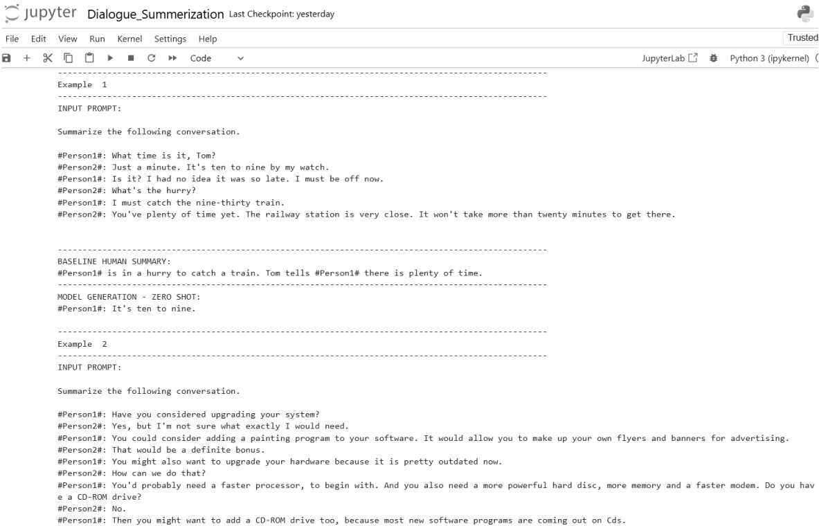
Figure 23. Zero-shot inference input and output (Part 3).
