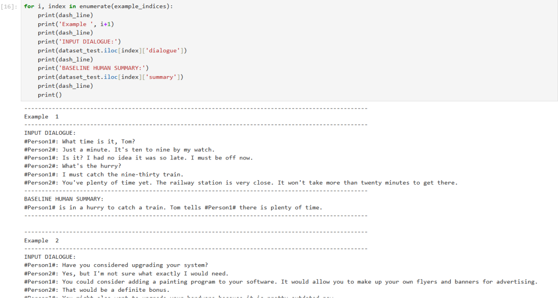
Figure 4. Dialogue summarization without prompt engineering (Part 1).
