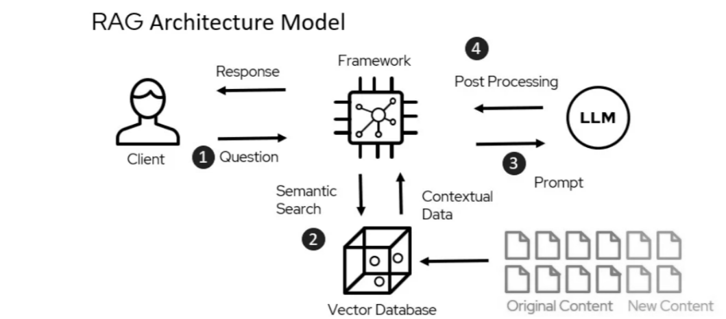
Figure 3. RAG architecture model illustrating the flow of information retrieval and response generation for educational applications.
