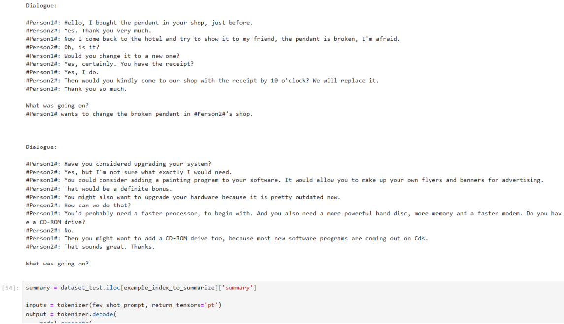
Figure 34. One-shot inference input and output (Part 1).
