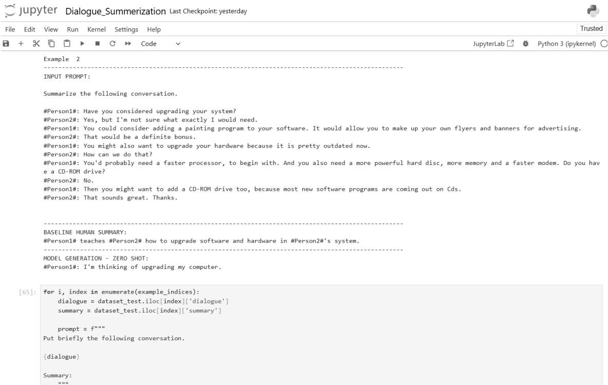
Figure 22. Zero-shot inference input and output (Part 2).
