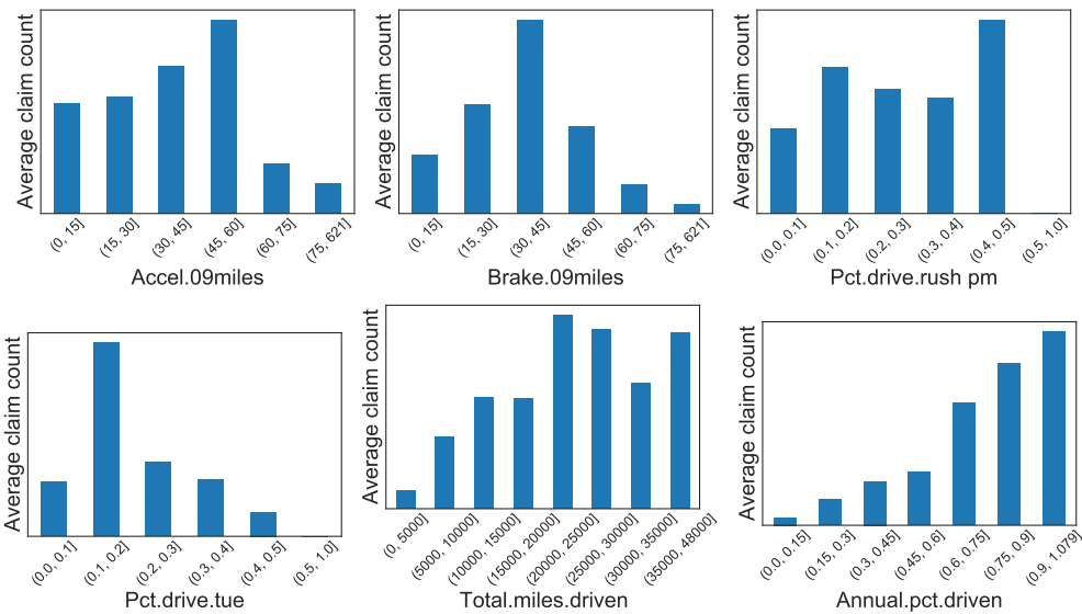
Figure A1. Synthetic data: Distribution of average number of claims for six telematics-related features.
