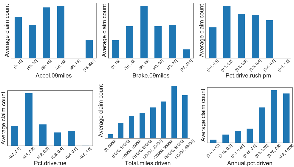
Figure A2. Real data: Distribution of average number of claims for six telematics-related features.
