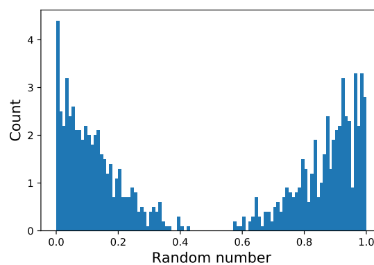
Figure 4. 1000 random numbers drawn from the U -shape distribution
