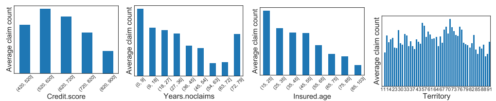
Figure A3. Synthetic data: Distribution of average number of claims for four traditional features.
