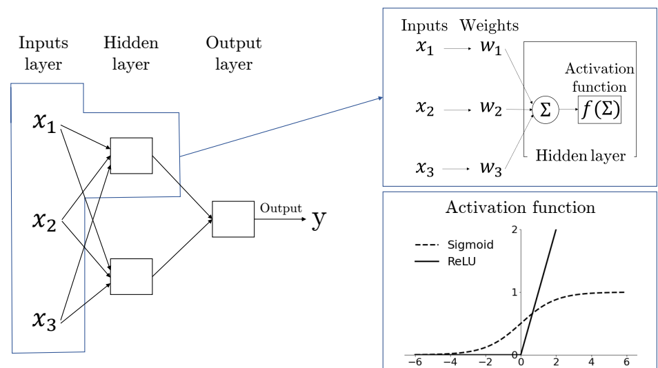
Figure 1. Architecture of a feedforward neural network.
