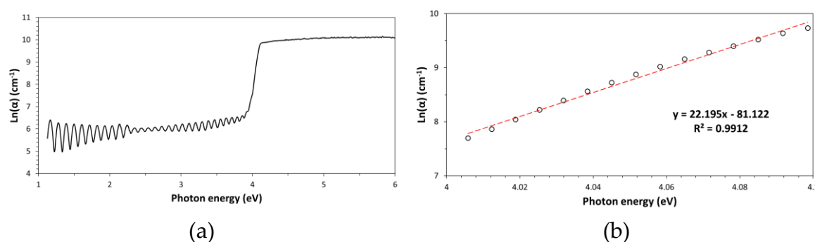
Figure 3. – PET thin film Urbach plot (a) and best fitting of the linear section of the curve (b).
