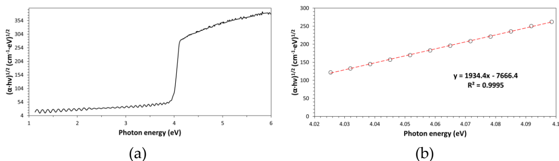
Figure 6. – PET thin film Tauc plot (a) and best fitting of the linear section of the curve (b).
