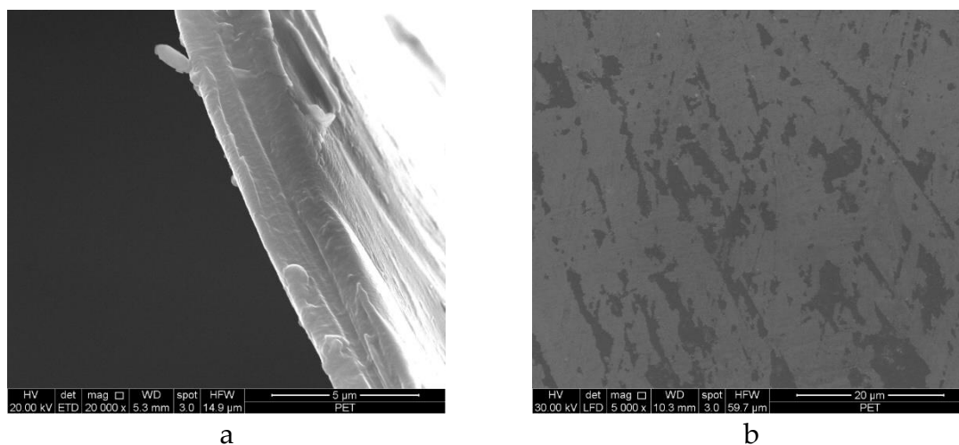
Figure 1. SEM micrographs of ultrathin PET film showing the cross-section (a) and the surface (b).
