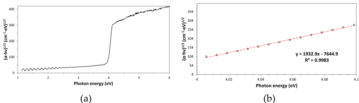
Figure 7. – Tauc plot (a) and bandgap energy estimation by linear regression analysis (b) for a stretched ultrathin PET film.
